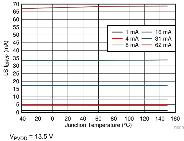
6-10. Low-Side Gate Driver Source Current
