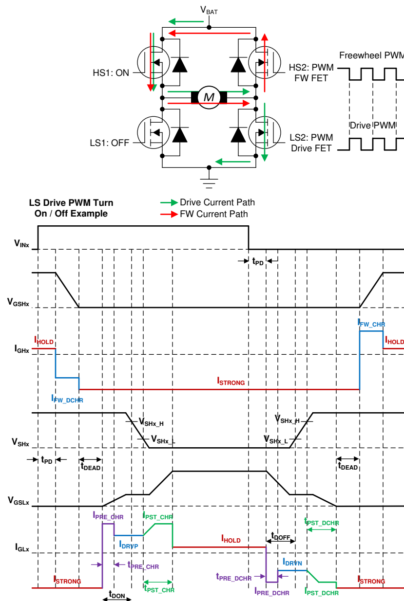
7-16. LS Drive PWM Turn On / Off Example
