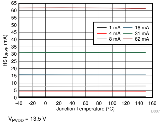
6-8. High-Side Gate Driver Source Current
