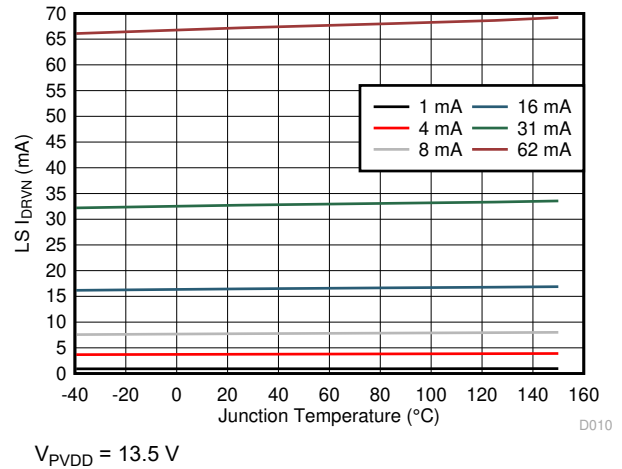
6-11. Low-Side Gate Driver Sink Current
