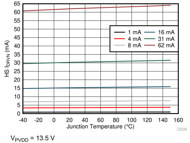
6-9. High-Side Gate Driver Sink Current
