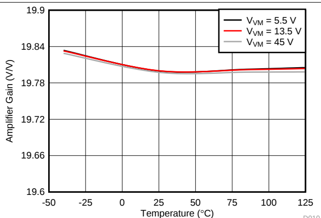
12. Amplifier Gain
