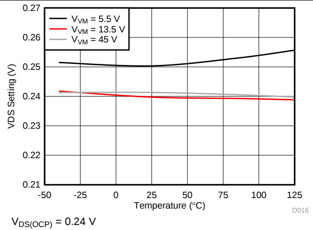
FIG 18. OCP Threshold Voltage
