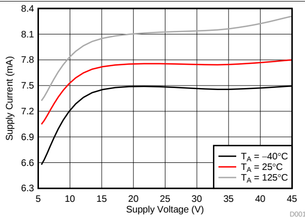
图 3. Supply Current vs Supply Voltage (VM)
