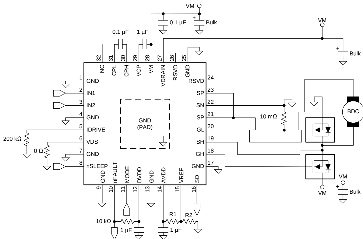
FIG 53. DRV8702D-Q1 Typical Application Schematic
