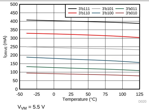
FIG 22. High-Side Sink Current
