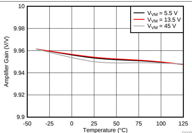
11. Amplifier Gain
