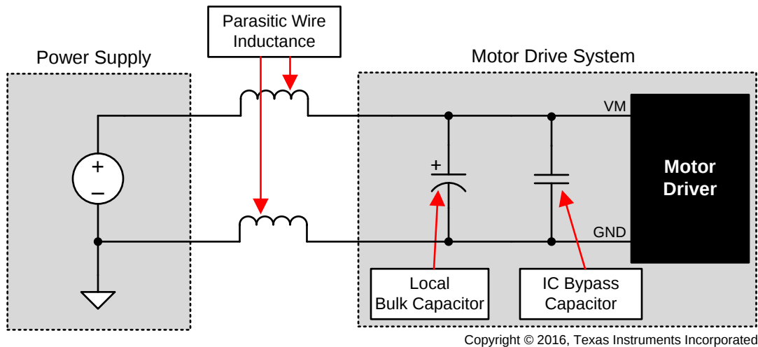
FIG 59. Example Setup of Motor Drive System With External Power Supply
