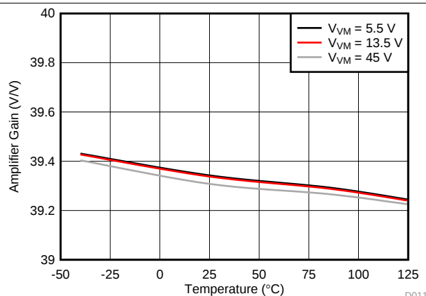
11. Amplifier Gain
