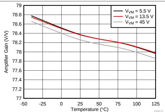
12. Amplifier Gain
