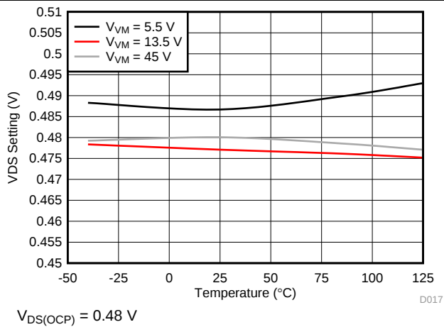
FIG 19. OCP Threshold Voltage
