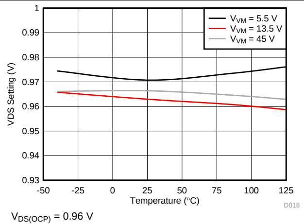
FIG 20. OCP Threshold Voltage
