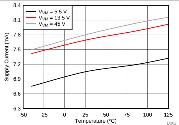
图 4. Supply Current vs Temperature
