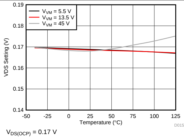
FIG 17. OCP Threshold Voltage
