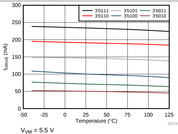
FIG 21. High-Side Source Current
