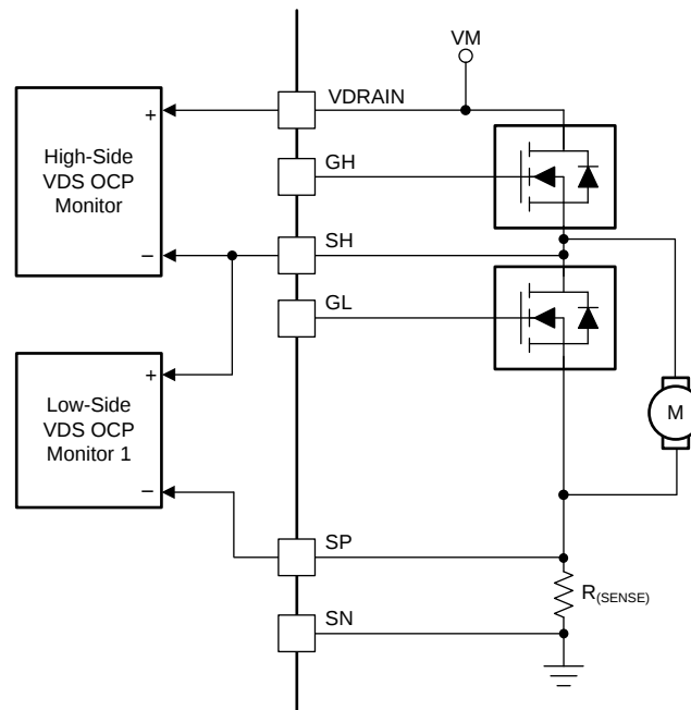
41. V_{DS(OC)} Block Diagram
