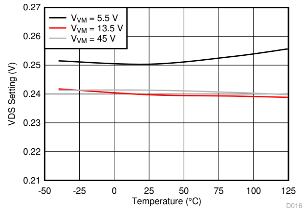
6-14. OCP Threshold Voltage
