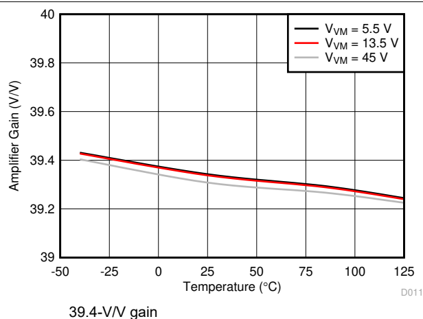
6-11. Amplifier Gain
