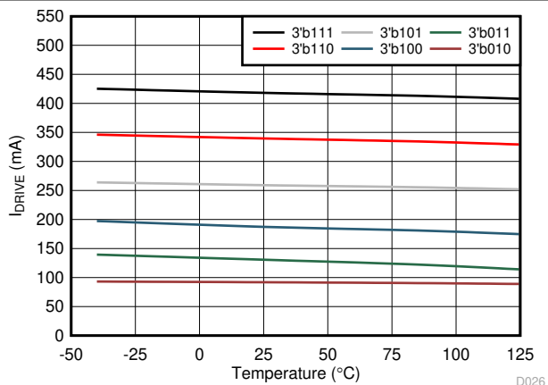
6-26. Low-Side Sink Current
