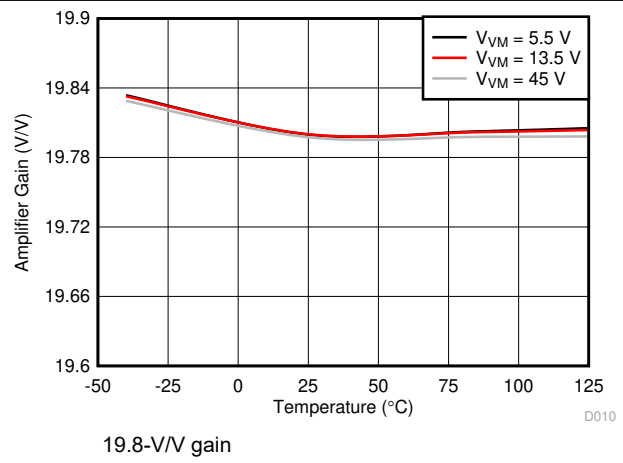
6-10. Amplifier Gain
