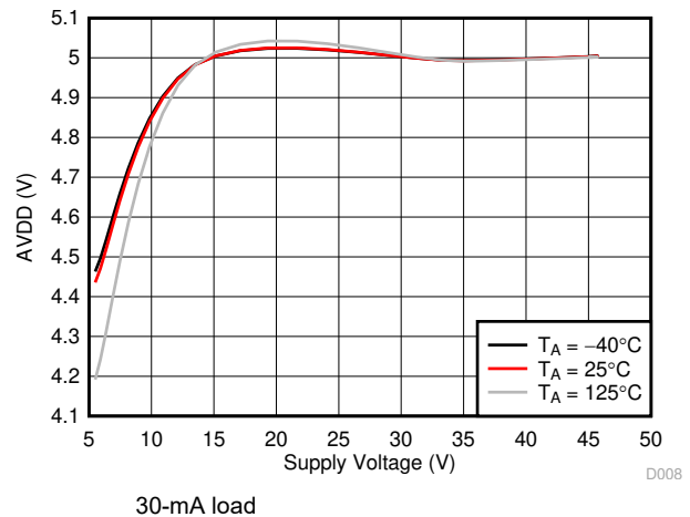
6-8. AVDD Regulator
