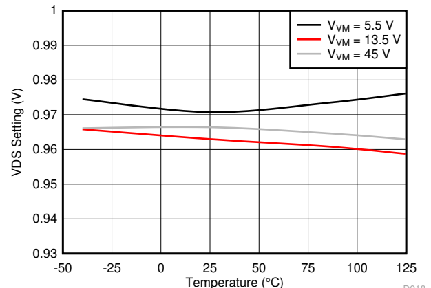
6-16. OCP Threshold Voltage
