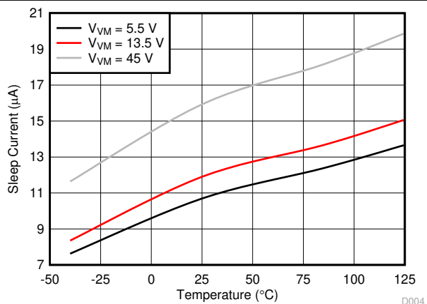
6-4. Sleep Current vs Temperature
