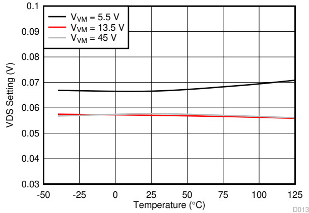
6-13. OCP Threshold Voltage
