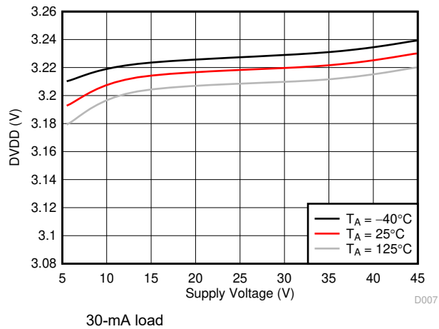
6-7. DVDD Regulator
