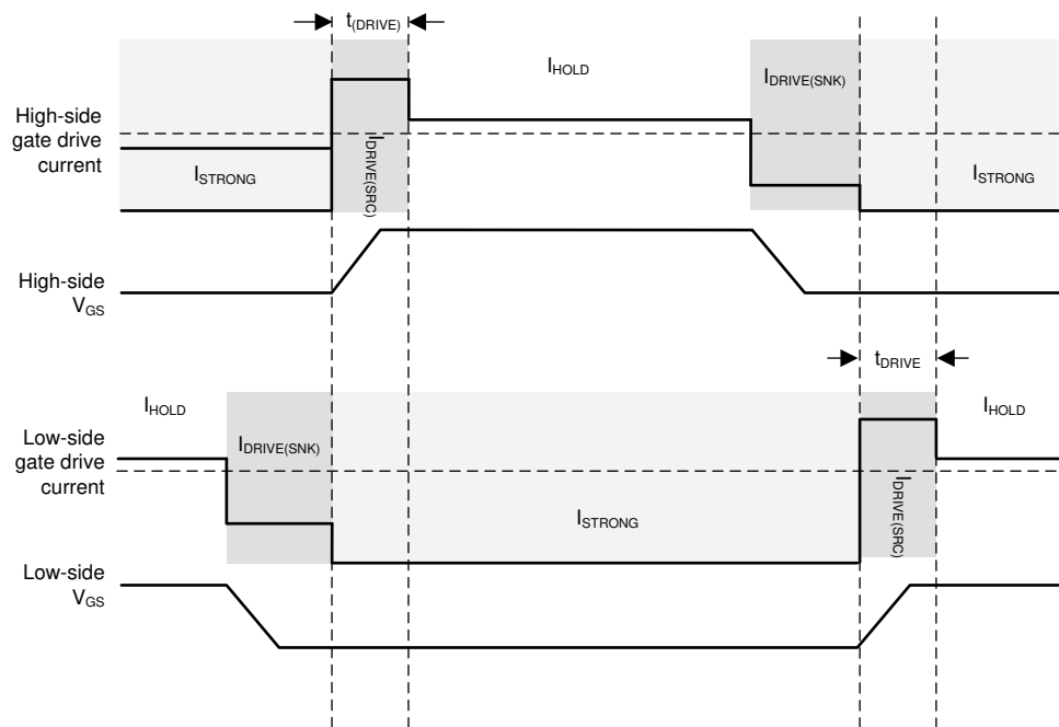
FIG 7-10. Gate Driver Output to Control External FETs
