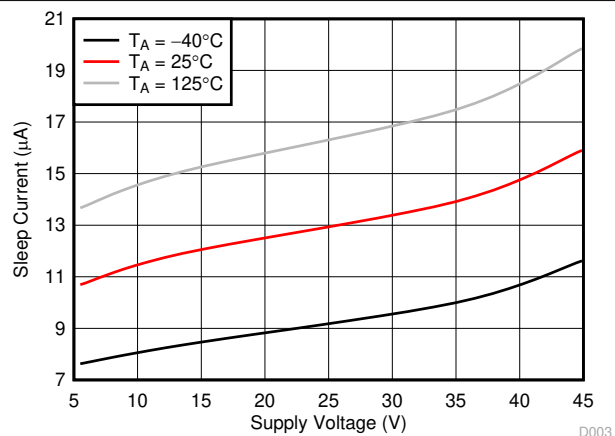
6-3. Sleep Current vs Supply Voltage (VM)
