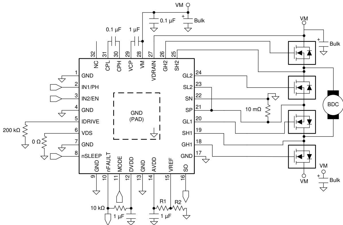
図 8-1. DRV8702-Q1 Typical Application Schematic
