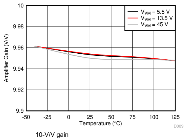
6-9. Amplifier Gain
