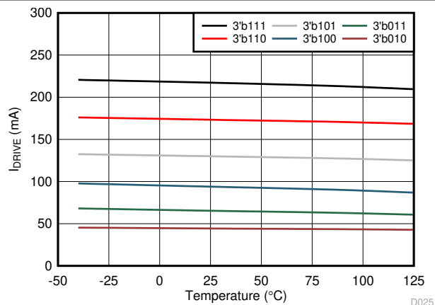
6-25. Low-Side Source Current
