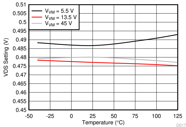
6-15. OCP Threshold Voltage
