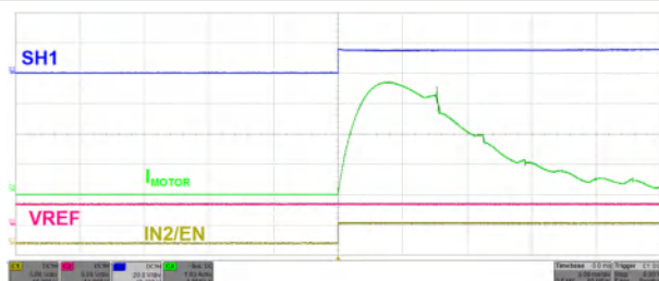
Figure 8-5. Current Profile on Motor Startup Without Regulation
