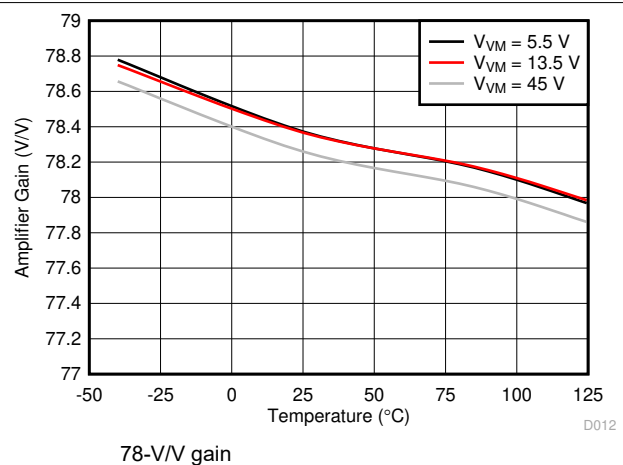
6-12. Amplifier Gain
