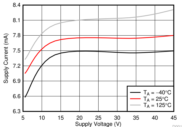
6-1. Supply Current vs Supply Voltage (VM)
