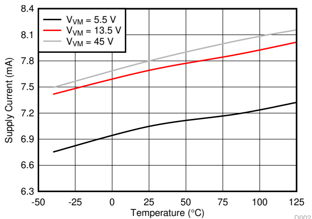
6-2. Supply Current vs Temperature
