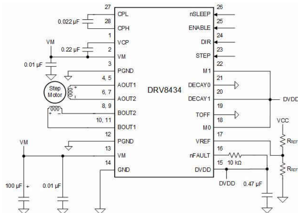
FIG 8-1. Typical Application Schematic (1/8 microstepping, smart tune Ripple Control Decay, HTSSOP package)
