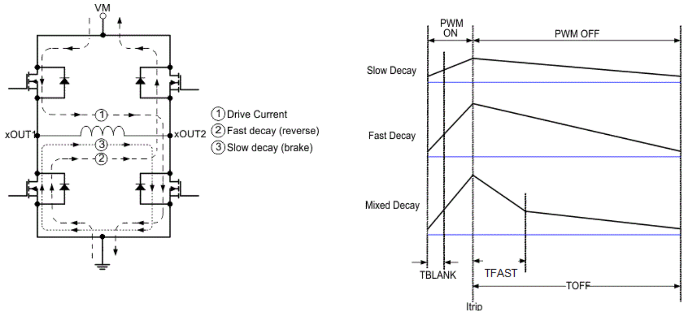
7-6. Decay Modes
