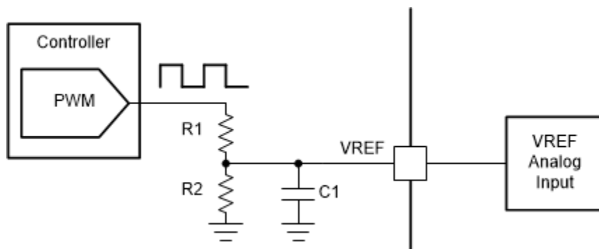
FIG 7-4. Controlling VREF With a PWM Resource
