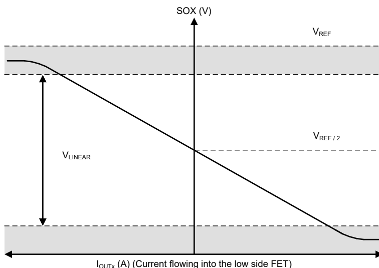
図 7-22. Bidirectional Current Sense Regions
