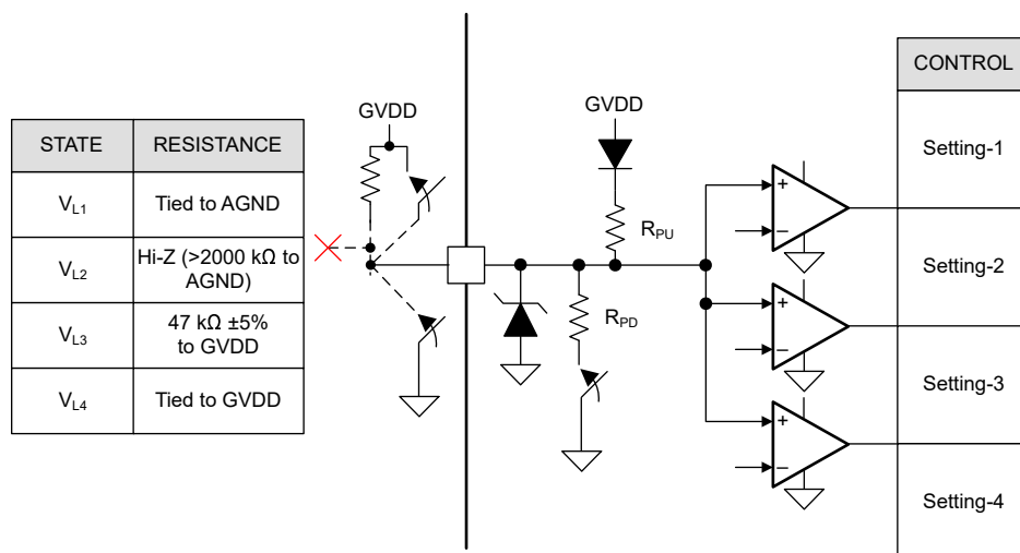
图 7-19. Four Level Input Pin Structure
