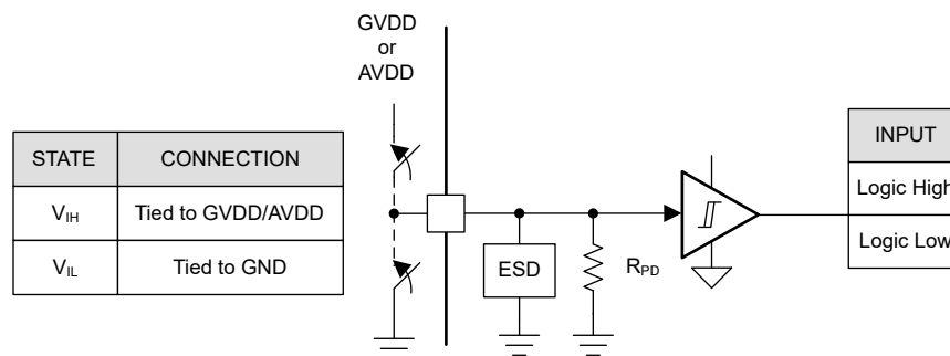
図 7-15. Logic-Level Input Pin Structure
