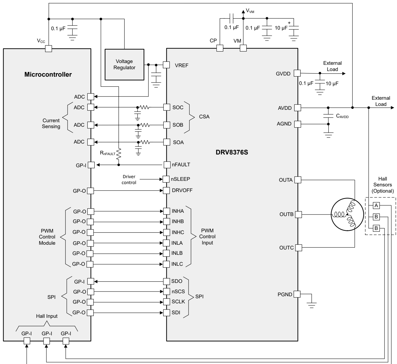
図 8-1. Primary Application Schematics
