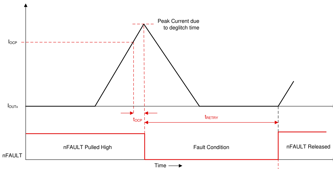
図 7-38. Overcurrent Protection - Automatic Retry Mode
