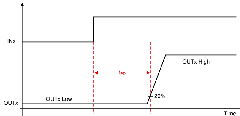
図 7-14. Propagation Delay Timing
