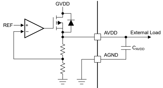
図 7-8. AVDD Linear Regulator Block Diagram
