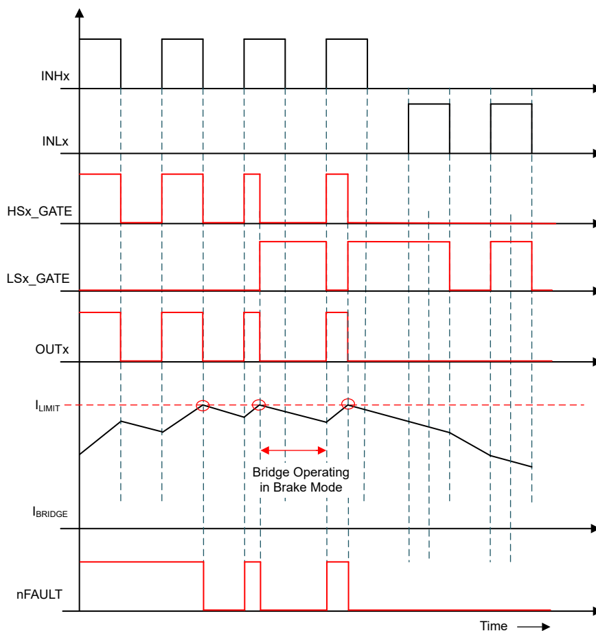
図 7-30. Cycle-by-Cycle Current-Limit Operation with Low Side Switching in Brake Mode
