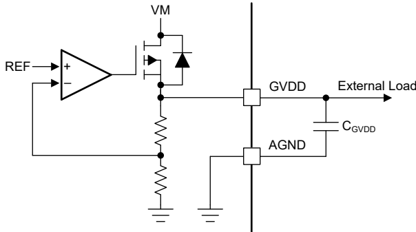
図 7-7. GVDD Linear Regulator Block Diagram
