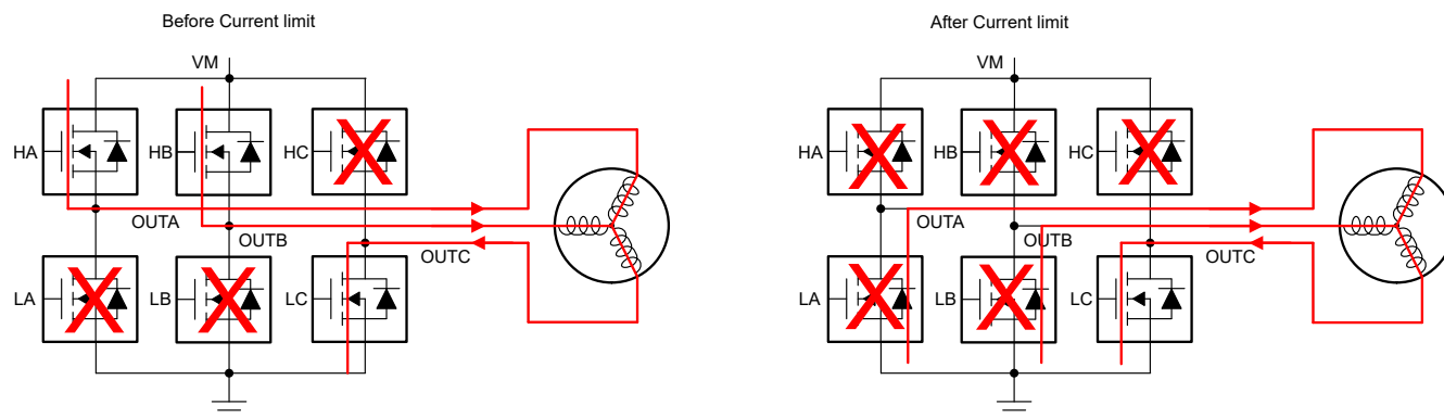
図 7-33. Coast State
