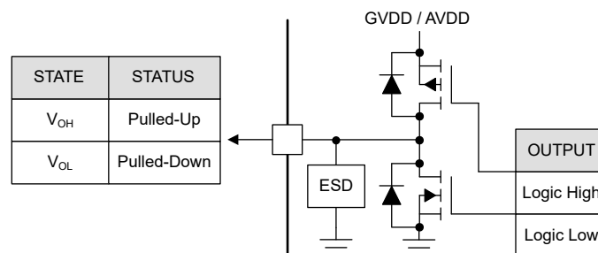
7-18. Push Pull
