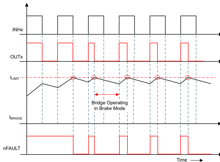
図 7-29. Cycle-by-Cycle Current-Limit Operation
