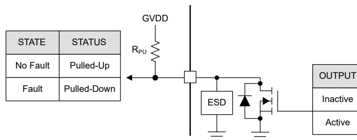
7-17. Open Drain
