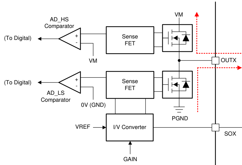
図 7-23. Active Demagnetization Operation
