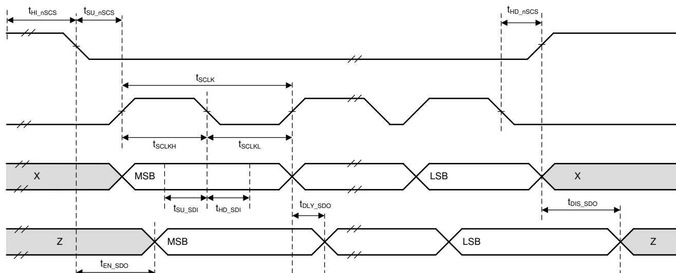
図 6-1. SPI Secondary Mode Timings
