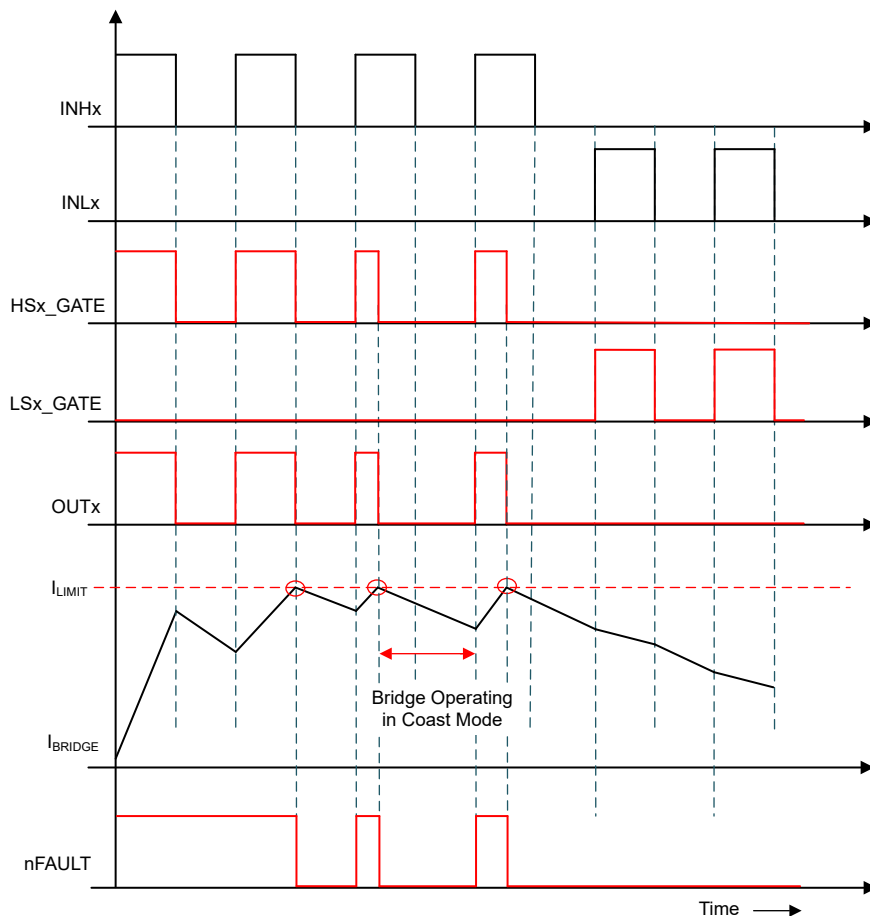
図 7-31. Cycle-by-Cycle Current-Limit Operation with Low Side Switching in Coast Mode
