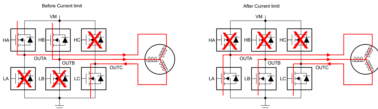
図 7-32. Brake State
