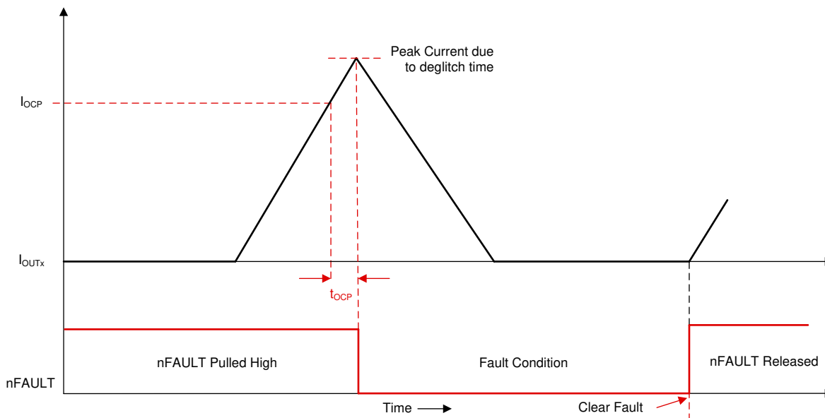
図 7-37. Overcurrent Protection - Latched Shutdown Mode
