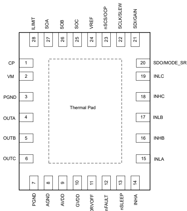
図 5-1. DRV8376 28-Pin VQFN With Exposed Thermal Pad Top View
