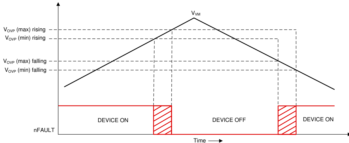
図 7-36. Over Voltage Protection
