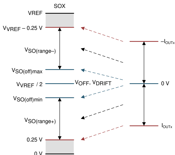
図 7-21. Bidirectional Current Sense Output
