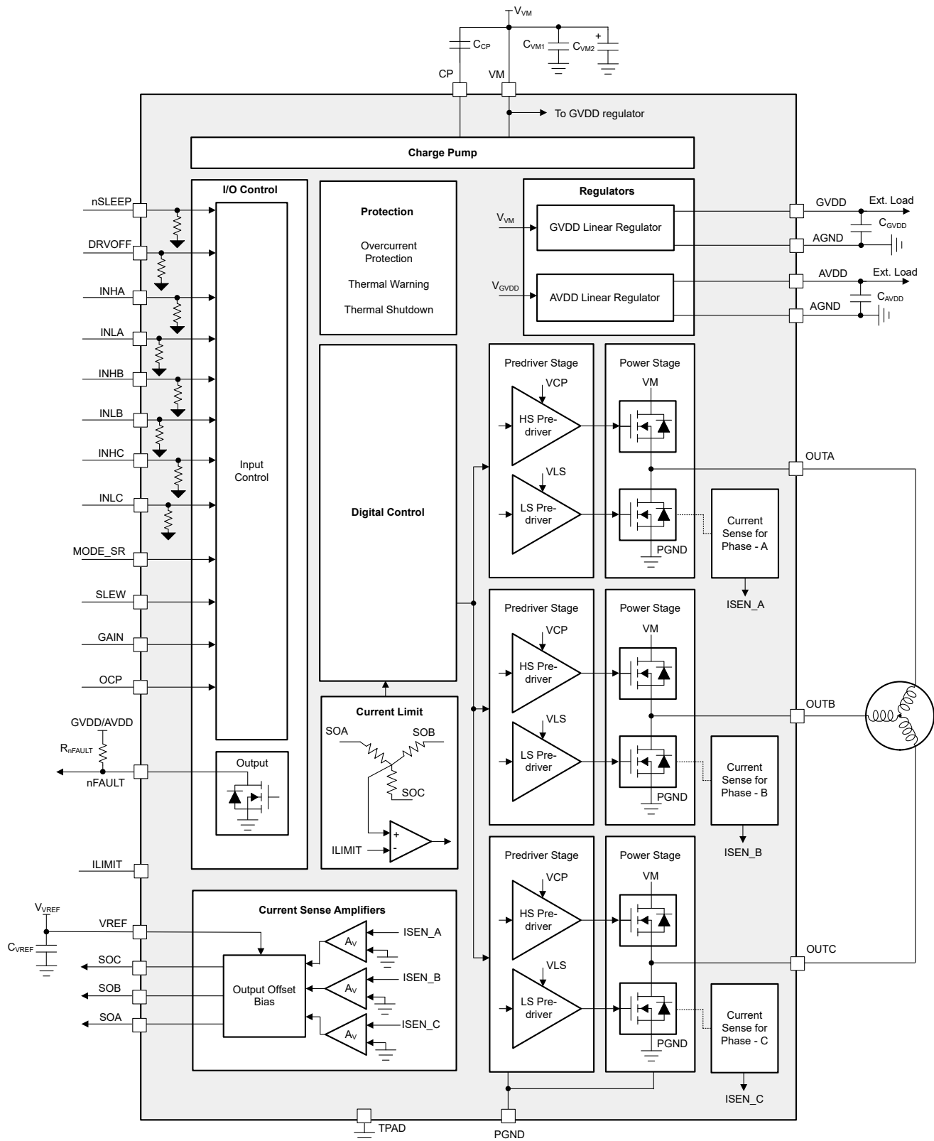
7-2. DRV8376H Block Diagram
