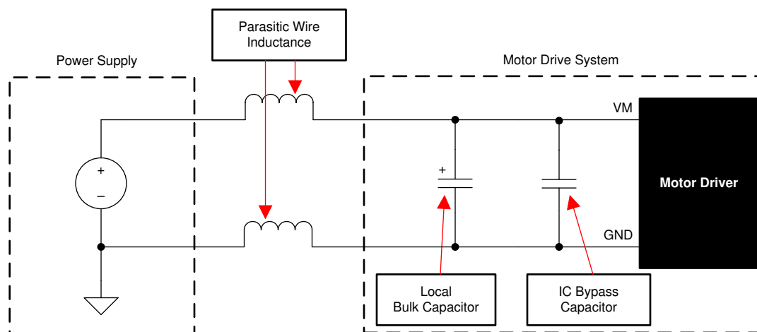
図 8-2. Example Setup of Motor Drive System With External Power Supply
