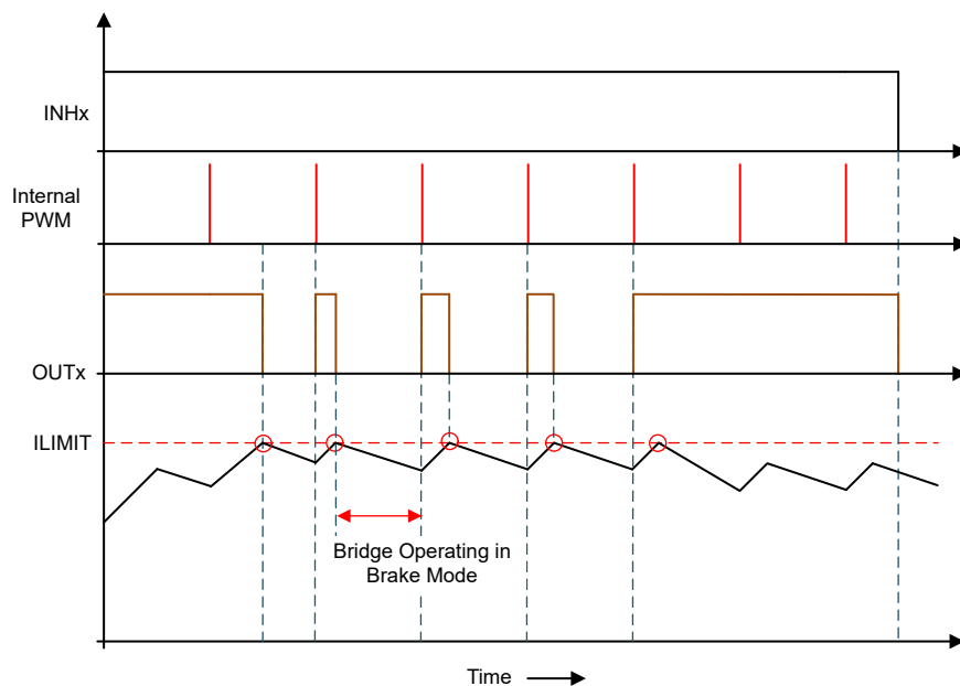
図 7-34. Cycle-by-Cycle Current-Limit Operation with 100% PWM Duty Cycle
