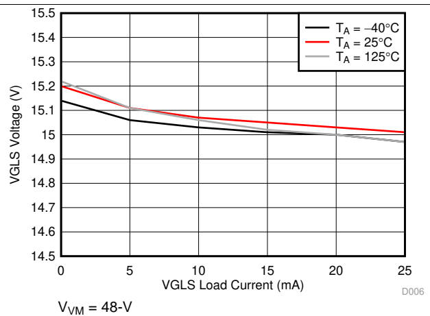
FIG 7. VGLS Voltage Over Load Current
