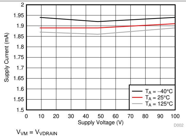
FIG 3. VDRAIN Supply Current Over Supply Voltage
