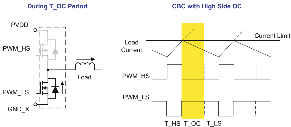
Figure 7-1. Cycle-by-Cycle Operation With High-Side OC
