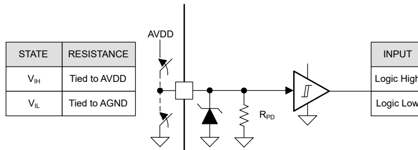
7-6. Logic-Level Input Pin Structure
