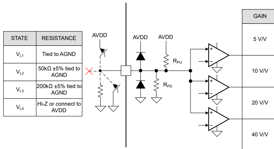
7-7. Four Level Input Pin Structure
