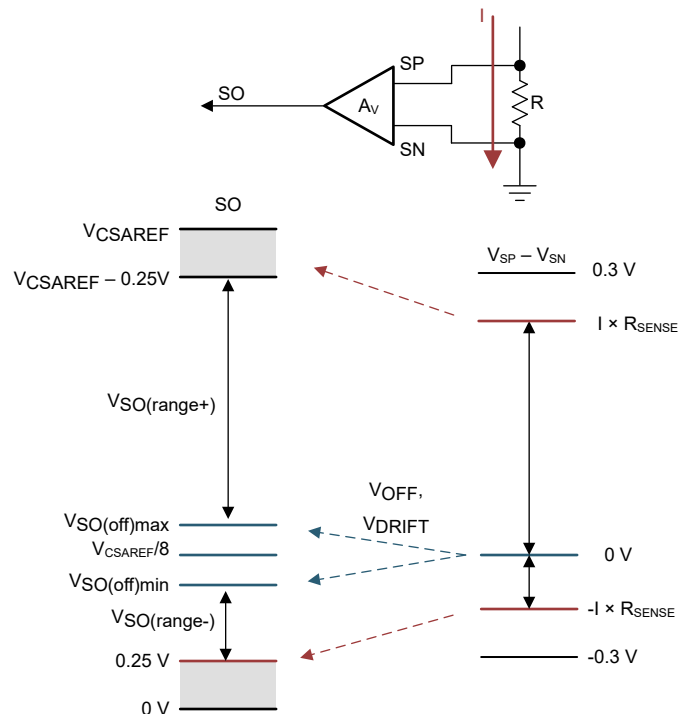
7-11. Current-Sense Regions
