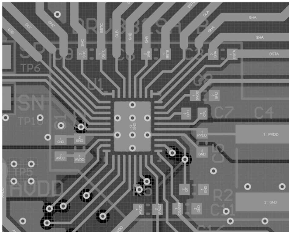
図 8-21. Layout of DRV8329 device
