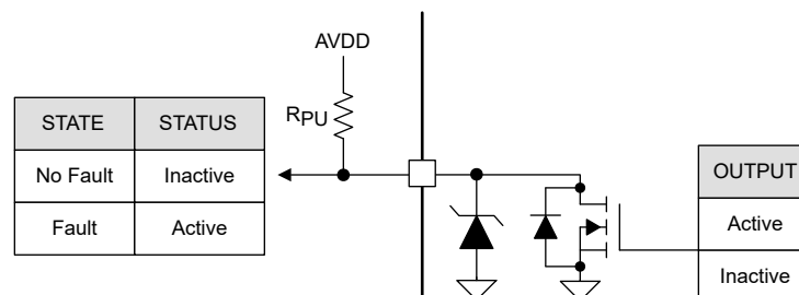
7-8. Open-Drain Output Pin Structure
