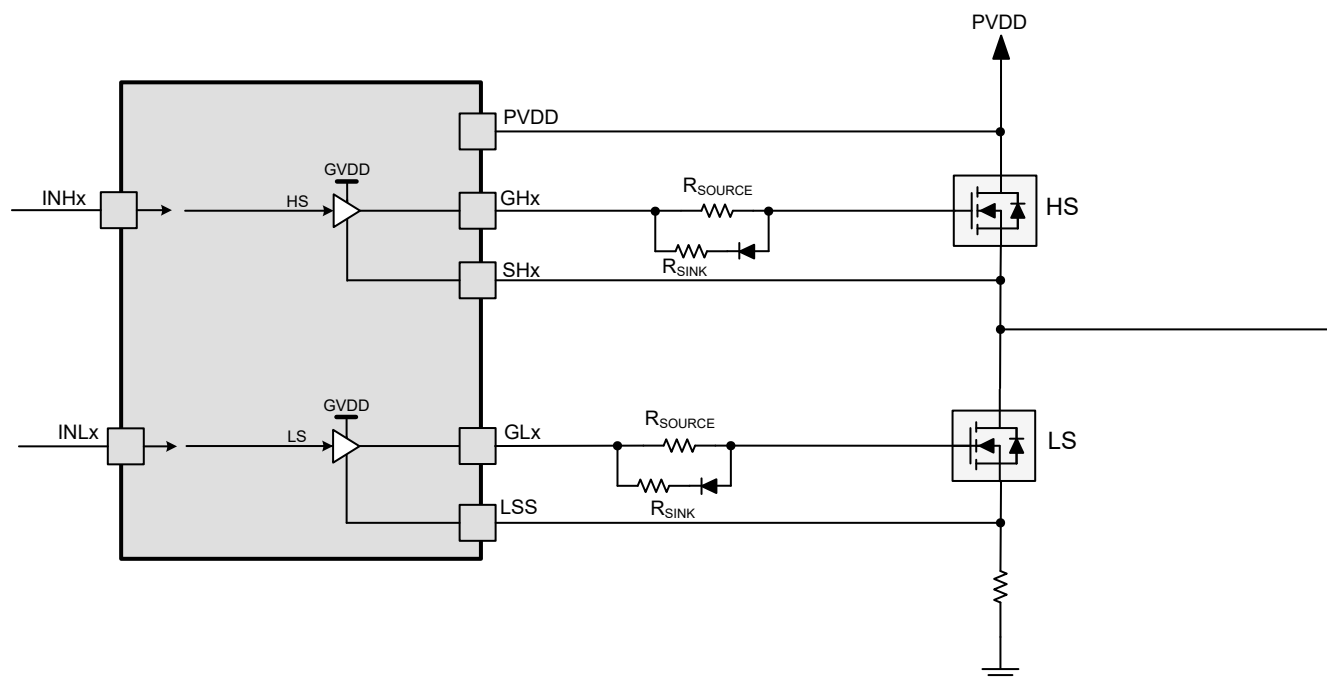
FIG 9-4. Gate driver outputs with separate source and sink current paths
