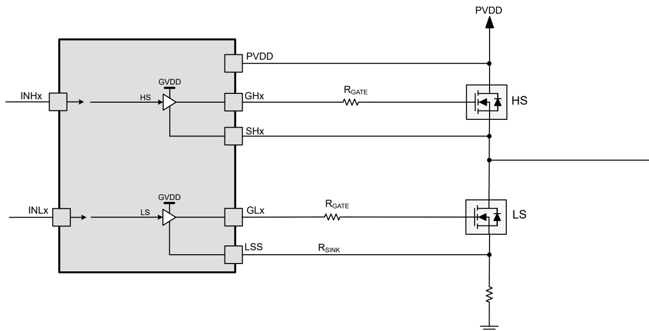
FIG 9-3. Gate driver outputs with series resistors
