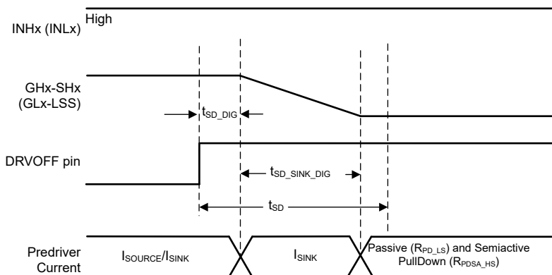
8-9. Gate Driver Shutdown Sequence
