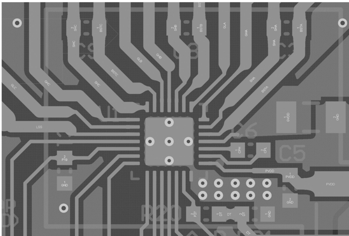
❏ 11-2. Layout of DRV8328 device
