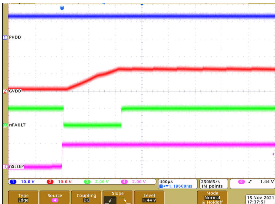
9-9. Device Powerup with nSLEEP
