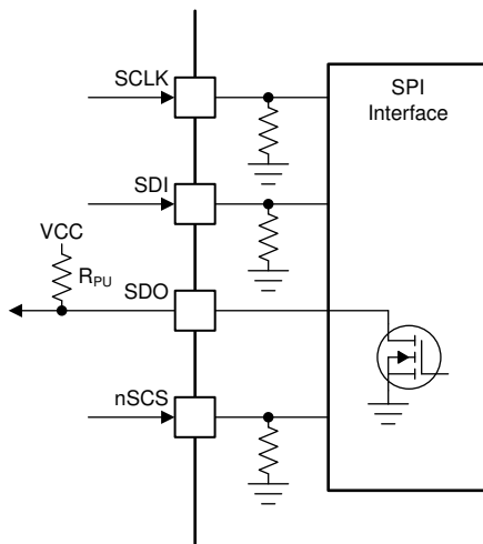
Figure 23. SPI
