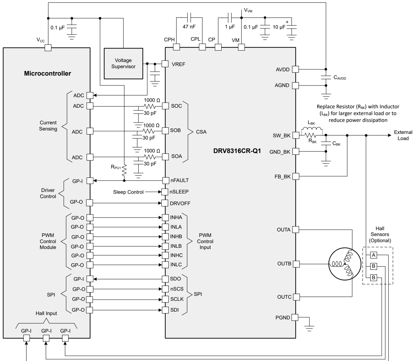
図 9-1. Primary Application Schematic
