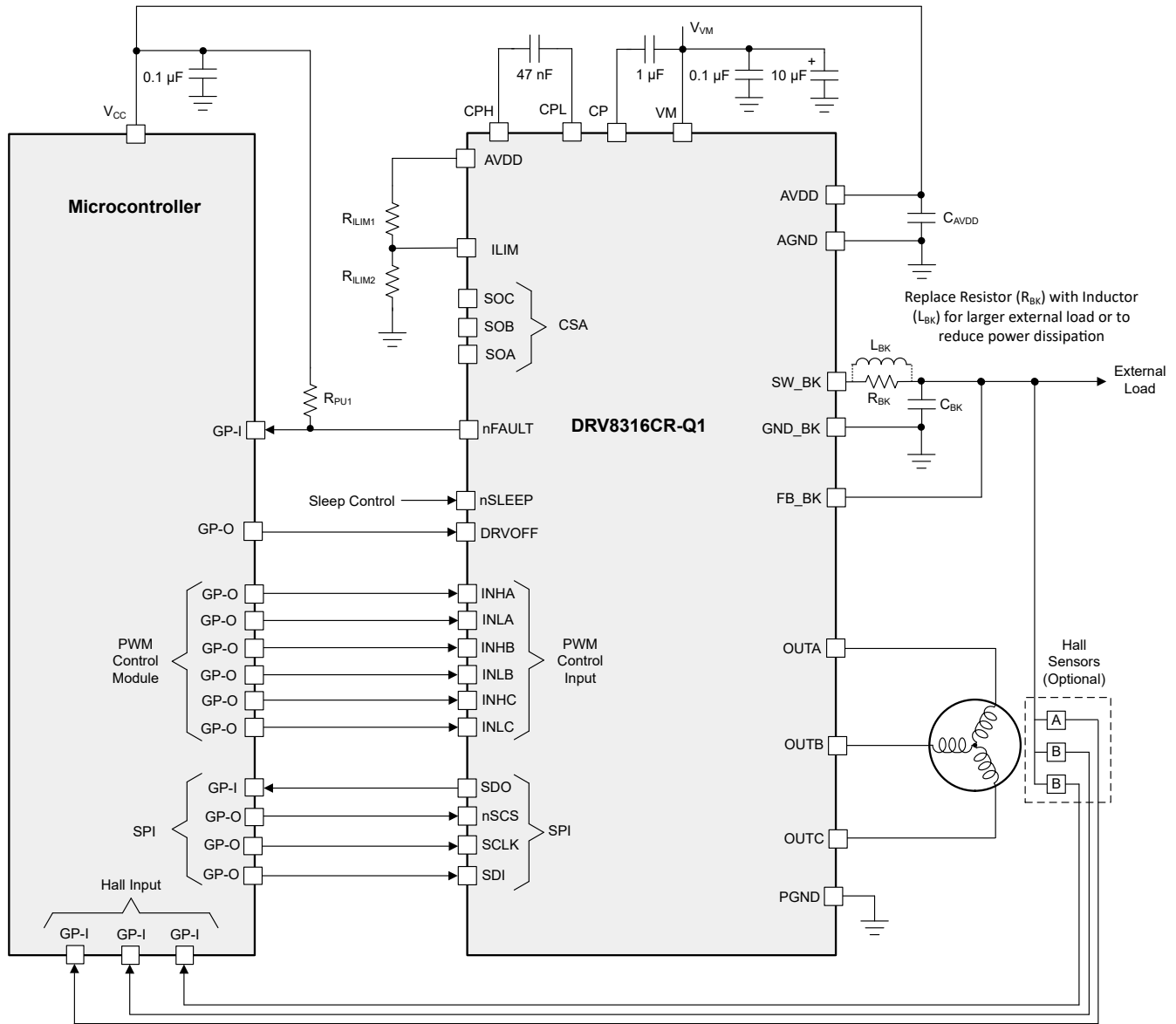
9-10. Alternate Application - BLDC Motor Control with Current Limit
