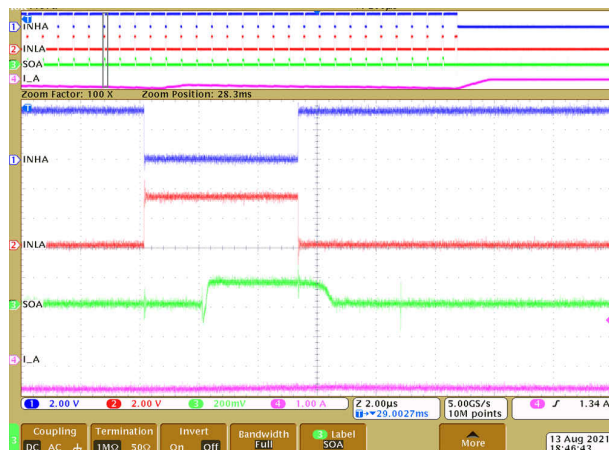
9-6. Driver PWM operation with feedback
