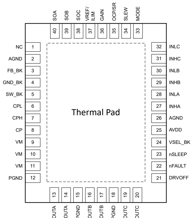
图 6-2. DRV8316CT-Q1 40-Pin VQFN With Exposed Thermal Pad Top View
