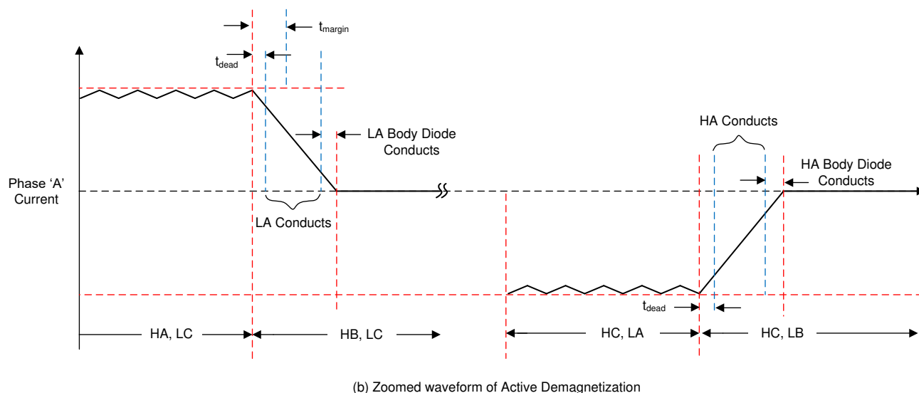
8-33. Current Waveforms for ASR in BLDC Motor Commutation
