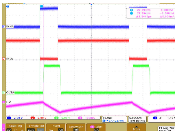
9-9. Driver delay compensation (1.8 µs)
