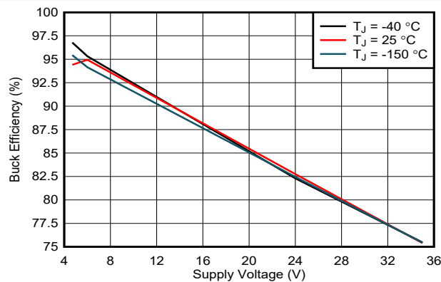
FIG 7-4. Buck regulator efficiency over supply voltage
