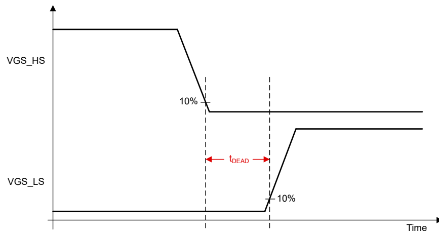
Figure 8-19. Dead Time
