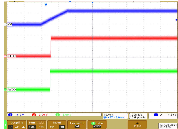
9-7. Power management
