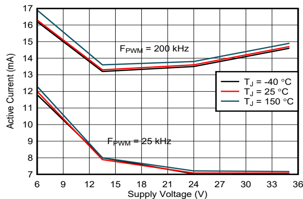
FIG 7-2. Supply current over supply voltage
