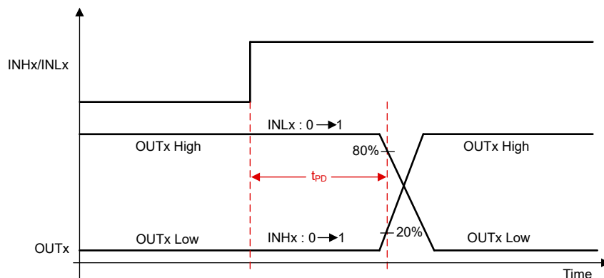
FIG 8-20. Propagation Delay
