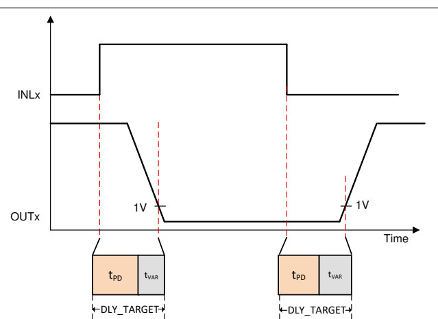
FIG 8-22. Delay Compensation with current flowing into the phase
