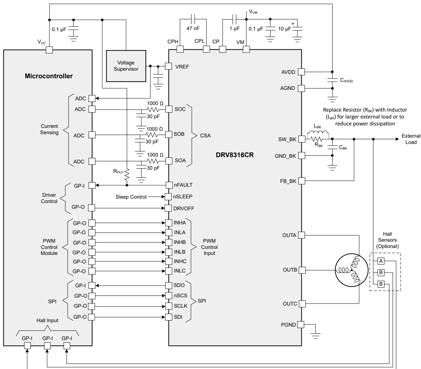
図 9-1. Primary Application Schematics
