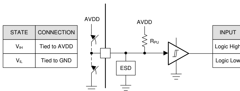
✎ 8-24. Logic nSCC
