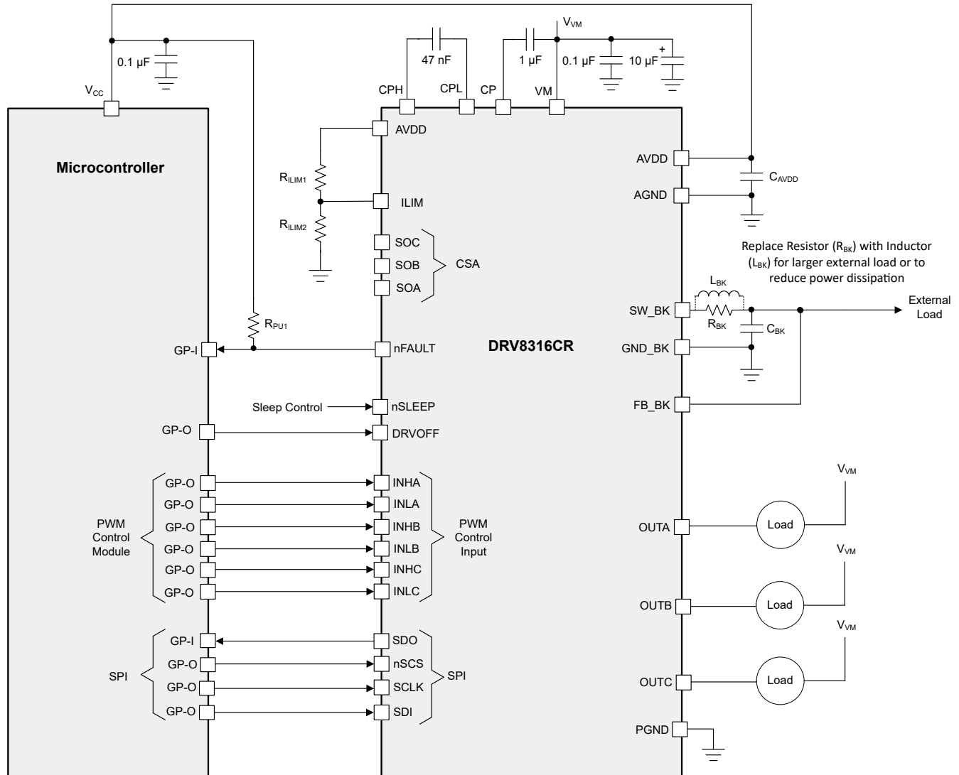
9-14. Alternate Application - Three Solenoid Loads with Current Limit
