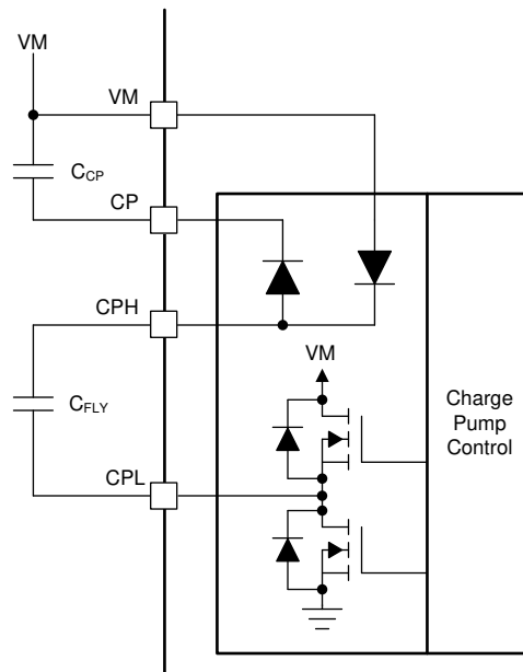
図 8-15. DRV8316C Charge Pump
