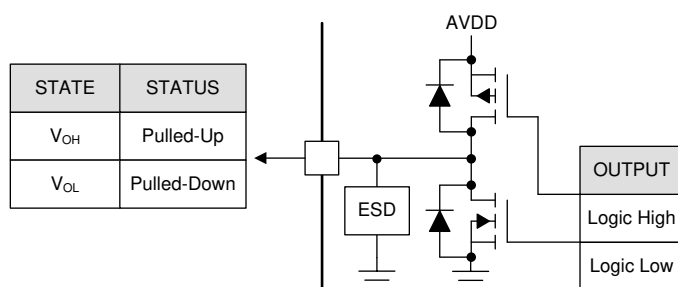
8-26. Push Pull
