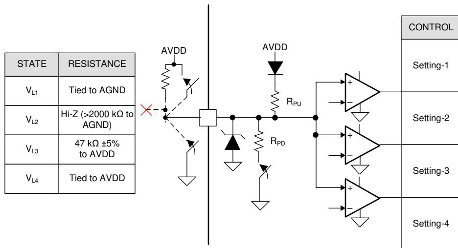
8-27. Four Level Input Pin Structure
