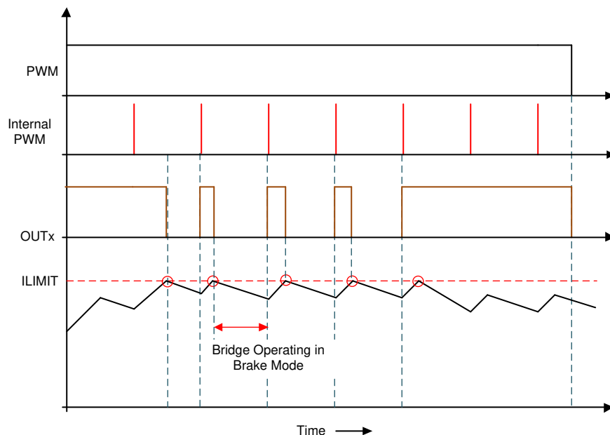
Figure 8-40. Cycle-by-Cycle Current-Limit Operation with 100% PWM Duty Cycle
