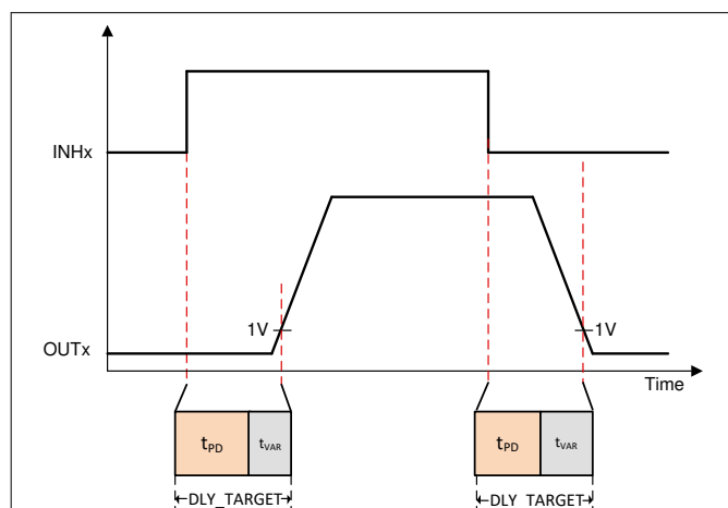
FIG 8-21. Delay Compensation with current flowing out of phase
