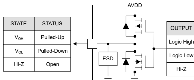
Figure 8-26. Push-Pull Output Pin Structure
