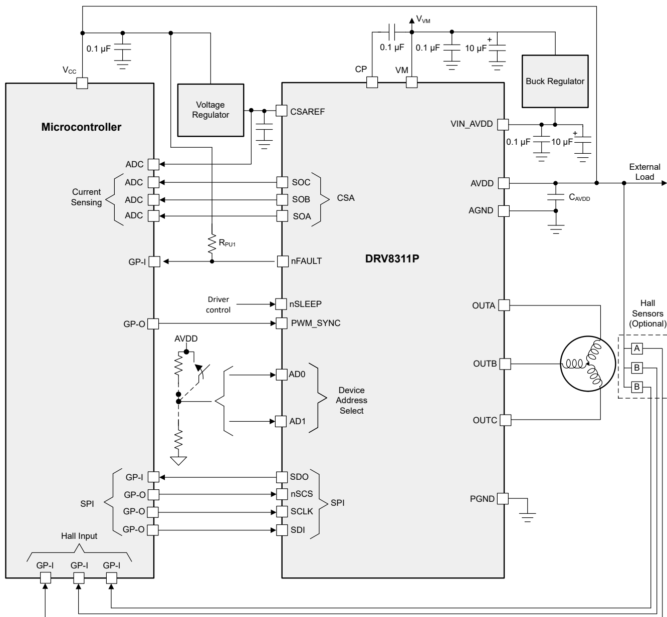
10-6. Application Schematics (DRV8311P) - Three Phase Brushless-DC tSPI Motor Control
