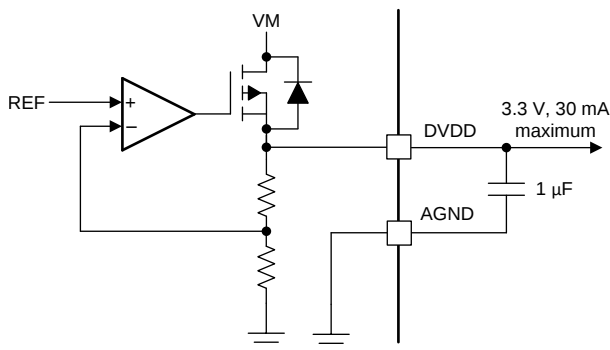
FIG 24. DVDD Linear Regulator Block Diagram
