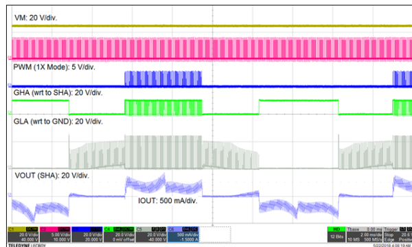
図 50. Gate Drive 20% Duty Cycle
