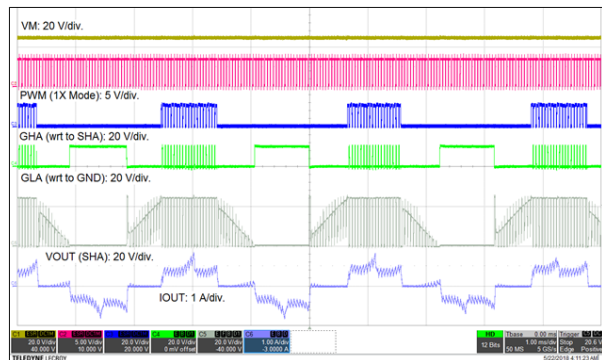
図 49. Gate Drive 80% Duty Cycle
