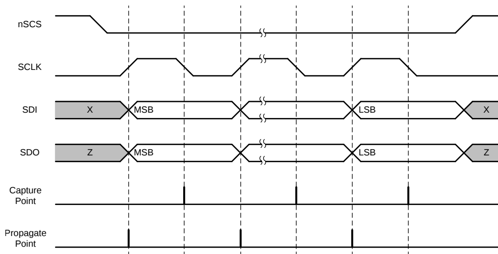
図 37. SPI Slave Timing Diagram
