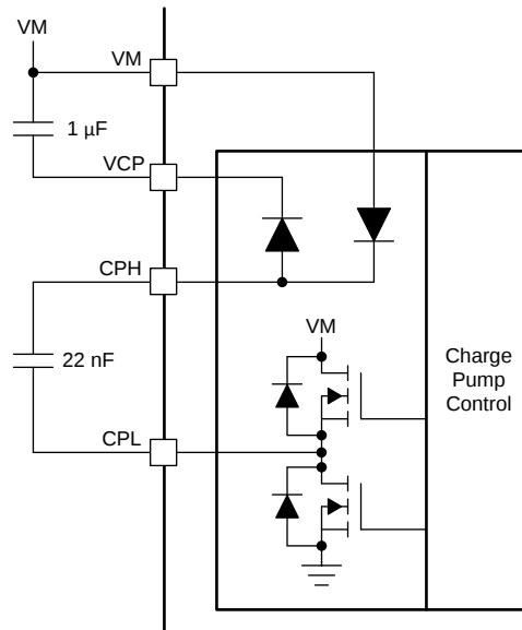
FIG 19. Charge Pump Architecture
