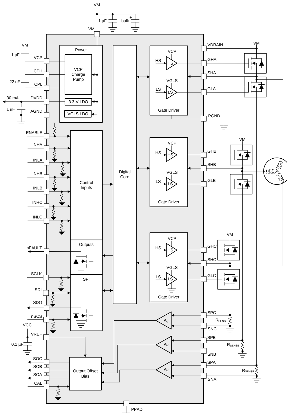
FIG 11. Block Diagram for DRV8304S
