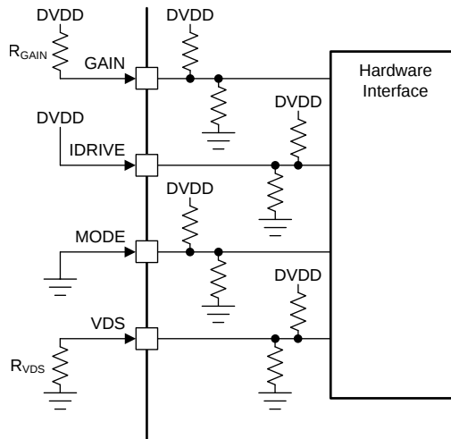
FIG 18. Hardware Interface
