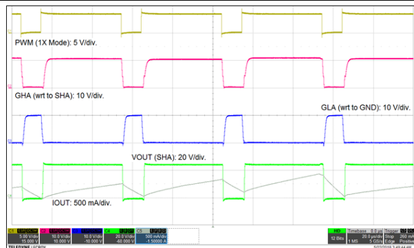
図 47. IDRIVE Maximum Setting
