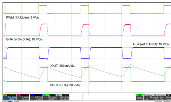
図 48. IDRIVE Minimum Setting
