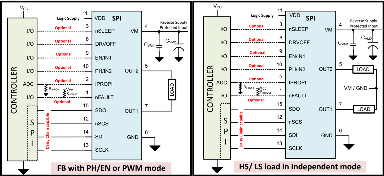
9-5. Typical Application Schematic - SPI Variant
