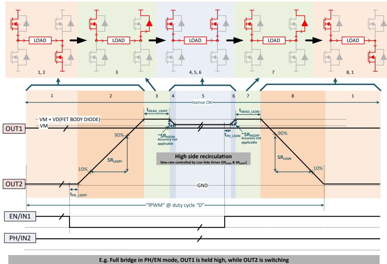
図 6-2. Output Switching Transients for a H-Bridge with High-Side Recirculation
