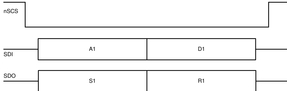
図 7-8. SPI Data - Standard "16-bit" Frame
