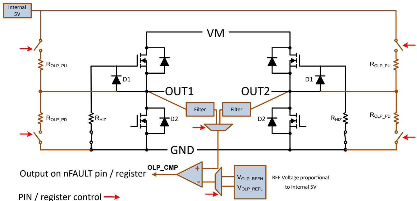
図 7-5. Off-State Diagnostics for full-bridge Load (PH/EN or PWM Mode)
