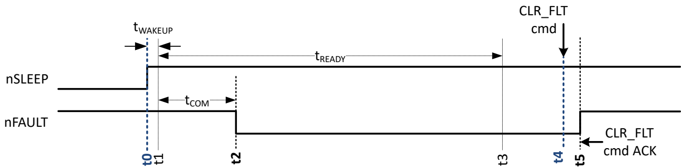
FIG 6-6. Wake-up from SLEEP State to STANDBY State
