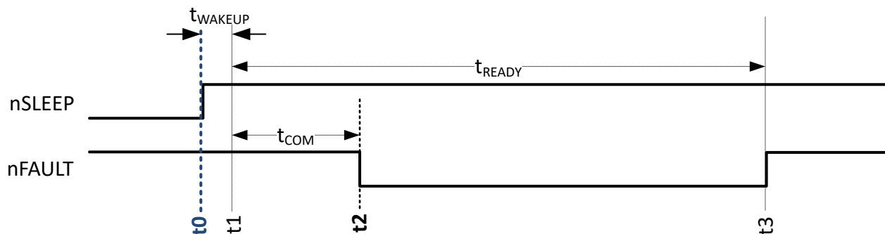
図 6-3. Wake-up from SLEEP State to STANDBY State
