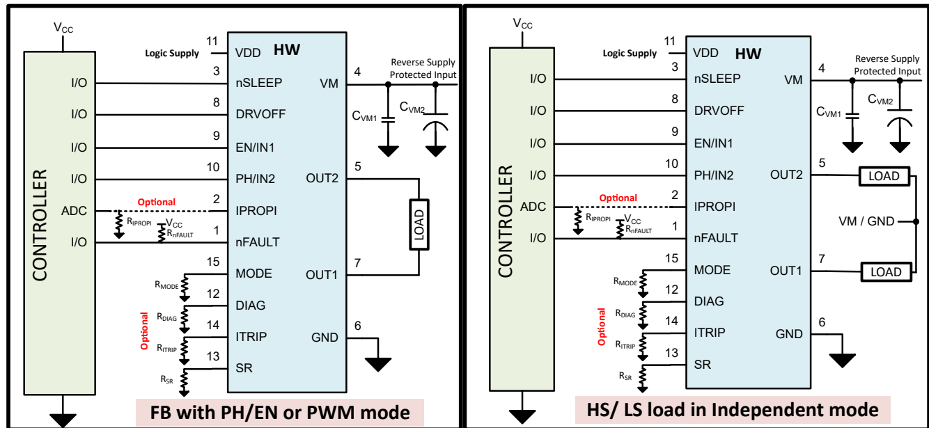
图 9-4. Typical Application Schematic - HW Variant
