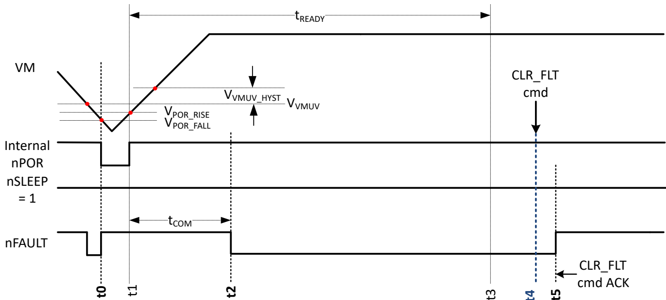
FIG 6-7. Power-up via VM to STANDBY State Transition
