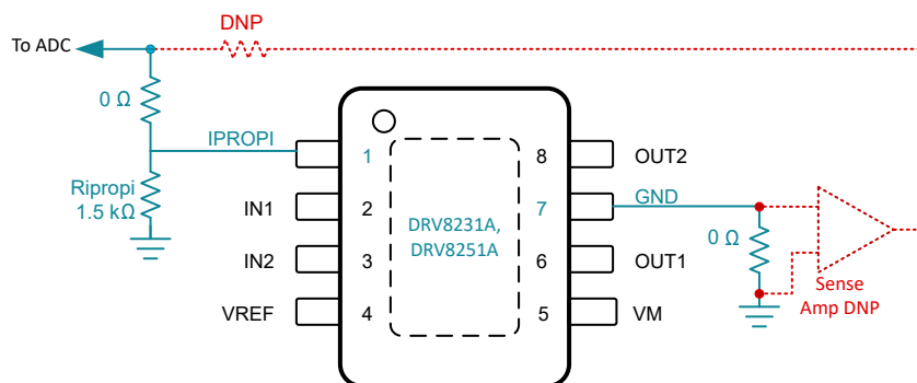
FIG 9-17. DRV8231A/51A Device Using IPROPI to Integrate The Current Sense Function into The Motor Driver
