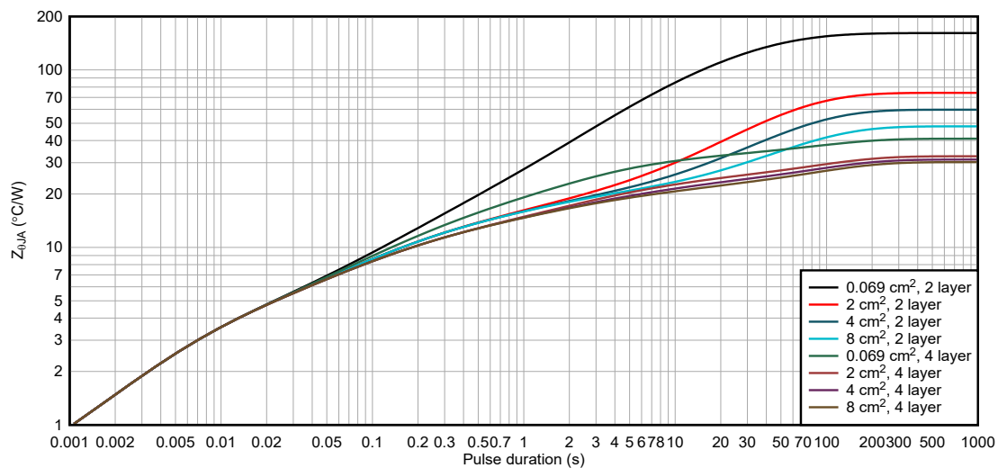
FIG 9-22. HSOP package junction-to-ambient thermal impedance for 2-oz copper layouts
