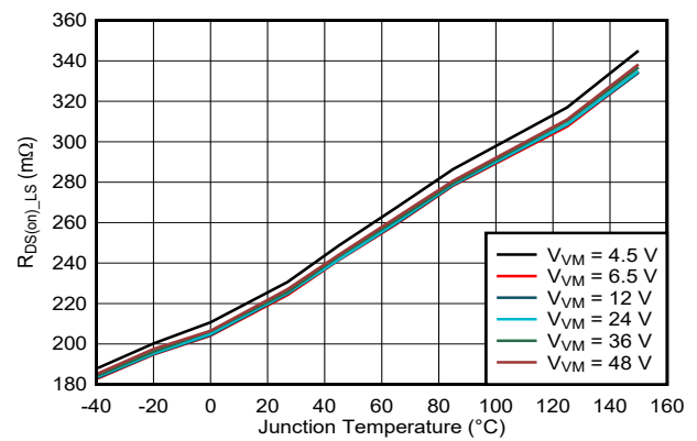
7-8. Low-Side R_{DS(on)} vs. Junction Temperature ( T_J )
