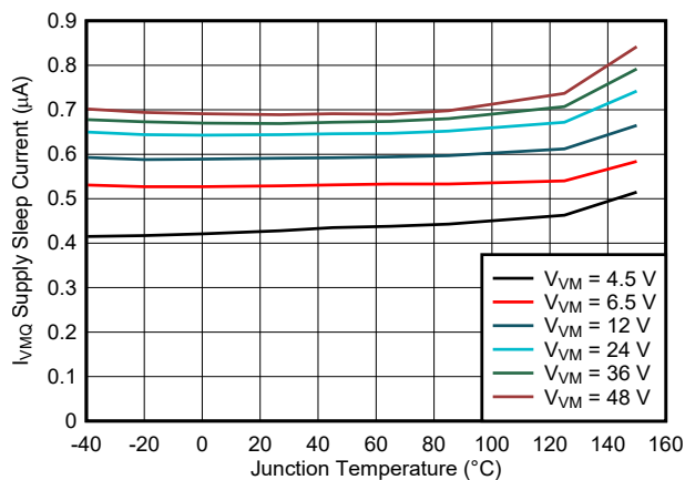
7-2. Sleep Current ( I_{VMQ} ) vs. Junction Temperature ( T_J )
