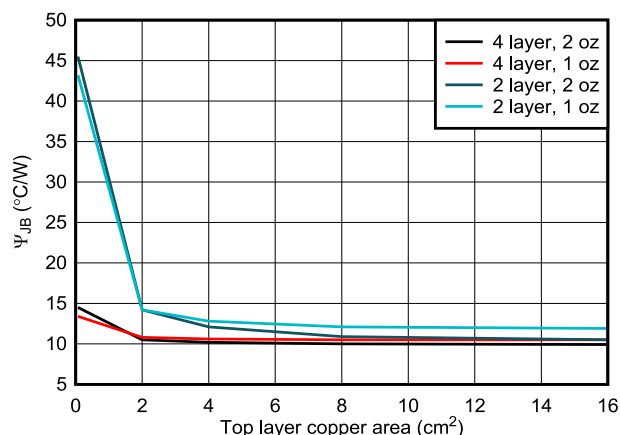
9-20. HSOP, junction-to-board characterization parameter vs copper area
