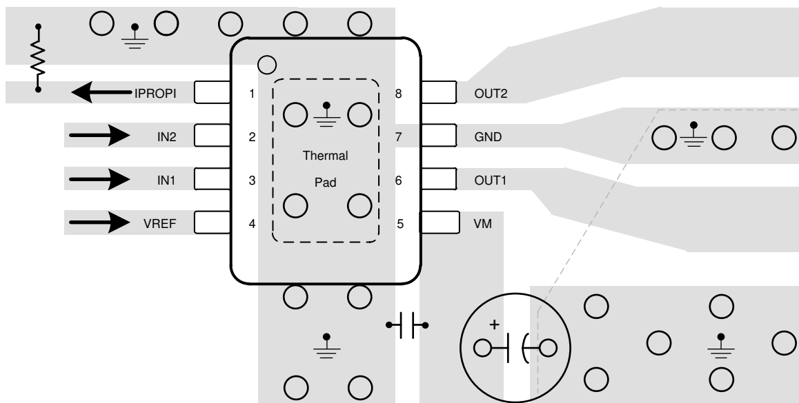
FIG 11-1. Layout Recommendation for DDA Package
