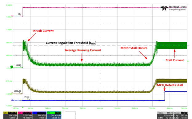
Ch 1 (Yellow) = V_{IPROPI} Ch 2 (Magenta) = IN1 Signal Ch 3 (Blue) = Stall Indication Ch 4 (Green) = Motor Current
