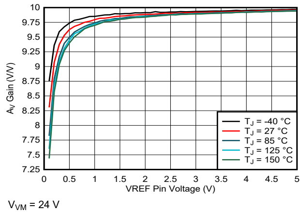
Figure 7-9. Current Regulation Gain ( A_V ) vs. Reference Voltage ( V_{REF} )
