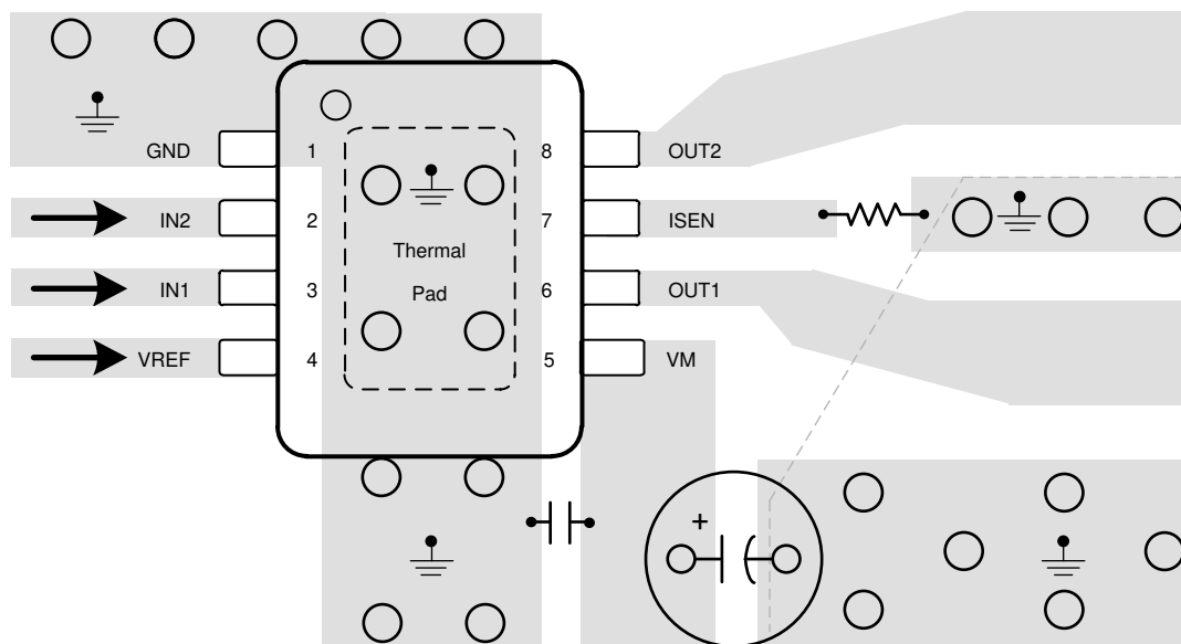
✎ 11-1. Layout Recommendation
