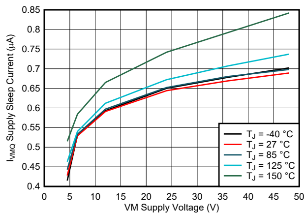
Fig 7-1. Sleep Current ( I_{VMQ} ) vs. Supply Voltage ( V_{VM} )
