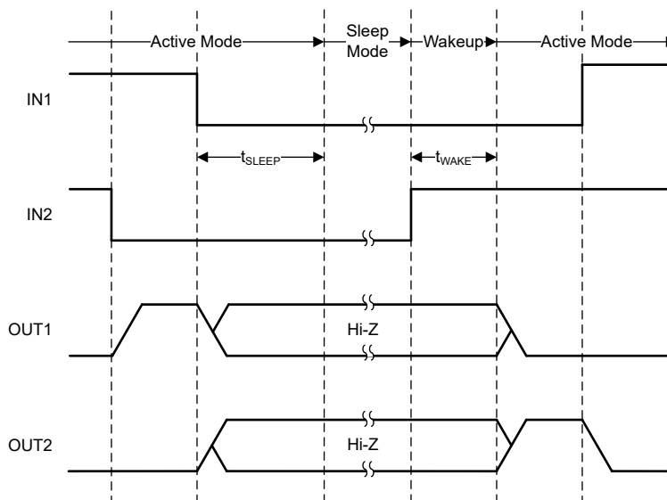
8-5. Sleep Mode Entry and Wakeup Timing Diagram
