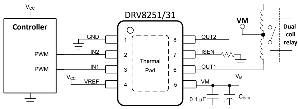
9-10. Dual-Coil Relay Driving
