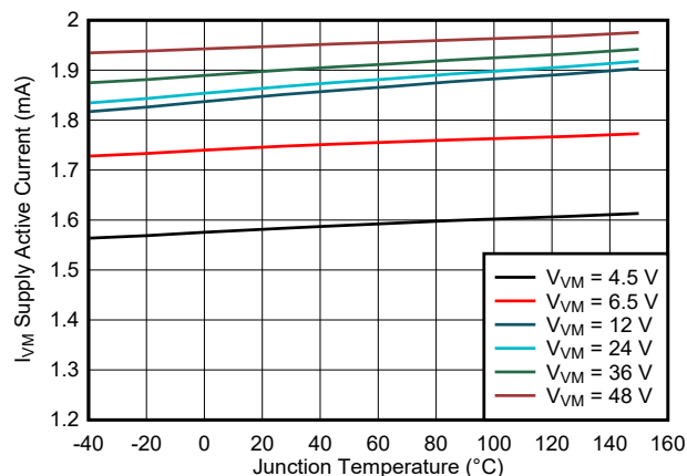
Fig 7-4. Active Current ( I_{VM} ) vs. Junction Temperature ( T_J )
