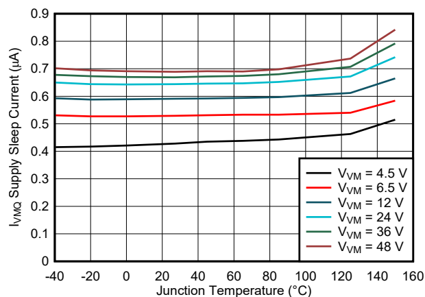
Fig 7-2. Sleep Current ( I_{VMQ} ) vs. Junction Temperature ( T_J )
