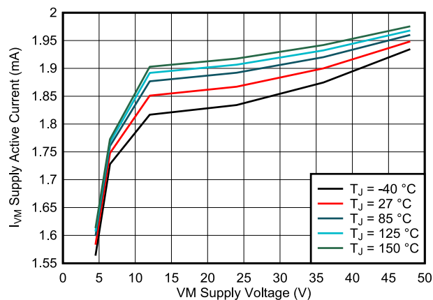
Fig 7-3. Active Current ( I_{VM} ) vs. Supply Voltage ( V_{VM} )
