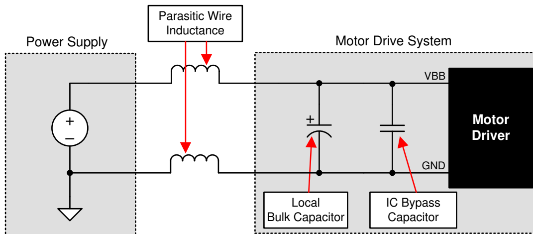
図 10-1. Example Setup of Motor Drive System With External Power Supply
