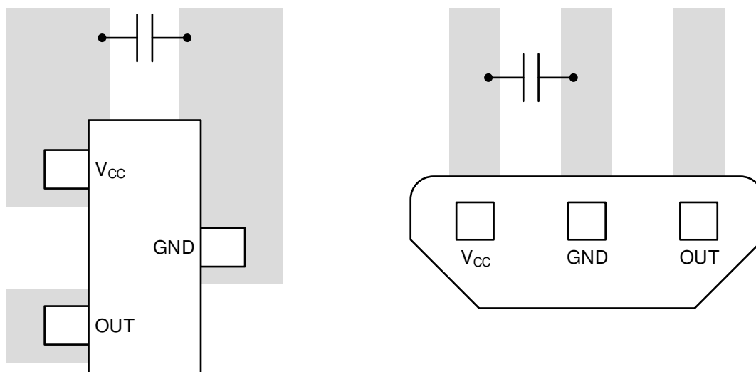
10-1. Layout Examples
