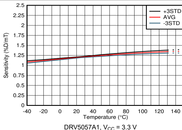
6-8. Sensitivity vs Temperature
