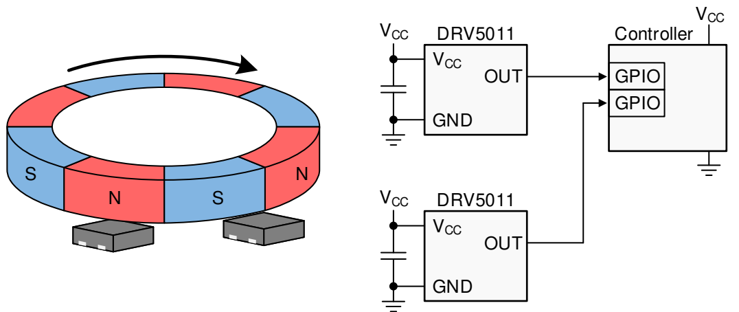
图 14. Incremental Rotary Encoding System
