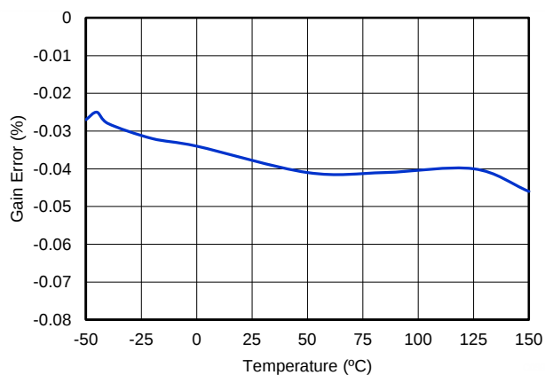
Figure 24. DIFFERENTIAL AMPLIFIER GAIN ERROR vs TEMPERATURE
