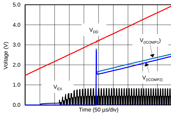
Figure 1. START-UP BEHAVIOR
