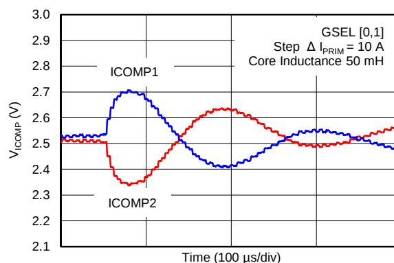
Figure 50. Settling of ICOMP1 and ICOMP2 (Mode Gain_2)
