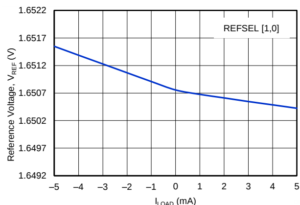
Figure 41. 1.65-V REFERENCE OUTPUT VOLTAGE vs LOAD CURRENT
