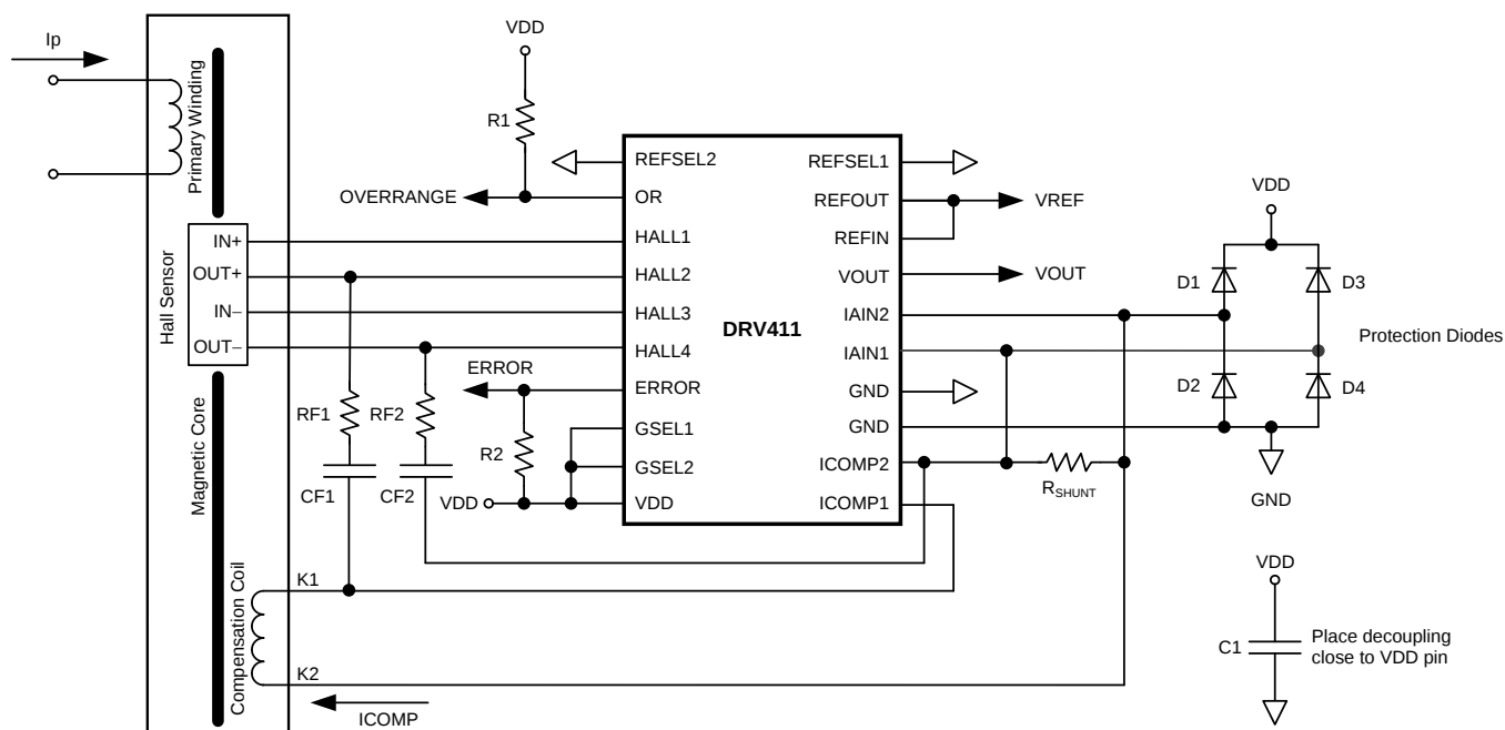
Figure 57. Application Example with External Gain and Compensation Setting (GSEL1 and GSEL2 set High), No Current Spinning
