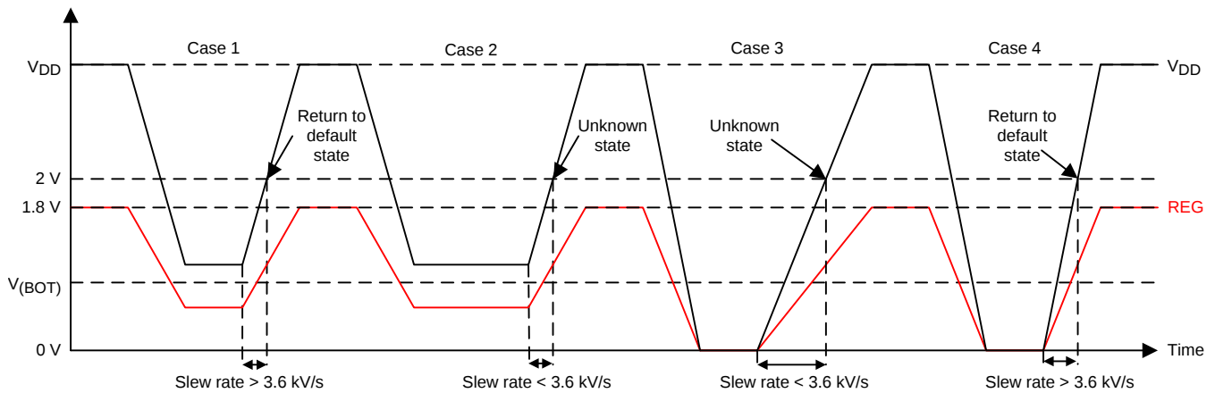
Figure 15. Brownout Behavior
