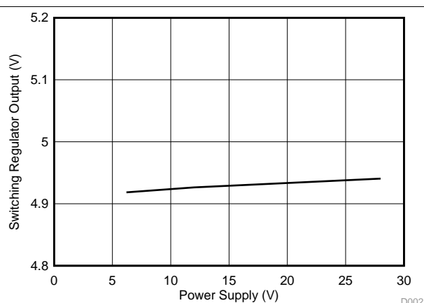
FIG 2. Switching Regulator Output vs Power Supply Voltage
