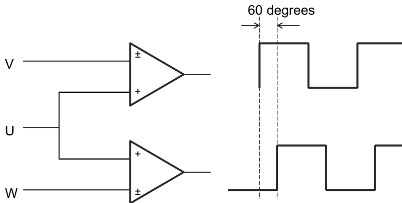
FIG 8-12. Initial Speed Detect Function
