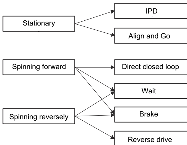
FIG 8-10. Start the Motor Under Different Initial Conditions
