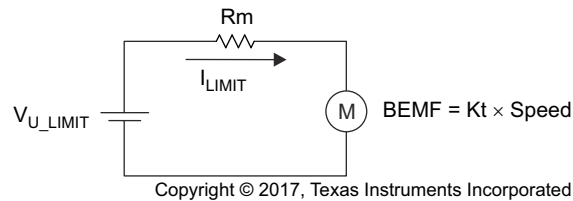
図 8-26. Acceleration Current Limit
