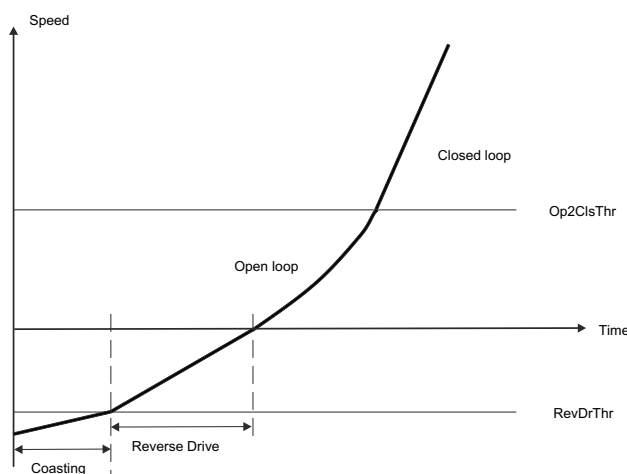
FIG 8-13. Reverse Drive Function
