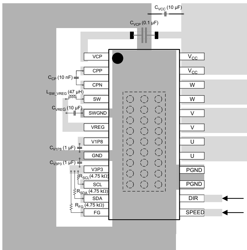
11-1. Layout Diagram
