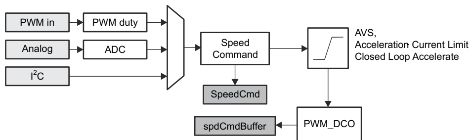
図 8-38. SpeedCmd and spdCmdBuffer Registers
