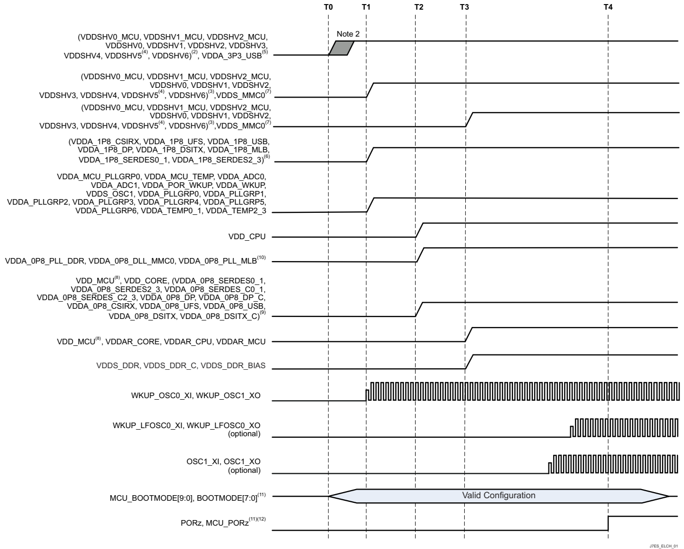
FIG 6-3. Combined MCU and Main Domains, Primary Power-Up Sequence
