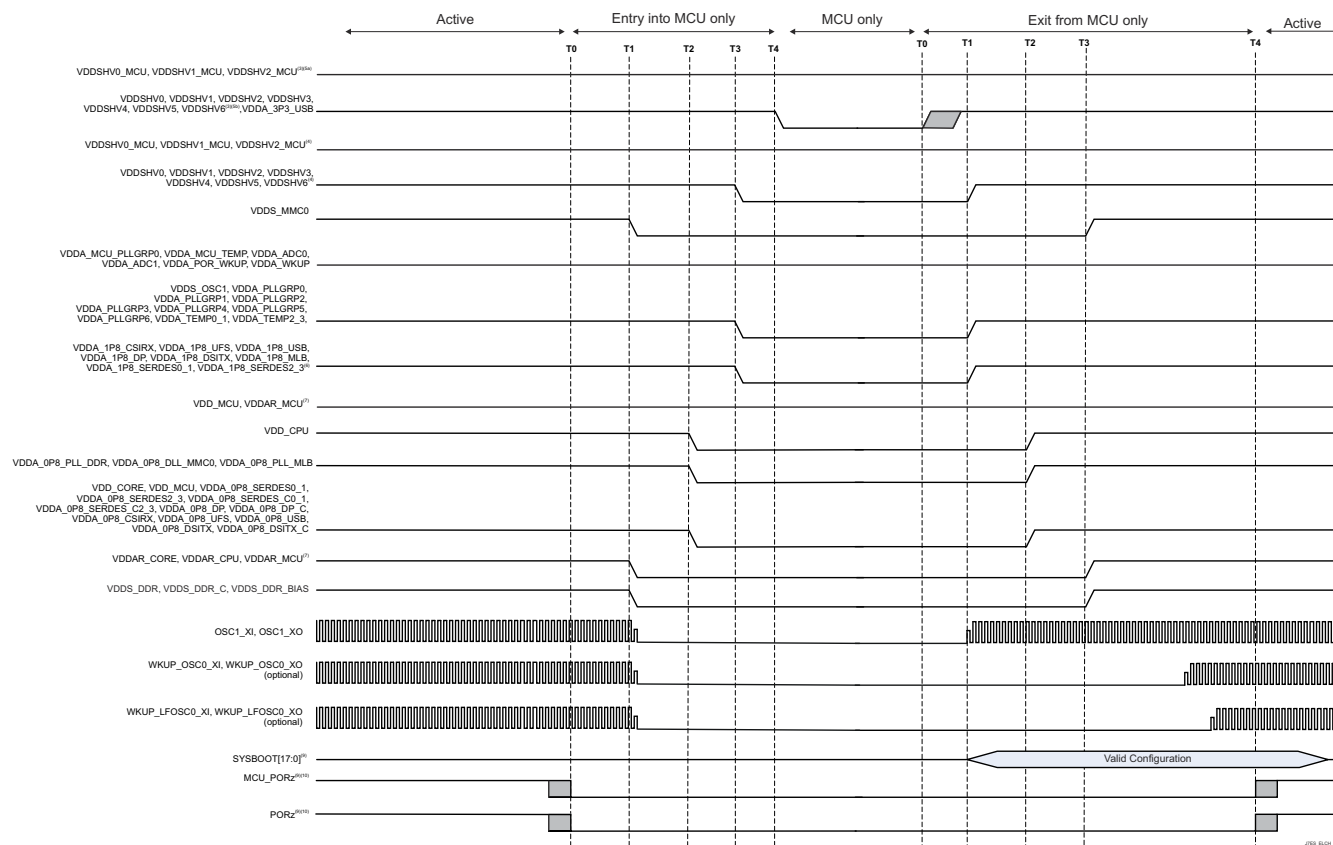
6-7. Entry and Exit of MCU Only Sequencing
