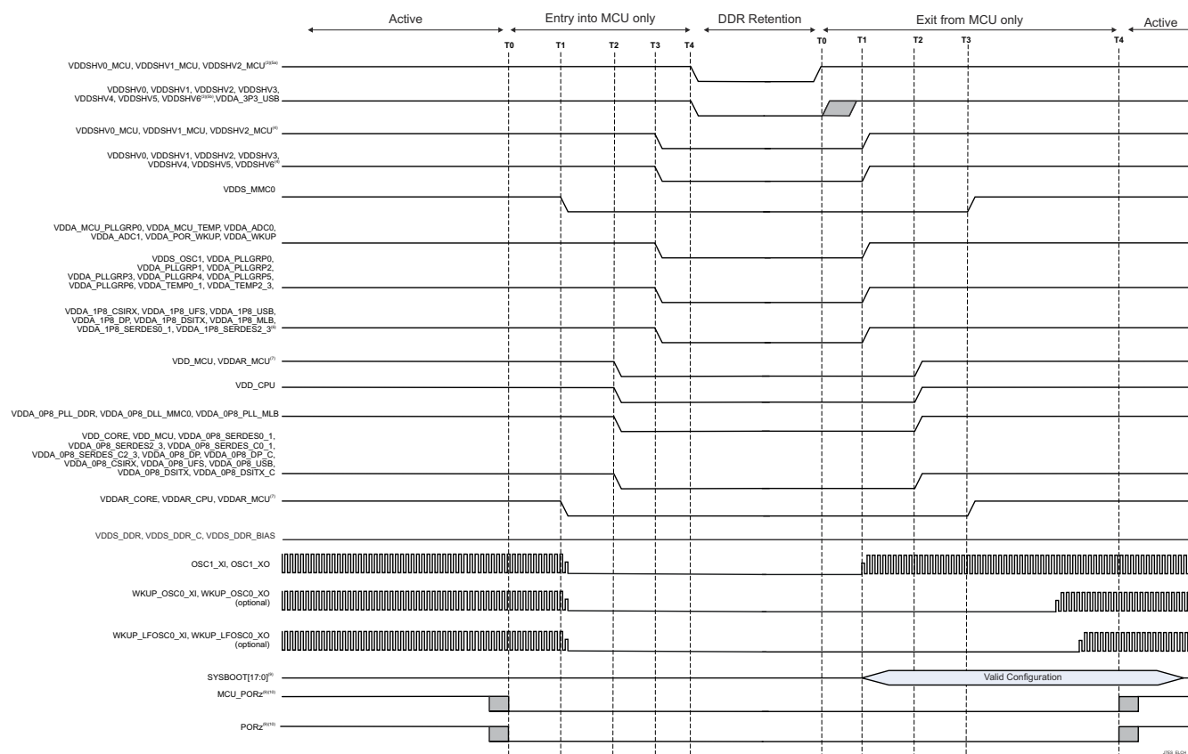
☒ 6-8. Entry and Exit of DDR Retention Sequencing
