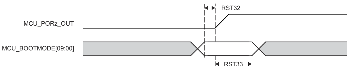
図 6-16. MCU_BOOTMODE Timing Requirements
