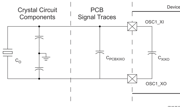
図 6-31. Shunt Capacitance
