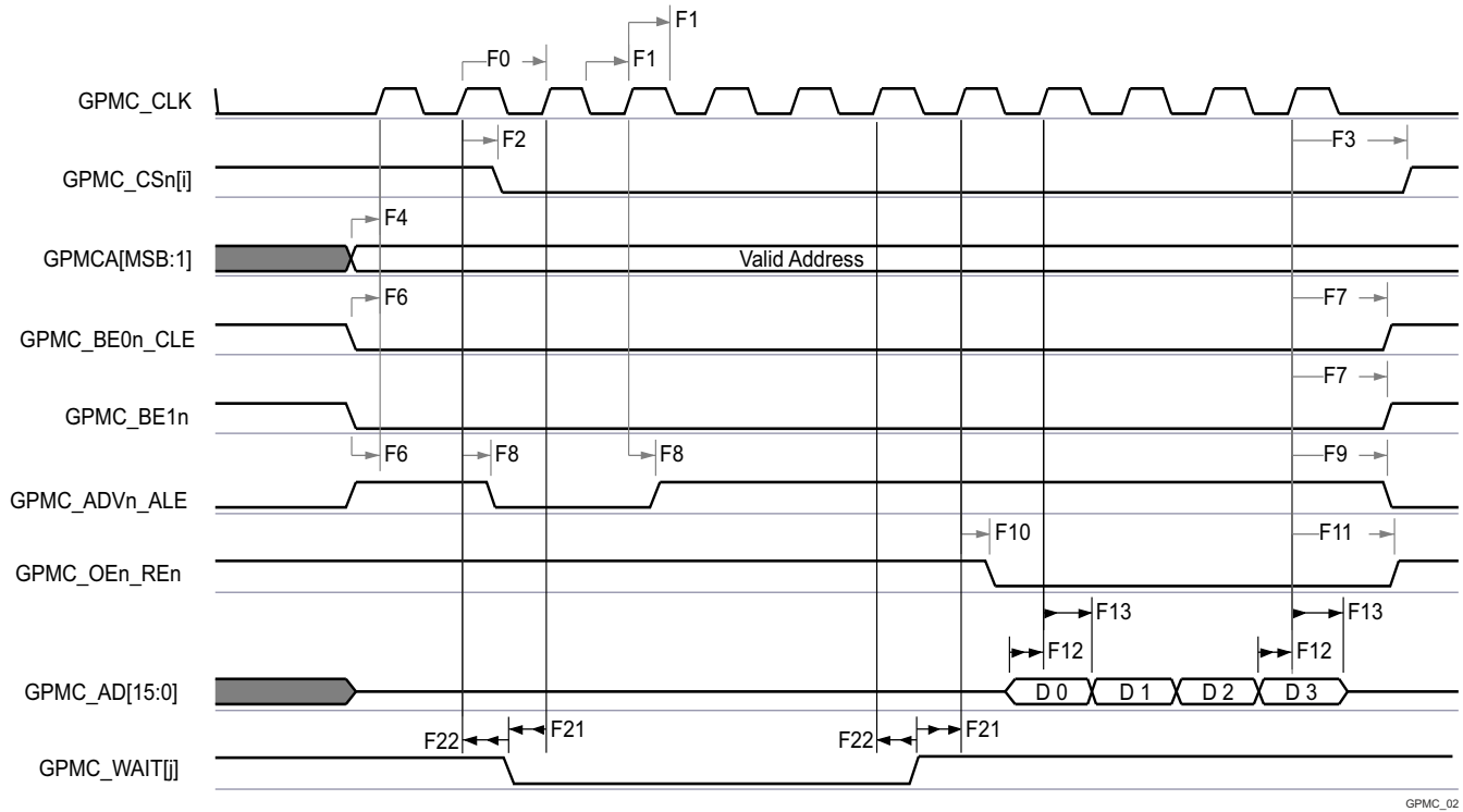
図 6-64. GPMC and NOR Flash — Synchronous Burst Read — 4x16-bit (GPMCFCLKDIVIDER = 0)
