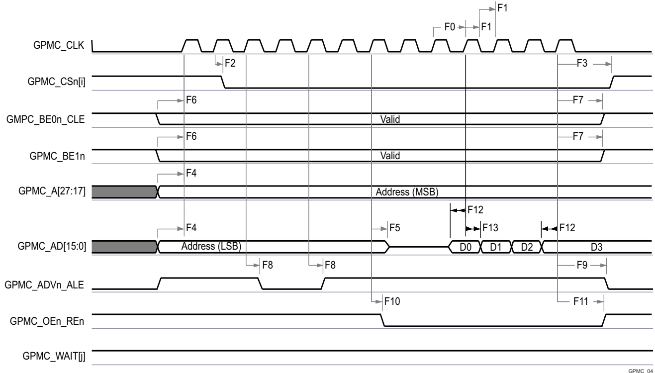
6-65. GPMC and NOR Flash—Synchronous Burst Write (GPMCFCLKDIVIDER = 0)
