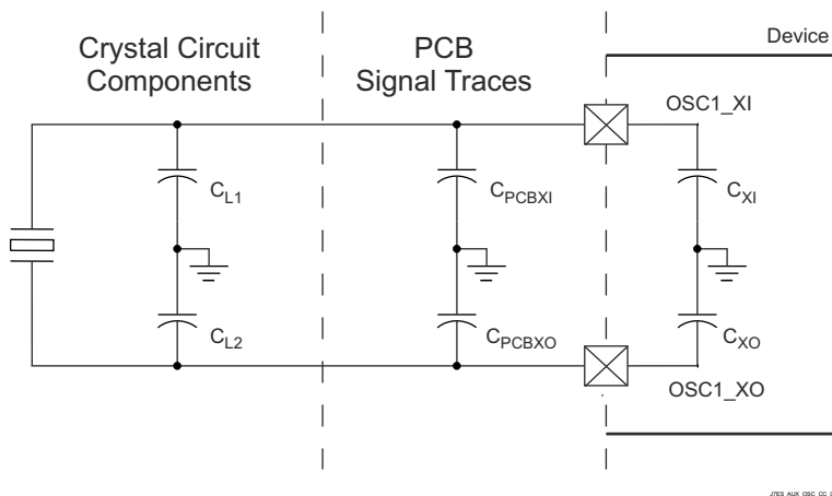
図 6-30. Load Capacitance
