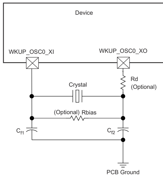
Figure 6-23. WKUP_OSC0 Crystal Implementation
