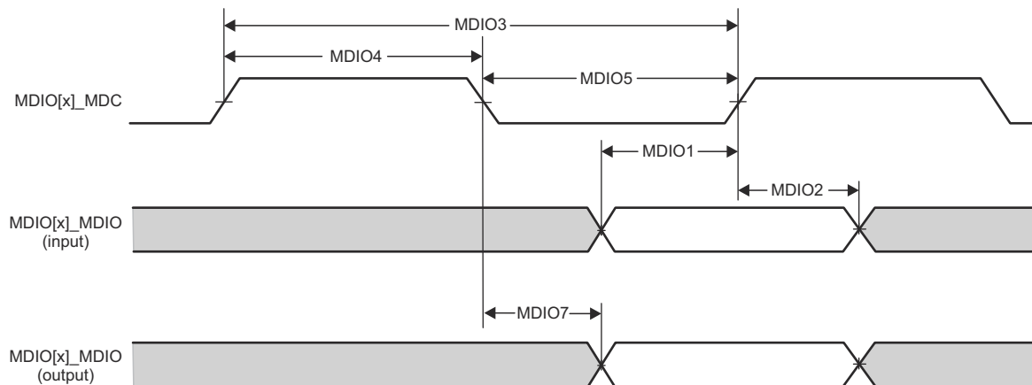
図 6-47. CPSW9G MDIO Diagrams Receive and Transmit
