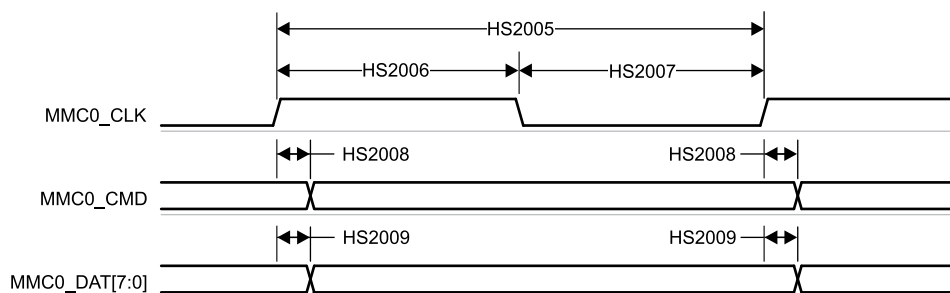
図 6-96. MMC0 – HS200 Mode – Transmit Mode
