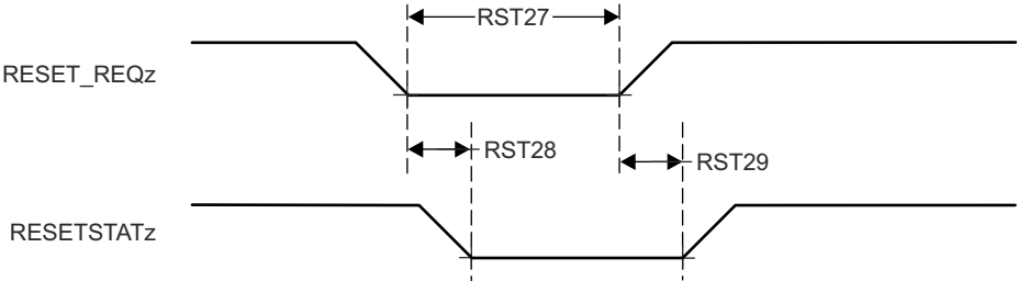
図 6-14. RESET_REQz initiates; RESETSTATz Timing Requirements and Switching Characteristics
