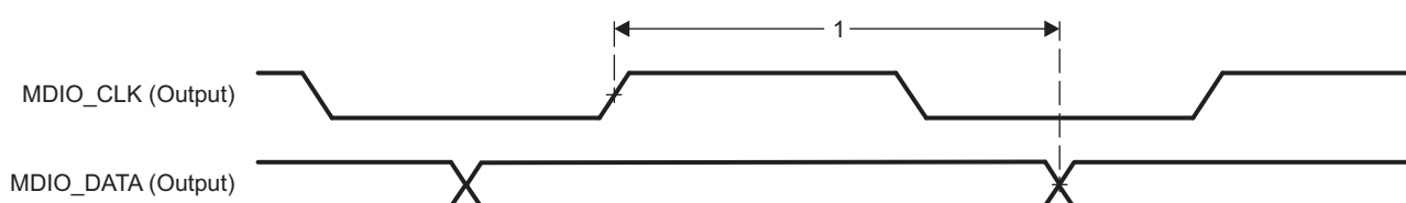
图 5-124. PRU-ICSS MDIO_DATA Timing – Output Mode
