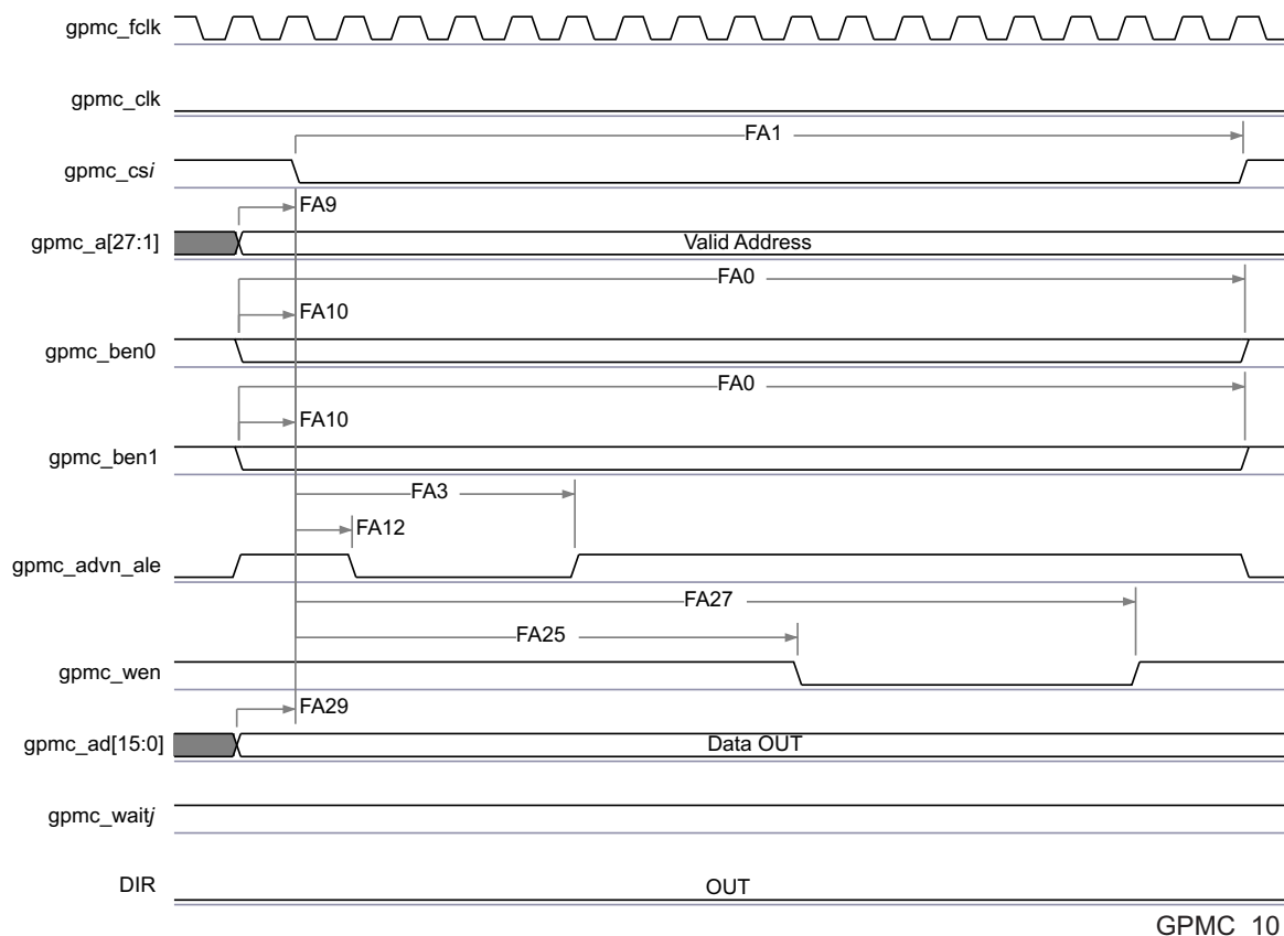
5-32. GPMC / NOR Flash - Asynchronous Write - Single Word (1)
