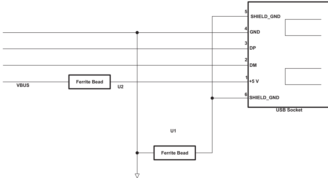
7-23. USB Connector
