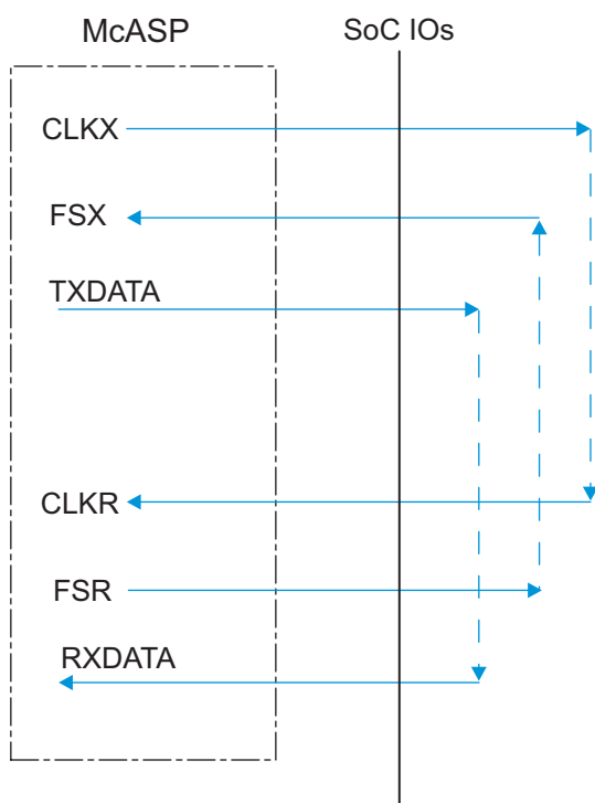
FIG 5-60. McASP1-8 COIFIO – ASYNC Mode
