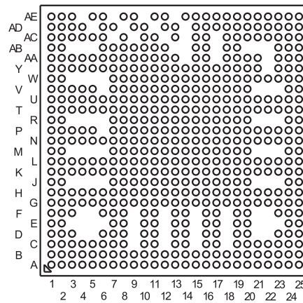
図 4-1. CBD S-PBGA-N538 Package (Bottom View)
