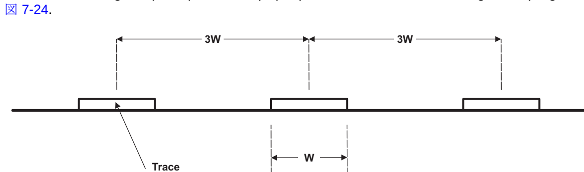
7-24. 3W Spacing Rule
