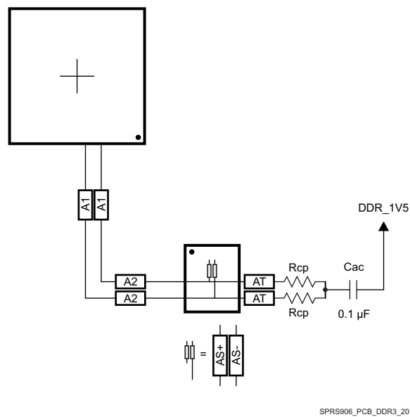
7-56. CK Routing for One DDR3 Device
