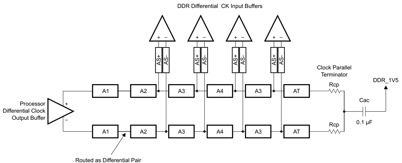
图 8-62. CK Topology for Four x8 DDR3 Devices
