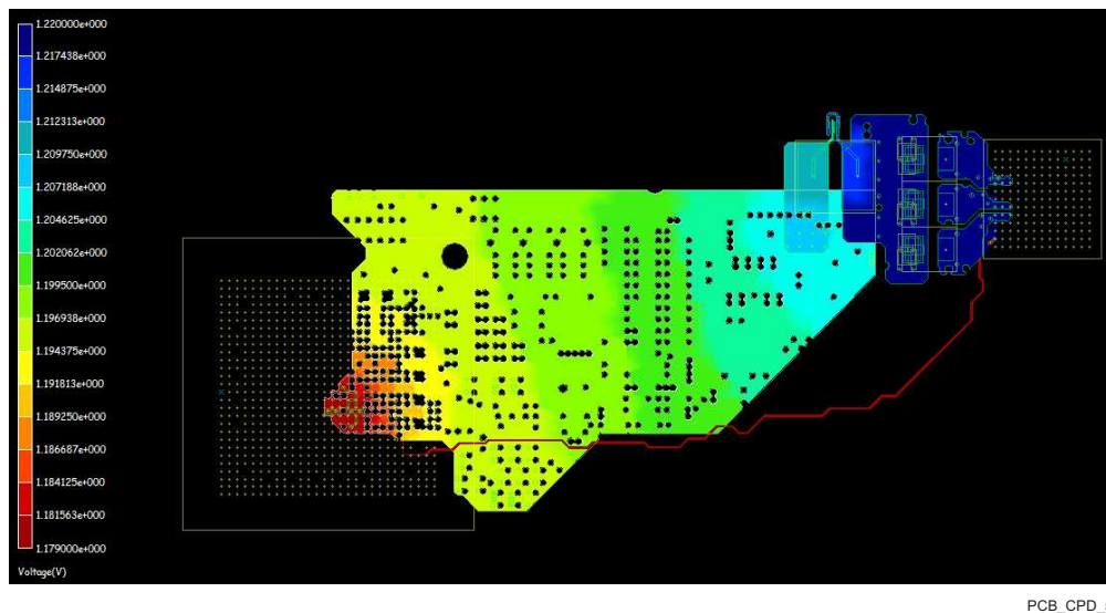
図 8-25. vdd_mpu Voltage/IR Drop [All Layers]
