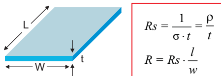
FIG 8-9. Depiction of Sheet Resistivity and Resistance
