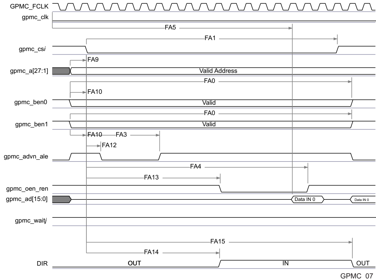
FIG 7-13. GPMC / NOR Flash - Asynchronous Read - Single Word Timing (1)(2)(3)(4)
