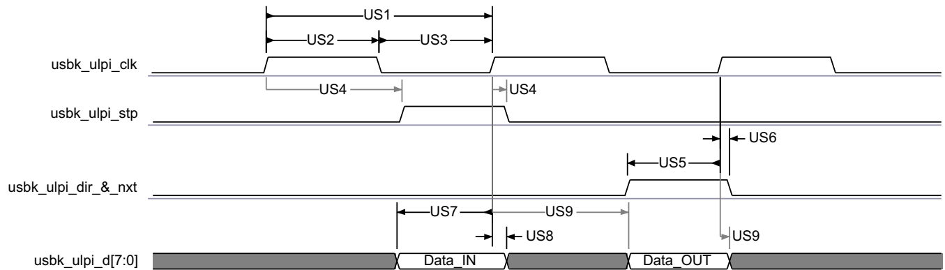
図 7-51. HS USB3 and USB4 ULPI —SDR—Slave Mode—12-pin Mode
