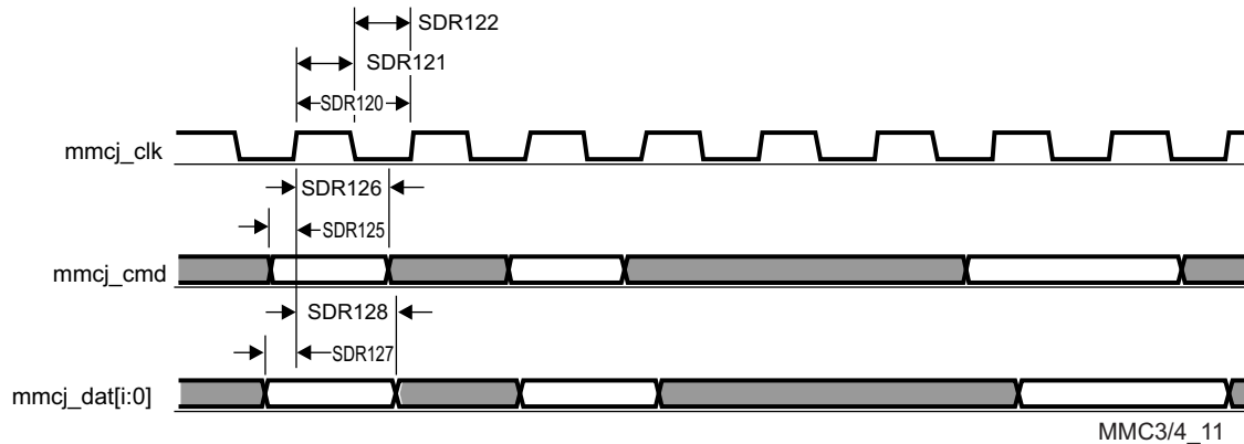
図 7-87. MMC/SD/SDIOj in - SDR12 - Receiver Mode
