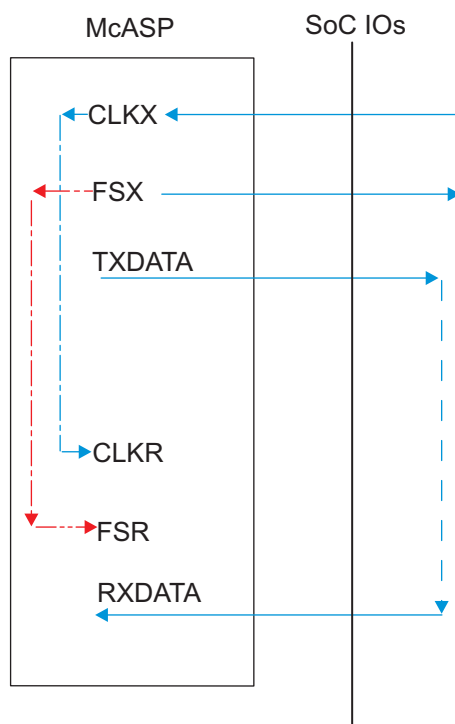
✎ 7-48. McASP1-8 CI-FO- – SYNC Mode
