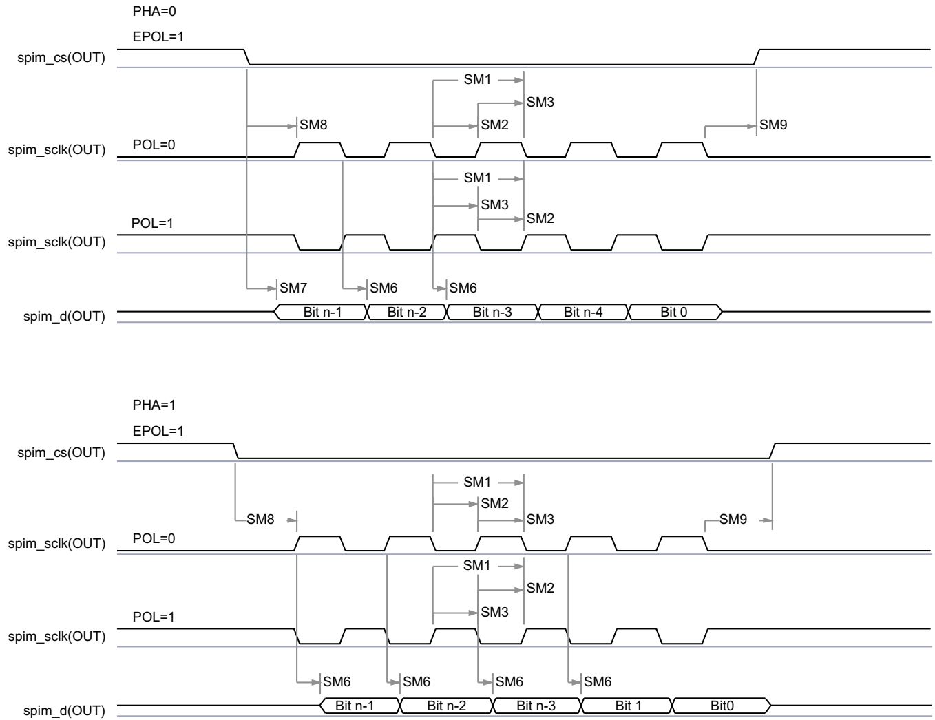
7-33. McSPI - Master Mode Transmit
