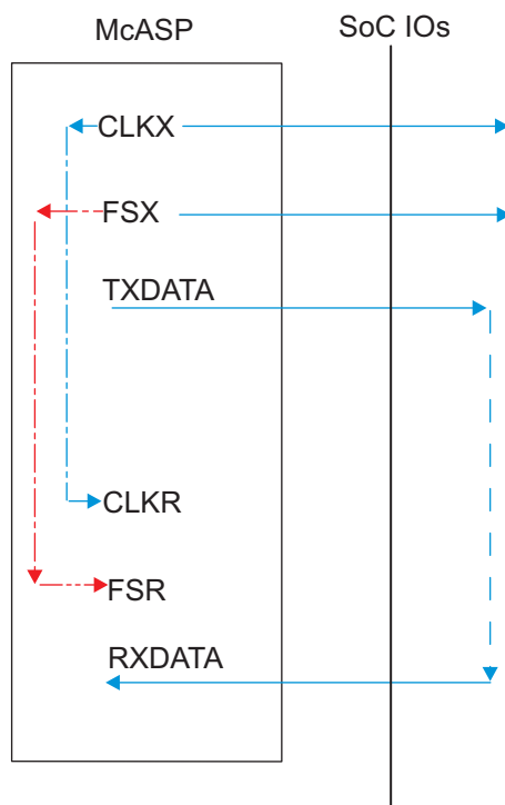
✎ 7-47. McASP1-8 CO-FO- – SYNC Mode
