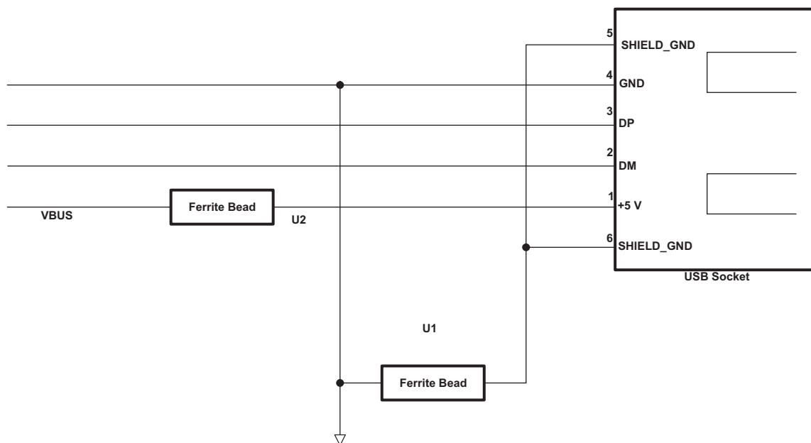
✎ 8-32. USB Connector
