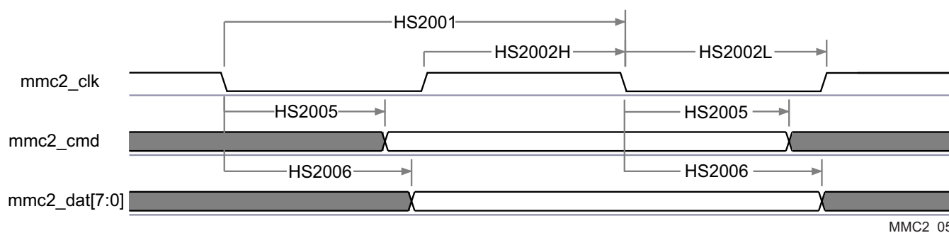
图 7-80. eMMC in - HS200 SDR - Transmitter Mode
