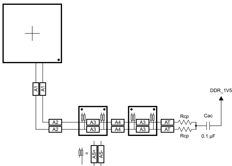
✎ 8-66. CK Routing for Four Mirrored DDR3 Devices
