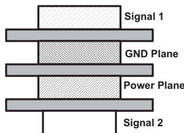
Figure 8-22. Four-Layer Board Stack-Up
