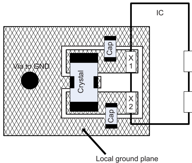
✎ 8-37. Slow Clock PCB Requirements
