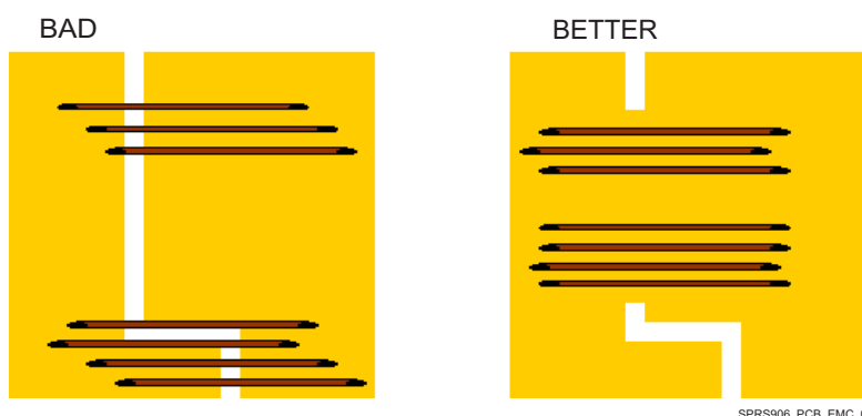
8-11. Trace Examples
