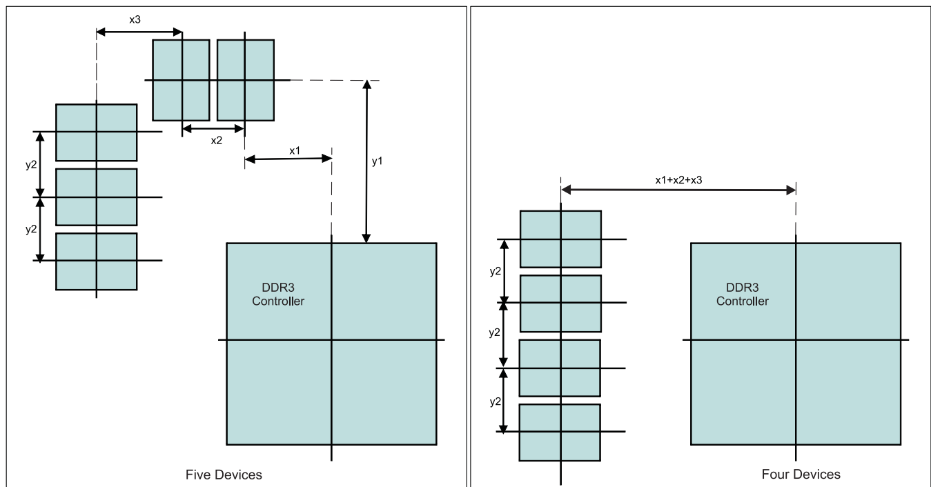
图 8-43. Placement Specifications
