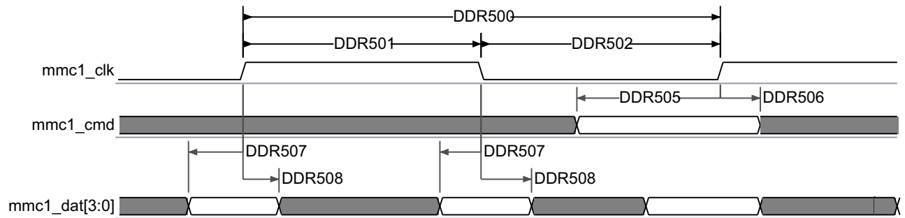
图 7-74. SDRAM - High Speed SD - DDR - Data/Command Receive
