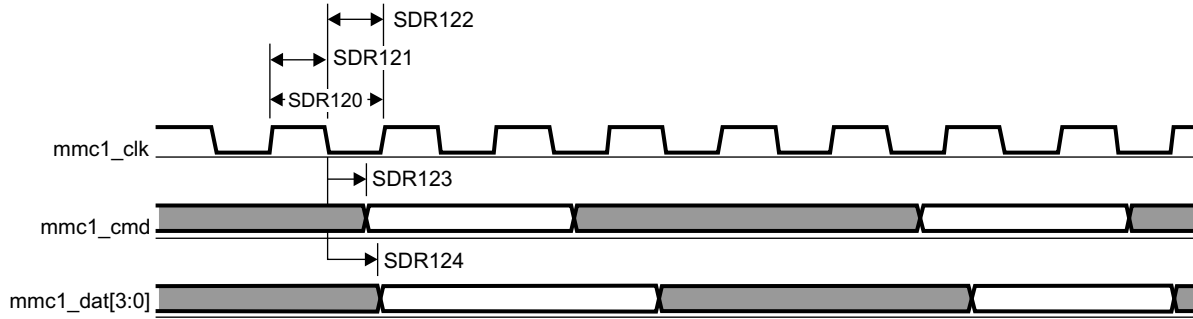
图 7-67. MMC/SD/SDIO in - High Speed SDR12 - Transmitter Mode
