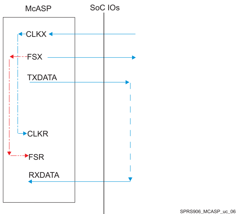
7-48. McASP1-8 CI-FO - SYNC Mode
