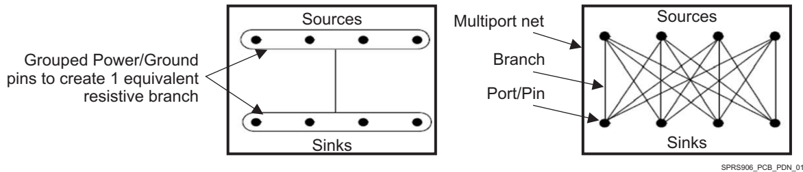
8-5. Pin-grouping concept: Lumped and Distributed Methodologies
