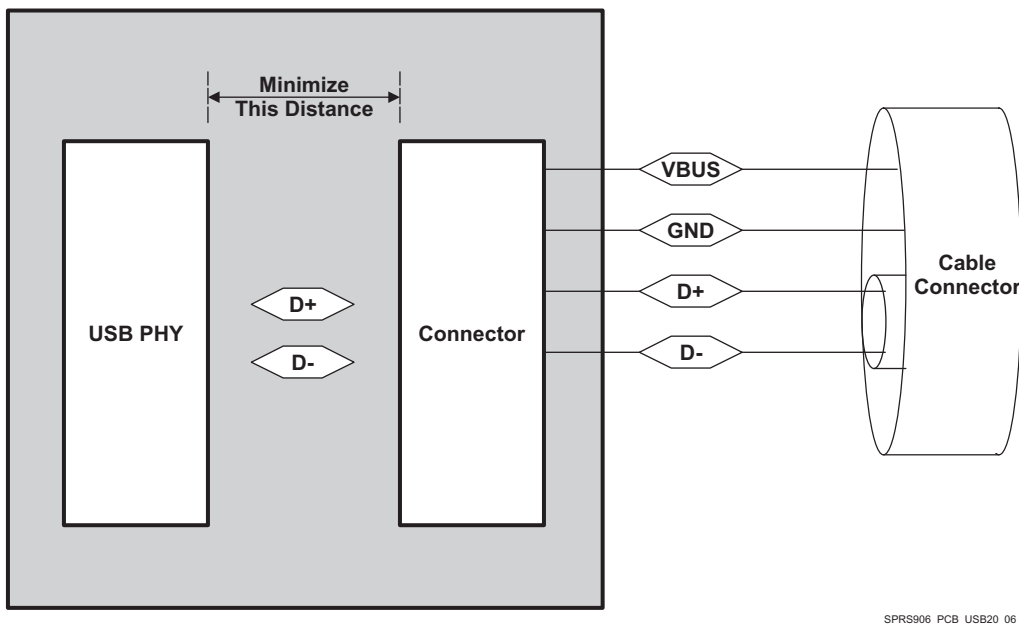
8-26. USB PHY Connector and Cable Connector
