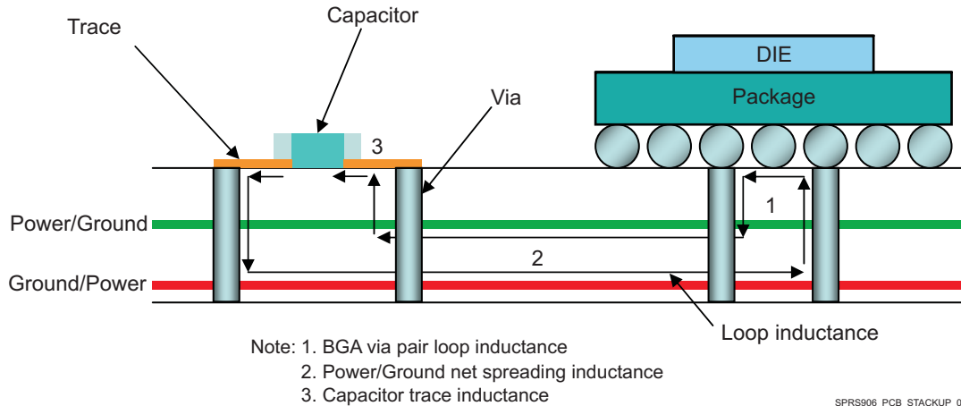
FIG 8-1. Minimize Loop Inductance With Proper Layer Assignment
