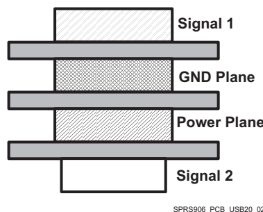
✎ 8-22. Four-Layer Board Stack-Up
