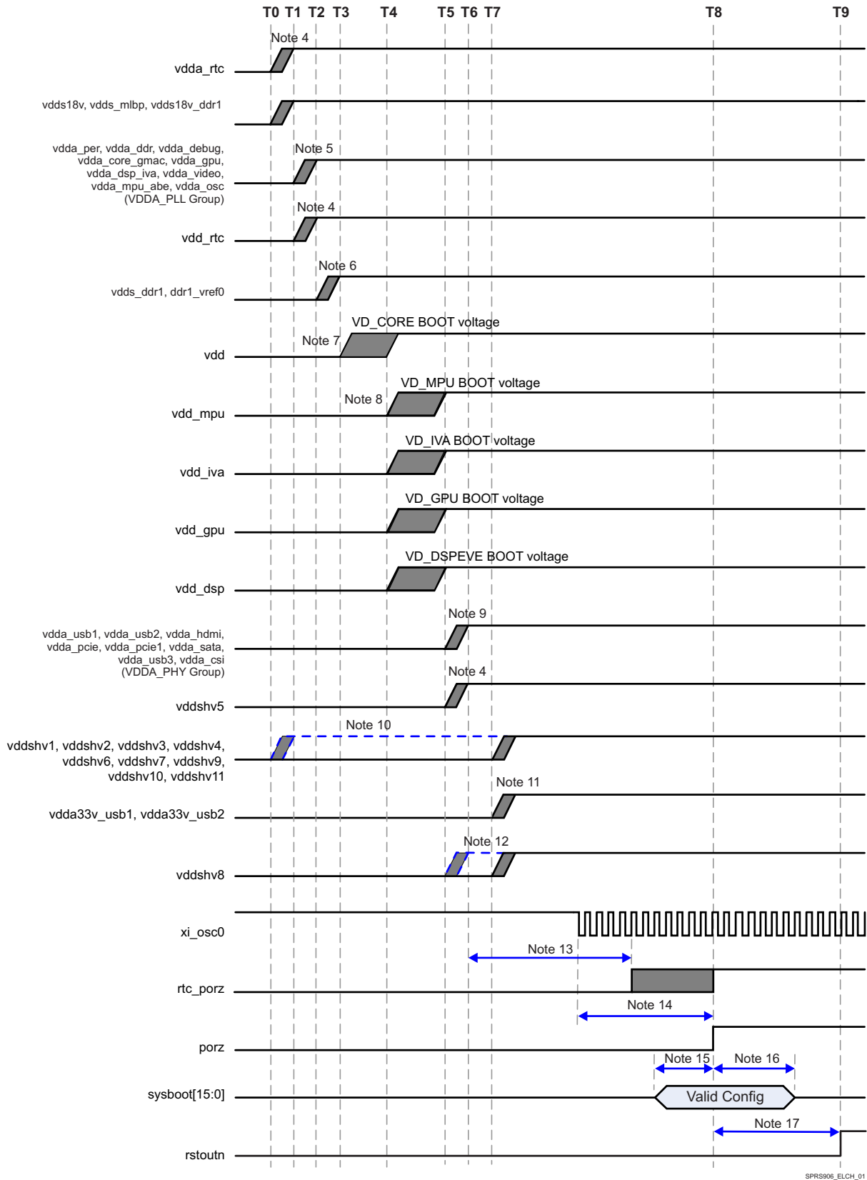
5-2. Recommended Power-Up Sequencing
