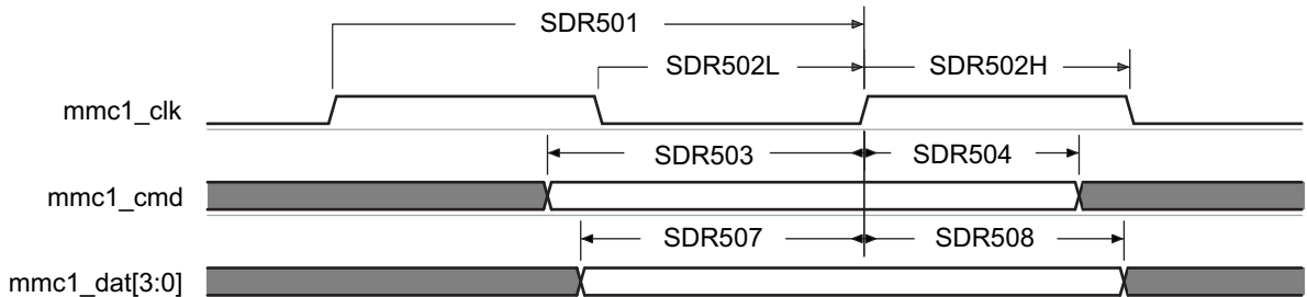
图 7-70. MMC/SD/SDIO in - High Speed SDR50 - Receiver Mode
