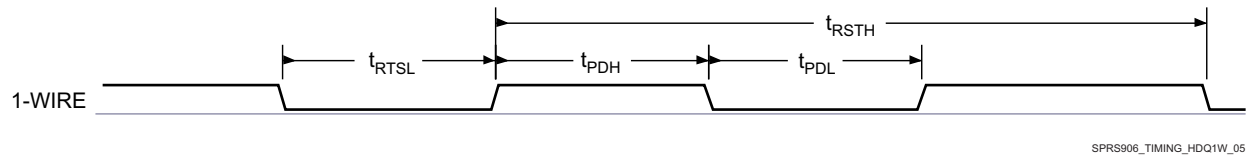
图 7-29. 1-Wire-Break (Reset)
