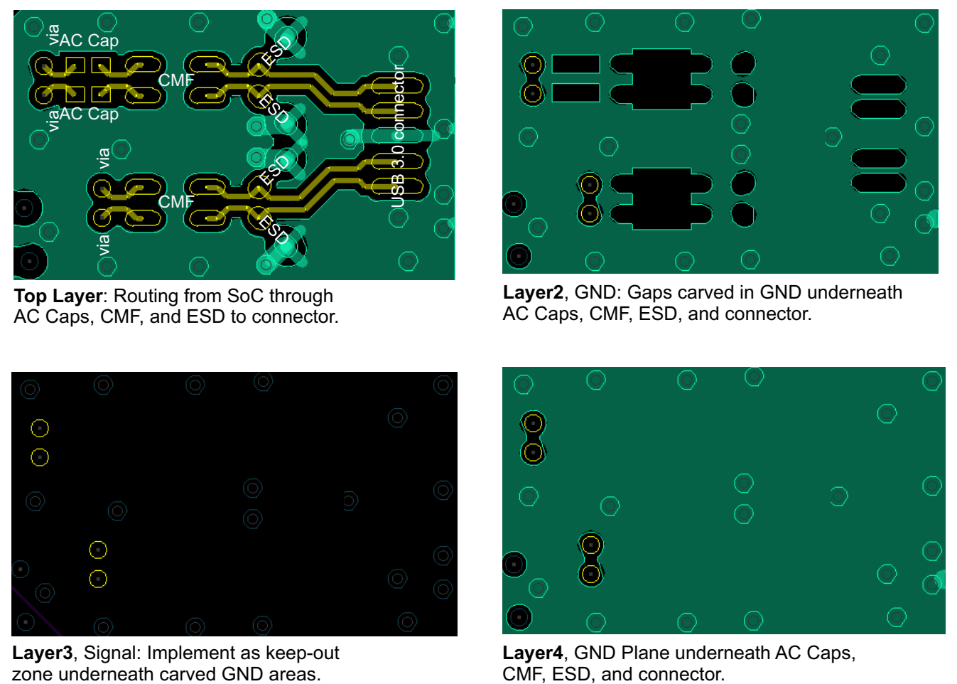
☒ 8-32. USB 3.0 Example “carve GND” layout
