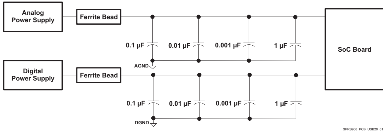
✎ 8-21. Suggested Array Capacitors and a Ferrite Bead to Minimize EMI
