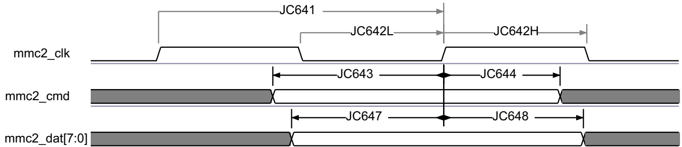
図 7-78. MMC/SD/SDIO in - High Speed JC64 - Receiver Mode
