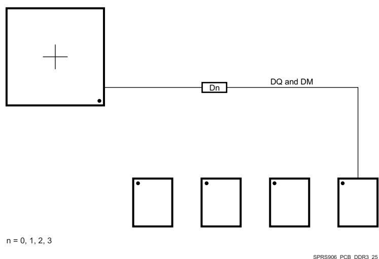
Figure 8-64. DQ/DM Routing With Any Number of Allowed DDR3 Devices
