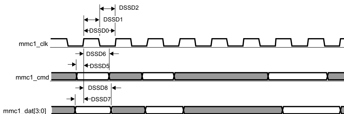
图 7-62. MMC/SD/SDIO in - Default Speed - Receiver Mode
