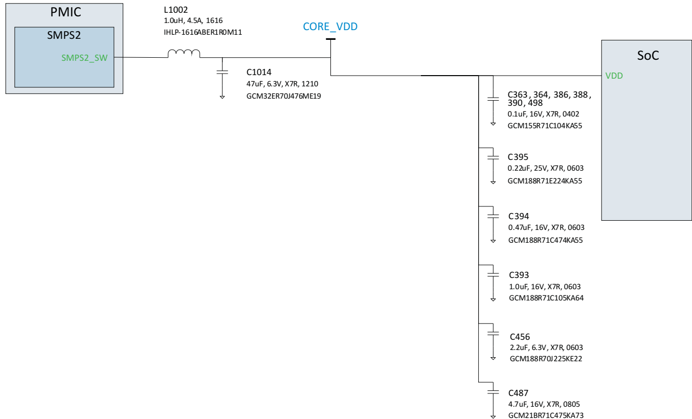
☒ 8-15. vdd Simplified SCH Diagram
