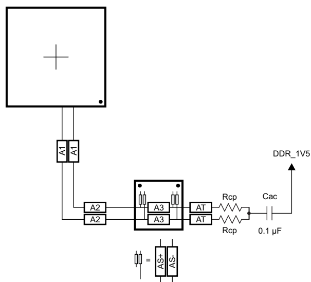
✖ 8-55. CK Routing for Two Mirrored DDR3 Devices
