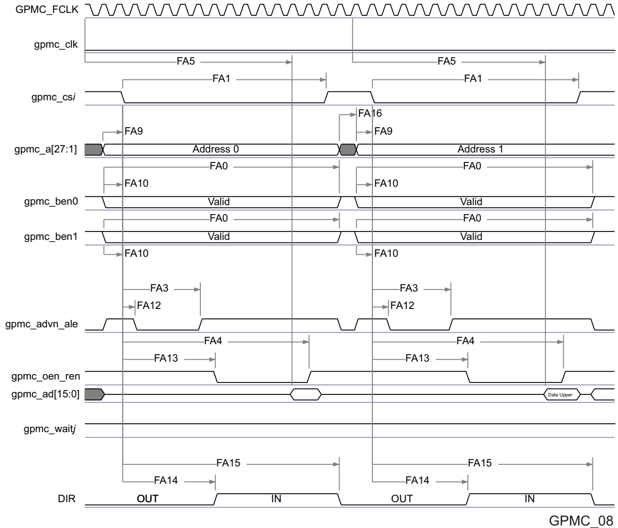
FIG 7-14. GPMC / NOR Flash - Asynchronous Read - 32-bit Timing (1)(2)(3)
