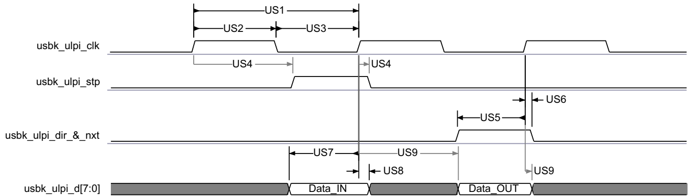
図 7-51. HS USB3 ULPI -SDR-Slave Mode-12-pin Mode
