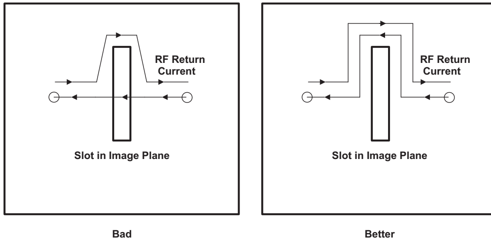
8-29. Do Not Violate Image Planes
