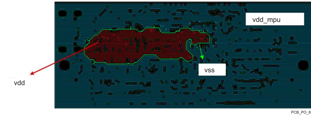
FIG 8-2. Coplanar Shielding of Power Net Using Ground Guard-band
