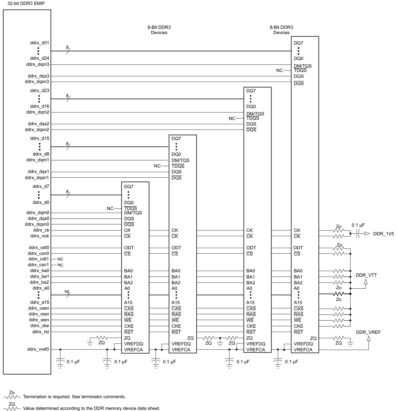
8-42. 32-Bit, One-Bank DDR3 Interface Schematic Using Four 8-Bit DDR3 Devices
