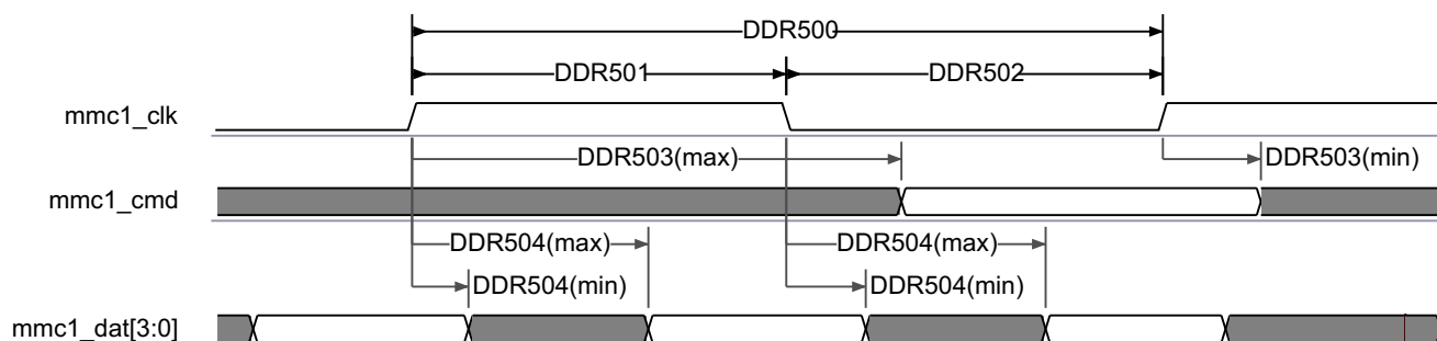
图 7-75. SDRAM - High Speed SD - DDR - Data/Command Transmit
