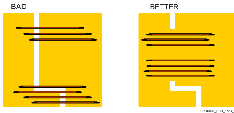
FIG 8-11. Trace Examples
