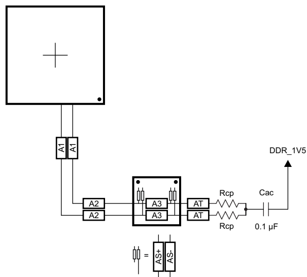
FIG 7-52. CK Routing for Two Mirrored DDR3 Devices
