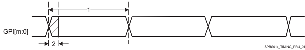
图 5-109. PRU-ICSS PRU Direct Input Timing
