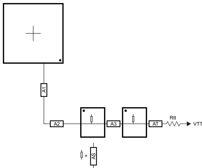
FIG 7-51. ADDR_CTRL Routing for Two Single-Side DDR3 Devices
