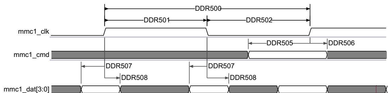
图 5-90. SDMMC - High Speed SD - DDR - Data/Command Receive
