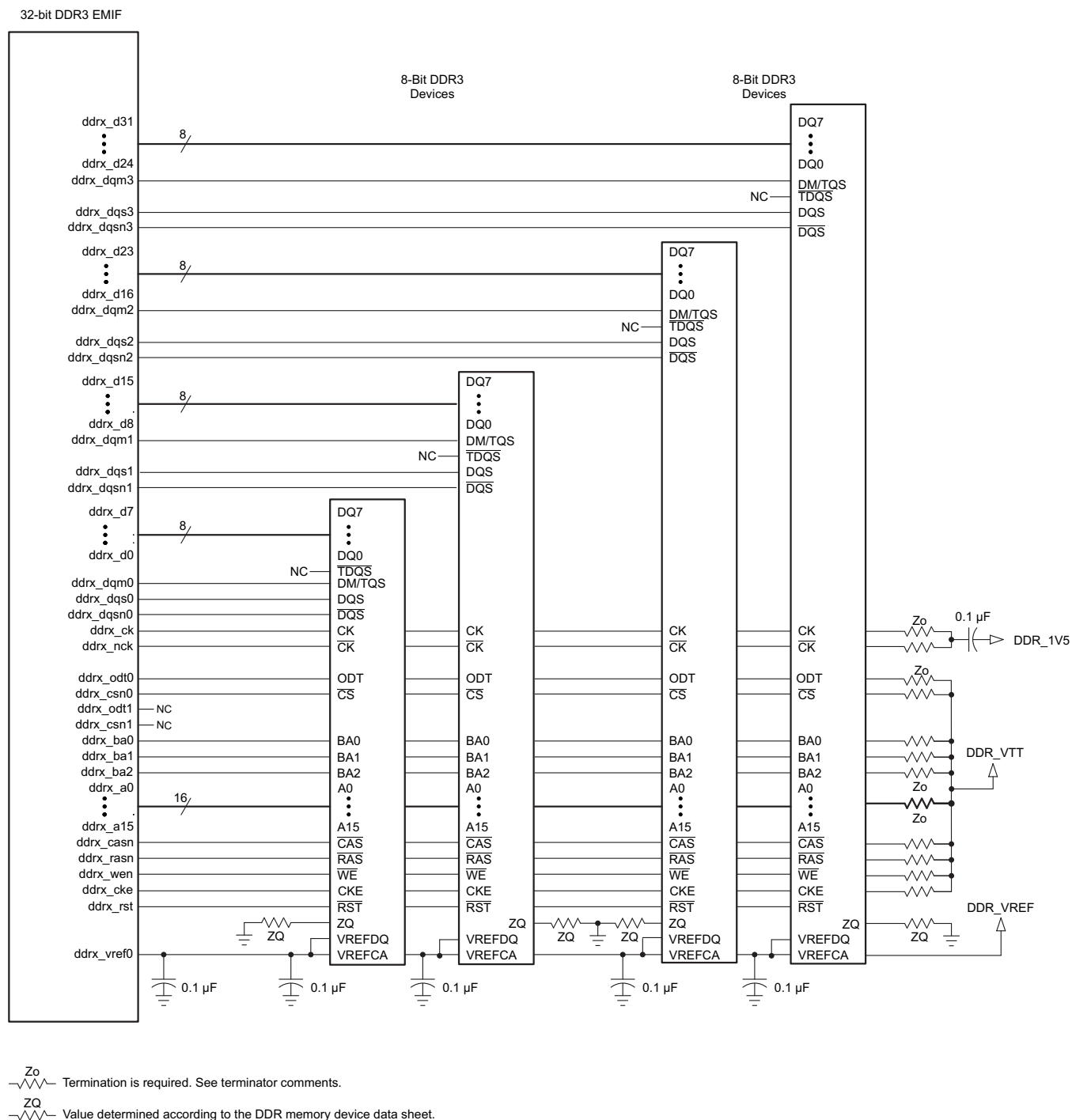
7-39. 32-Bit, One-Bank DDR3 Interface Schematic Using Four 8-Bit DDR3 Devices
