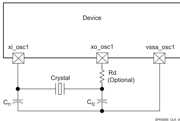
Figure 5-16. Crystal Implementation
