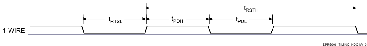
图 5-45. 1-Wire—Break (Reset)
