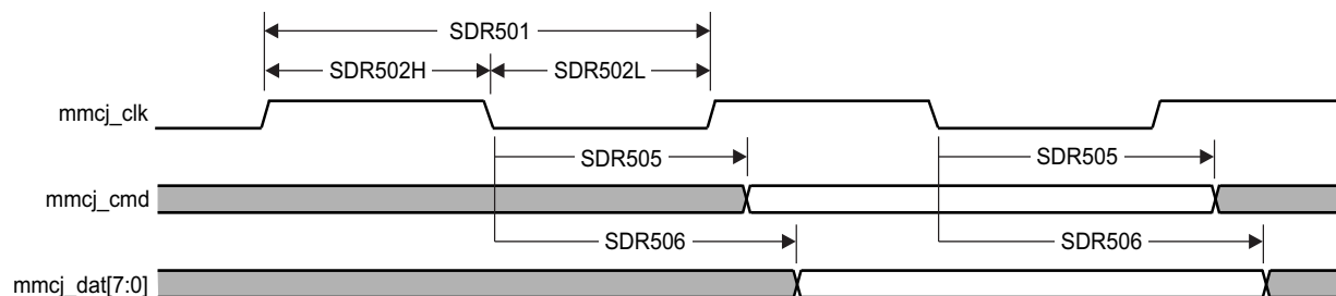
图 5-108. MMC/SD/SDIOj in - High Speed SDR50 - Transmitter Mode
