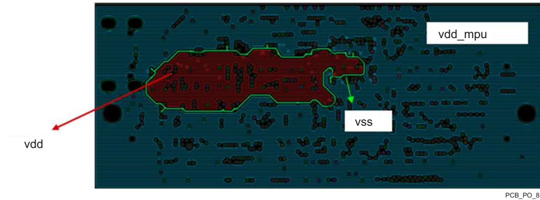
FIG 7-2. Coplanar Shielding of Power Net Using Ground Guard-band
