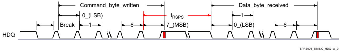
图 5-44. HDQ Communication Timing
