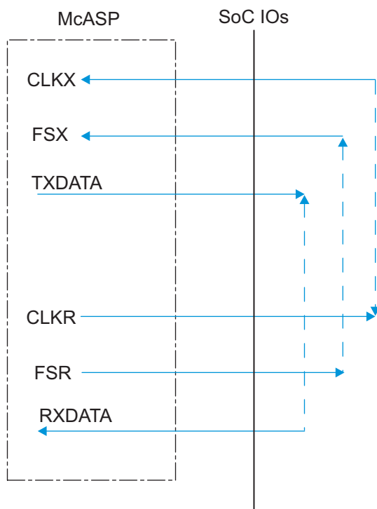
FIG 5-61. McASP1-8 CIOFIO – ASYNC Mode
