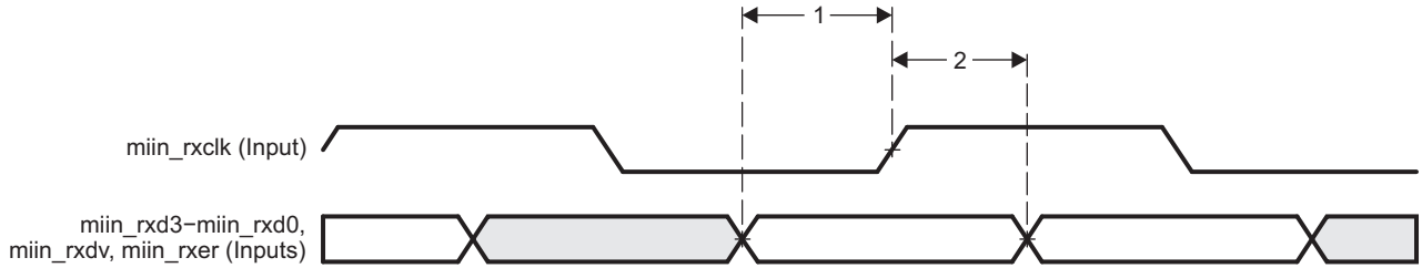
图 5-70. GMAC Receive Interface Timing MIIn operation
