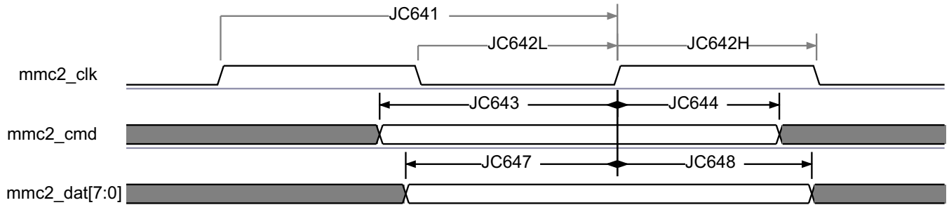
図 5-94. MMC/SD/SDIO in - High Speed JC64 - Receiver Mode
