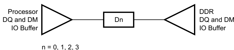
7-59. DQ/DM Topology
