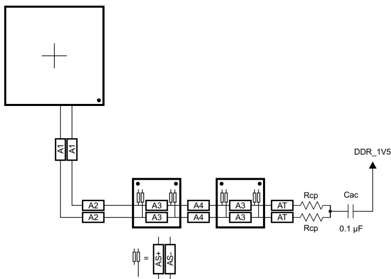
FIG 7-46. CK Routing for Four Mirrored DDR3 Devices
