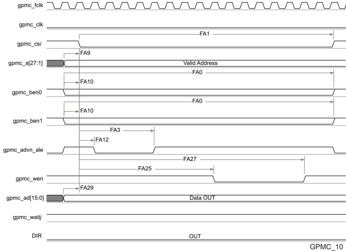
FIG 5-32. GPMC / NOR Flash - Asynchronous Write - Single Word Timing (1)
