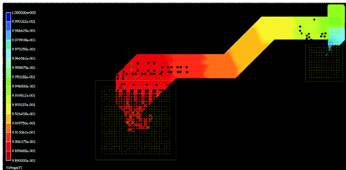
図 7-16. vdd Voltage/IR Drop [All Layers]
