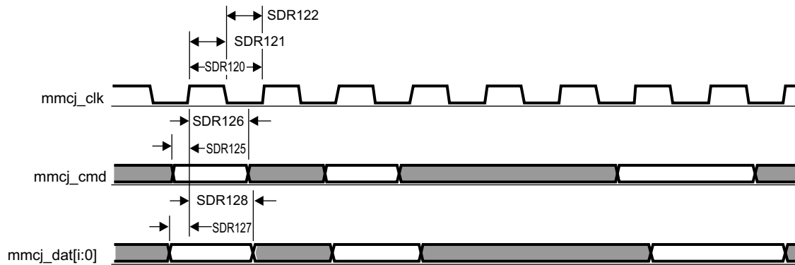
图 5-103. MMC/SD/SDIOj in - SDR12 - Receiver Mode
