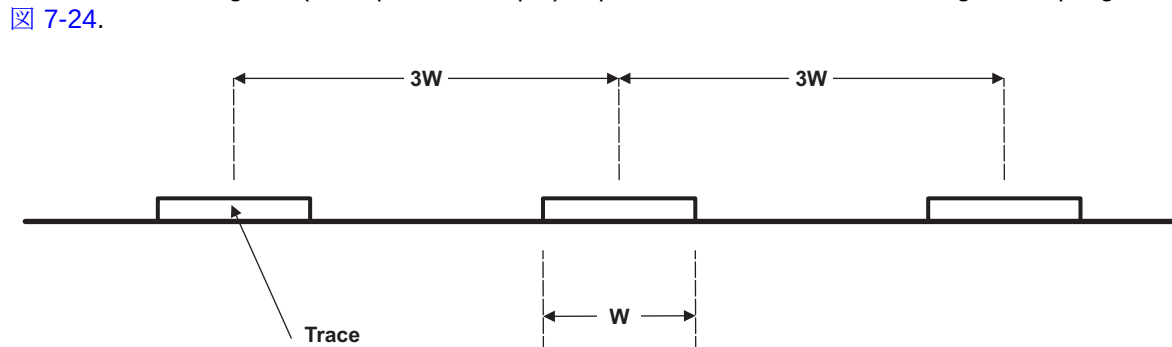
7-24. 3W Spacing Rule
