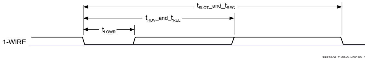
图 5-46. 1-Wire—Read Bit (Data)
