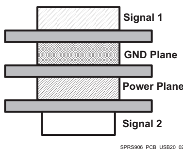
✎ 7-22. Four-Layer Board Stack-Up
