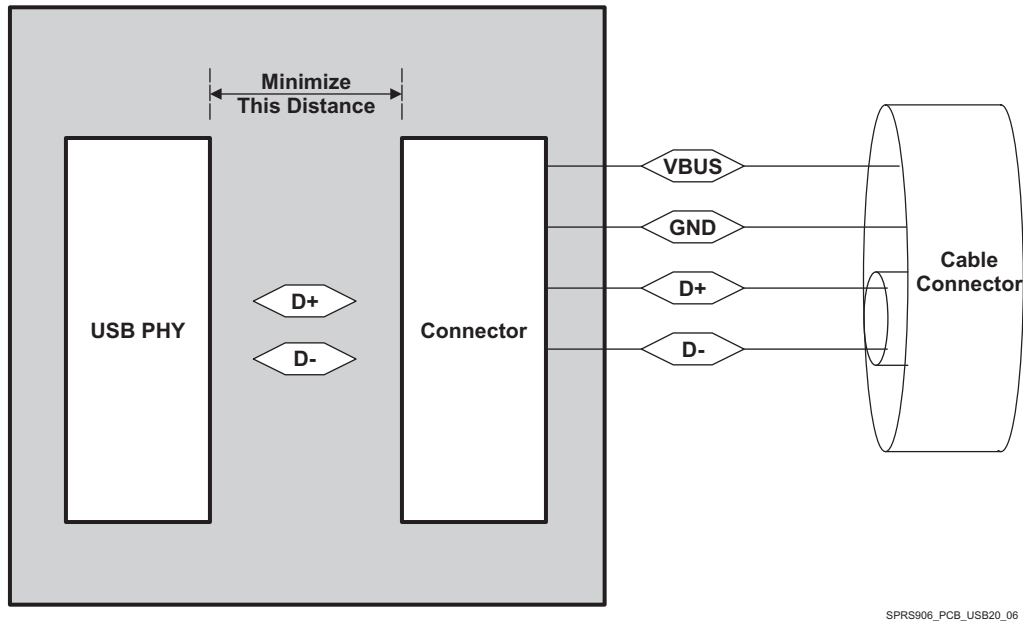
7-26. USB PHY Connector and Cable Connector
