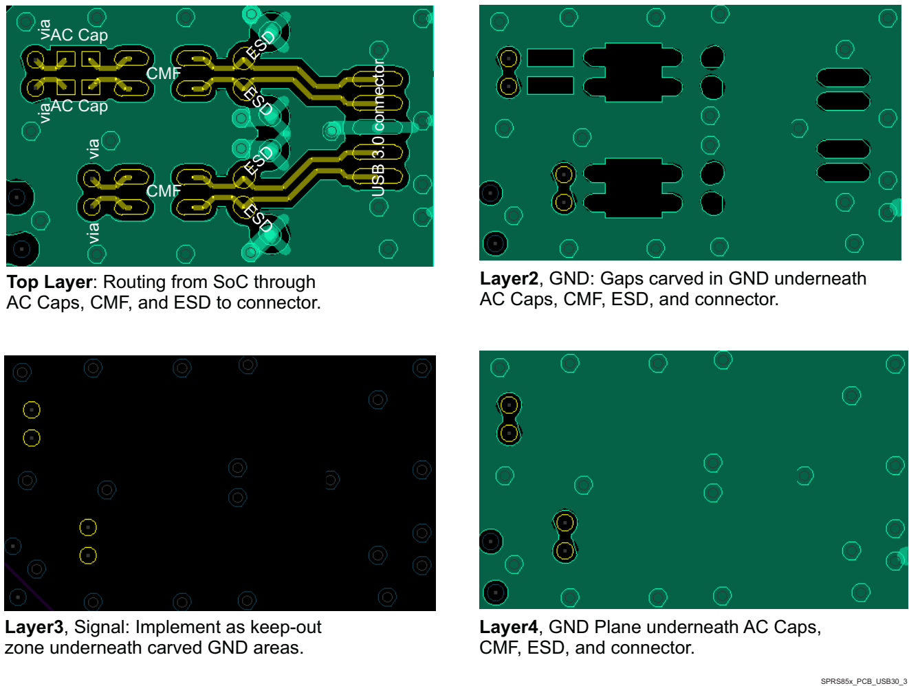
图 7-32. USB 3.0 Example “carve GND” layout
