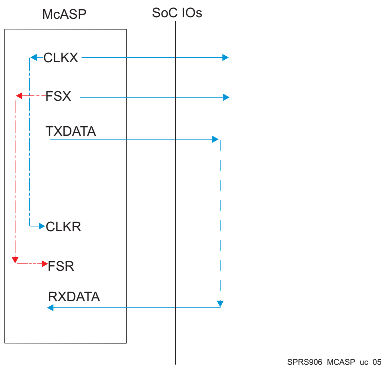
图 5-63. McASP1-8 CO-FO- – SYNC Mode
