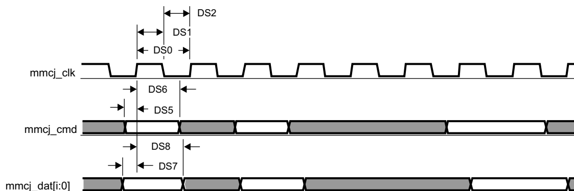
图 5-99. MMC/SD/SDIOj in - Default Speed - Receiver Mode
