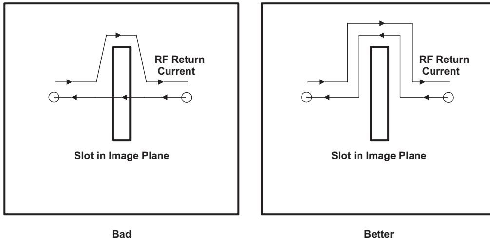
7-29. Do Not Violate Image Planes
