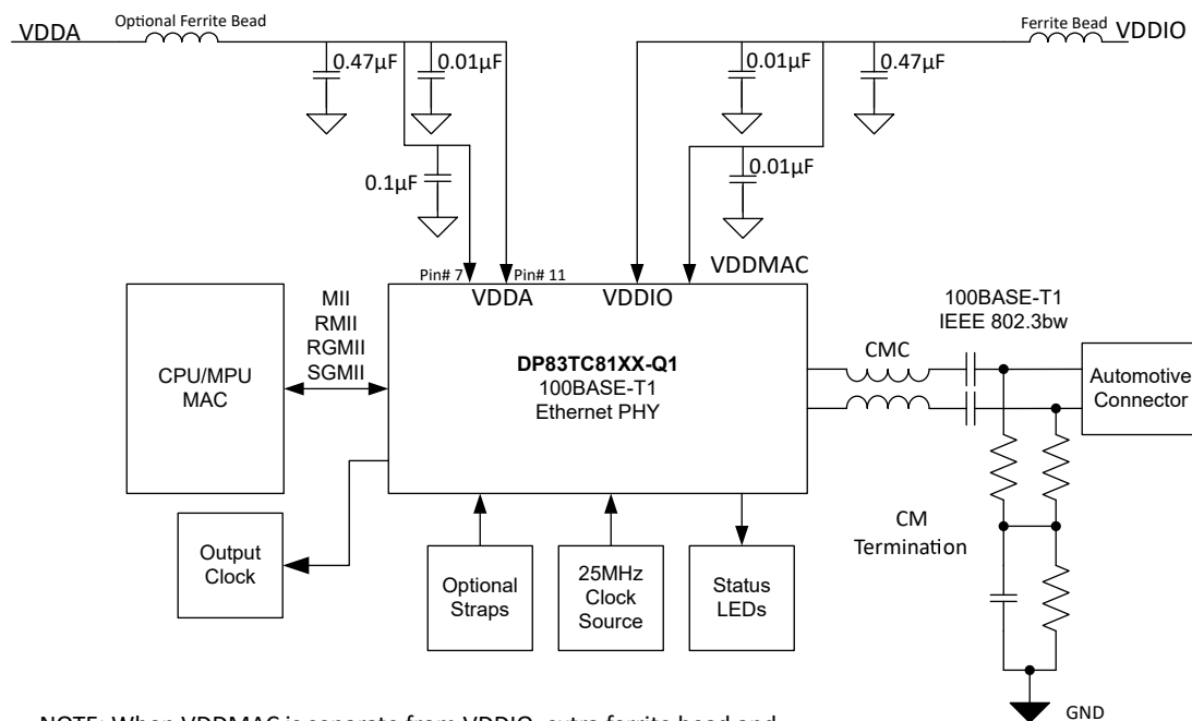
10-1. Typical Application With Peripherals
