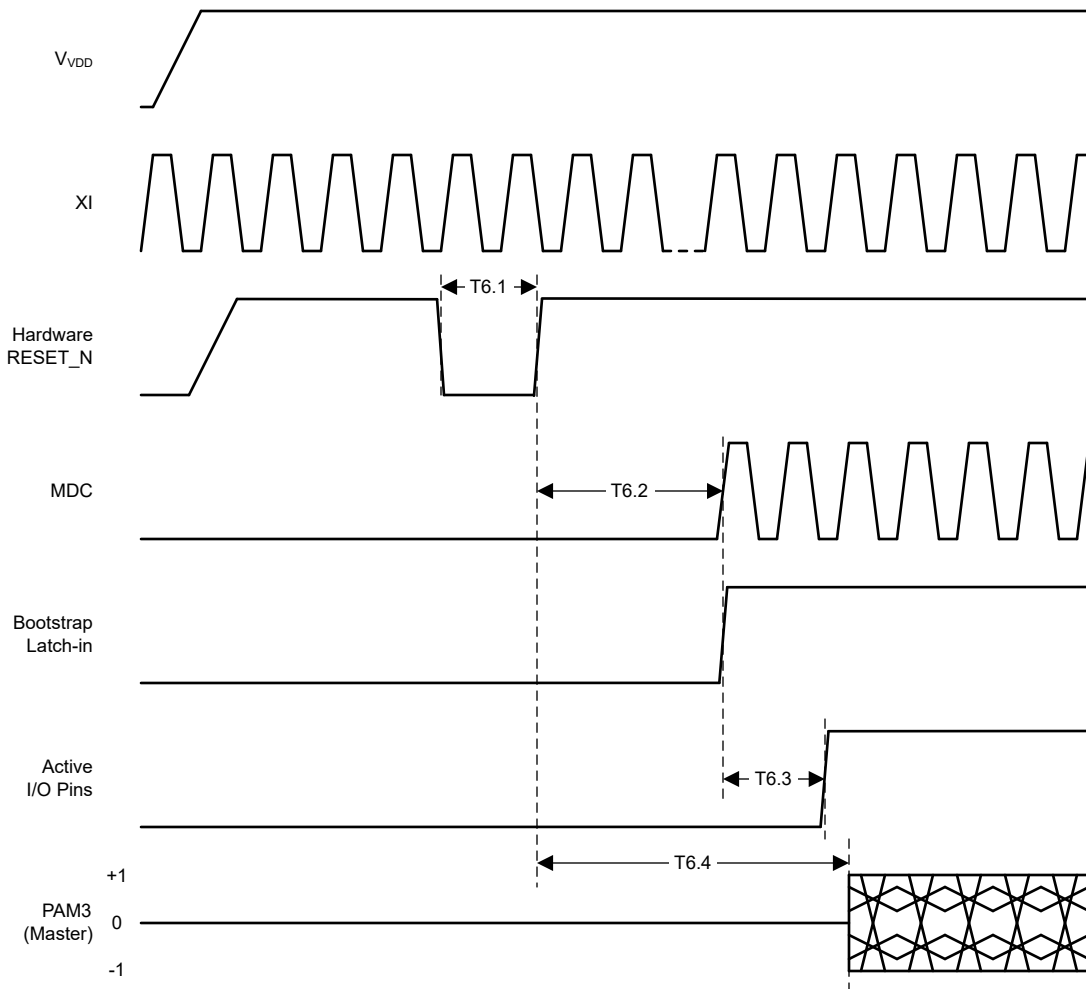
7-9. Reset Timing
