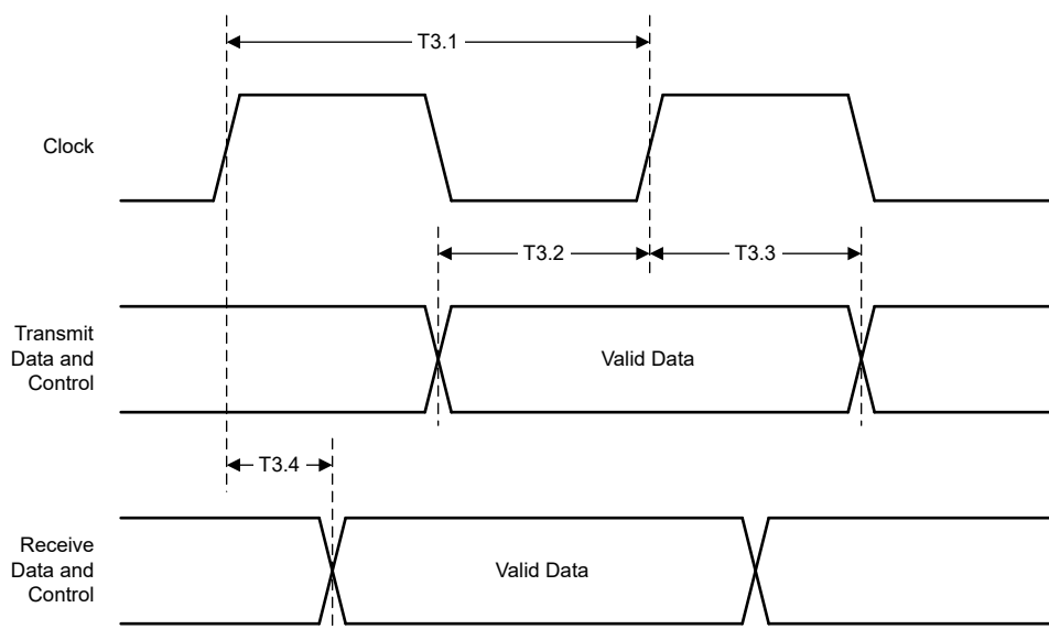
Fig 7-2. RMII Transmit and Receive Timing
