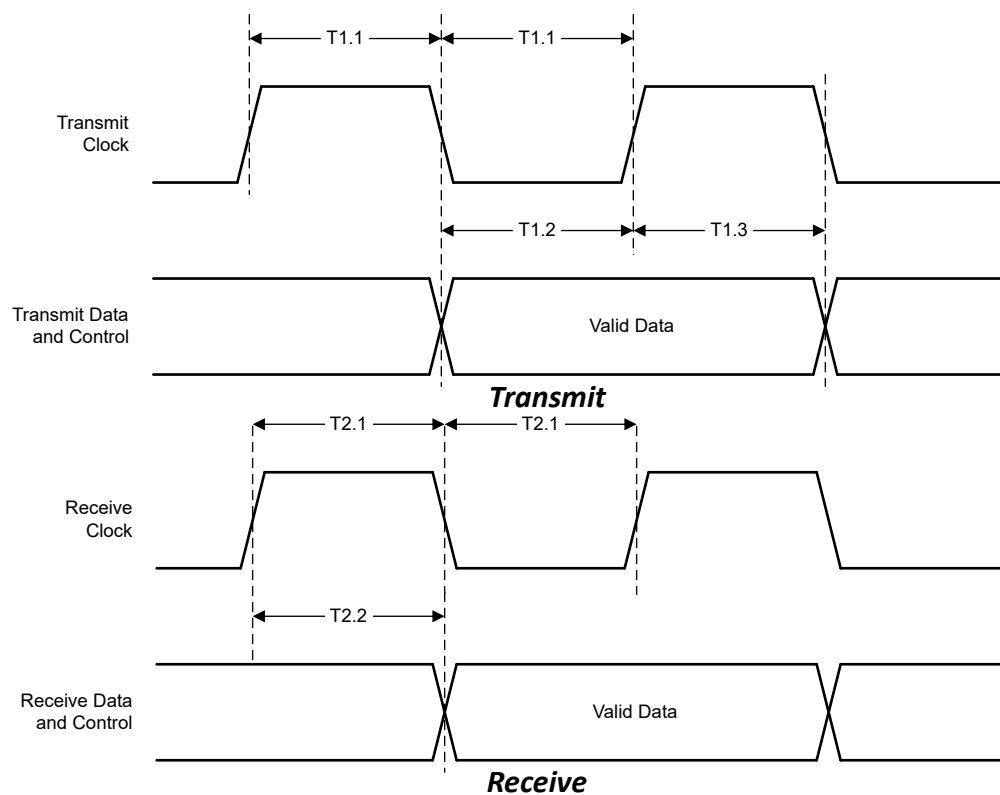
Fig 7-1. MII Timing
