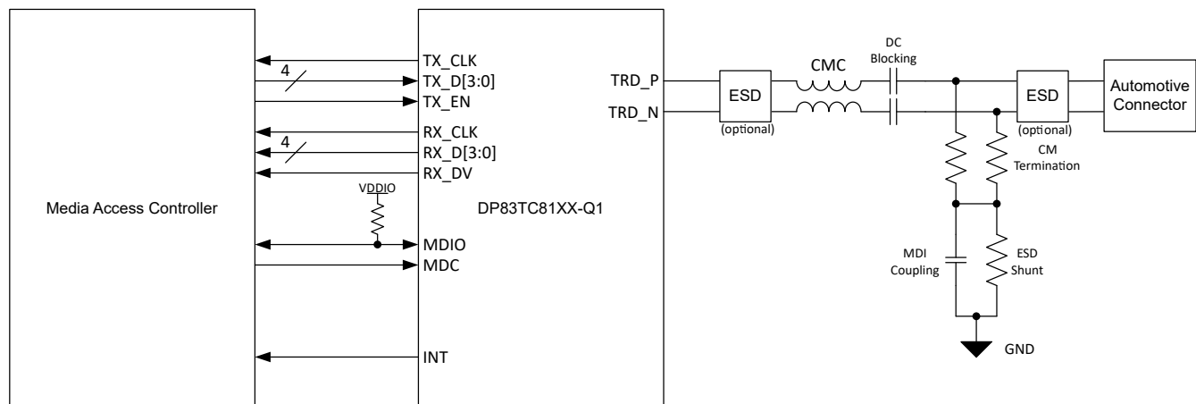
図 9-1. Typical Application (MII)
