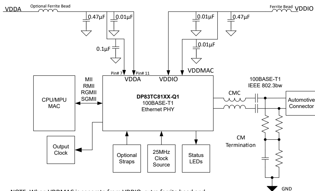
10-1. Typical Application With Peripherals
