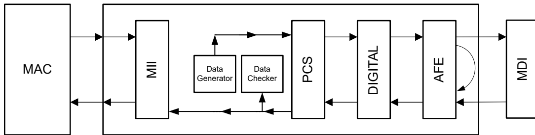
FIG 8-7. Analog loopback with data generator
