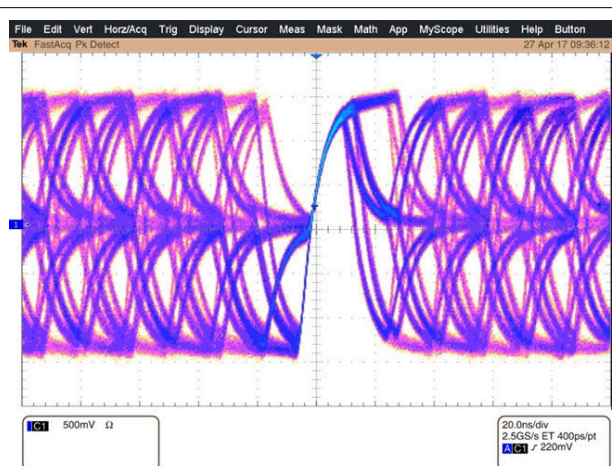
9-7. MDI IDLE Stream (Variable Persistence)
