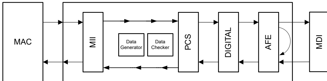
FIG 8-8. Analog loopback without data generator
