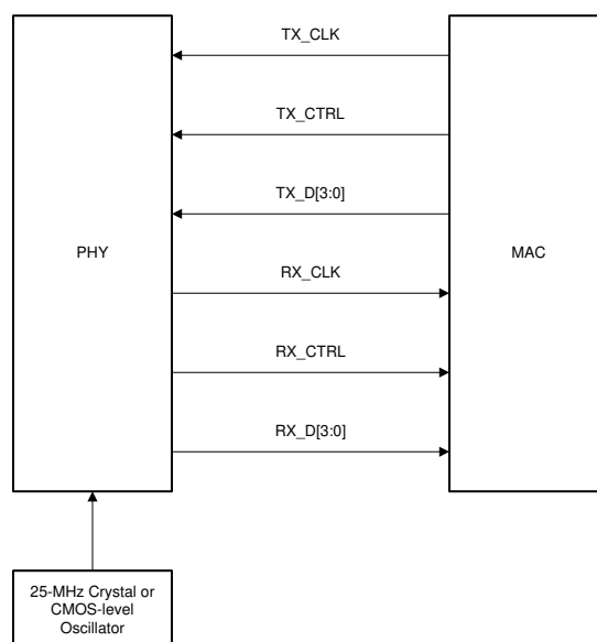
図 7-16. RGMI Connections
