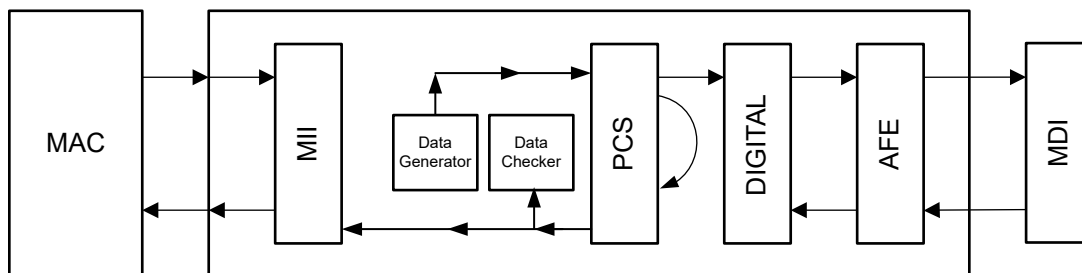
図 7-3. PCS Loopback with data generator
