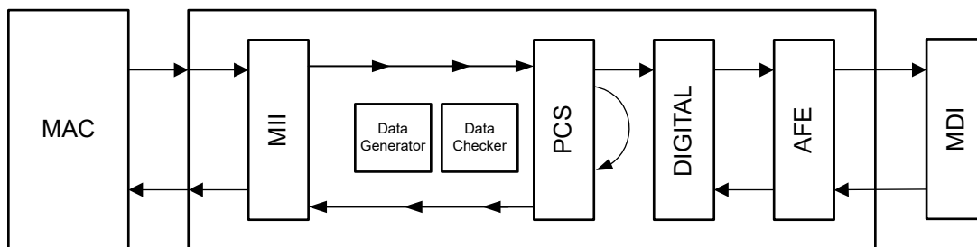
図 7-4. PCS Loopback without data generator
