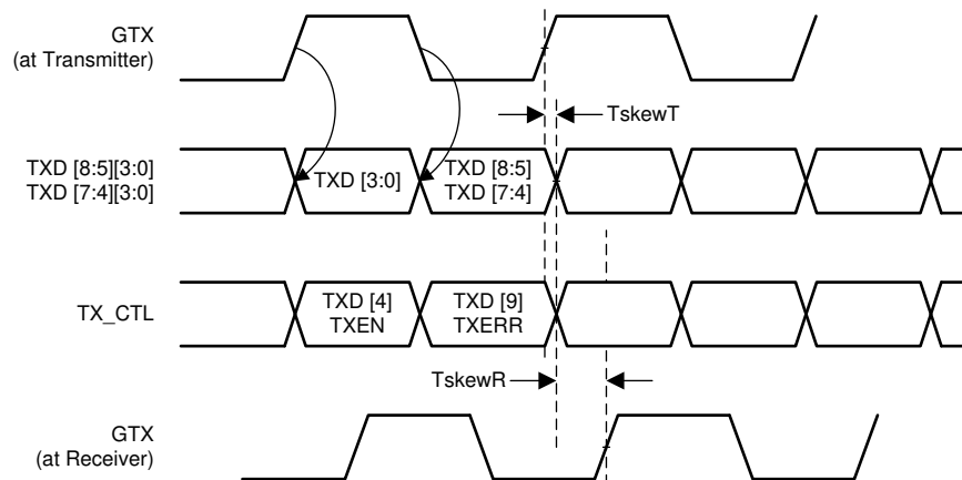
図 6-6. RGMII Transmit Multiplexing and Timing Diagram
