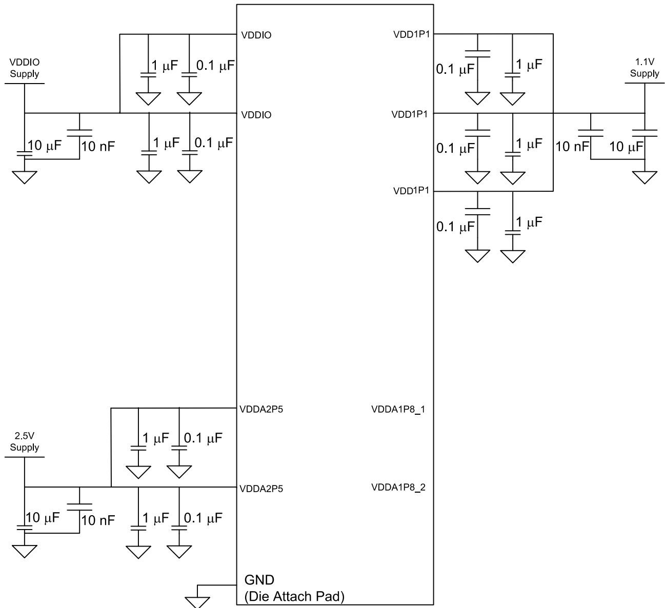
図 8-8. Two-Supply Configuration
