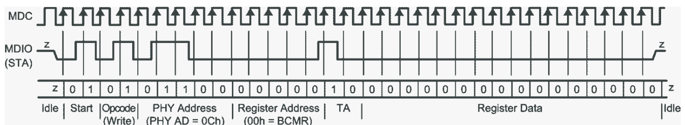
7-14. Typical MDC/MDIO Write Operation
