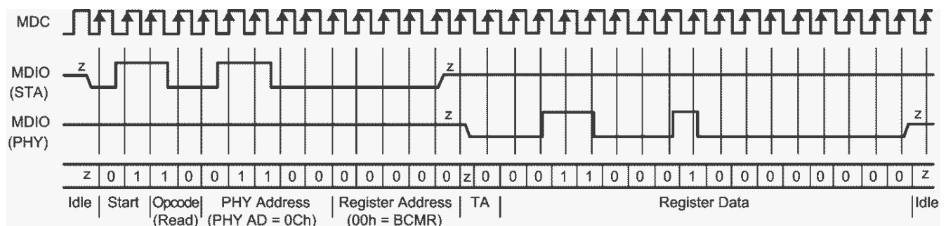
7-13. Typical MDC/MDIO Read Operation
