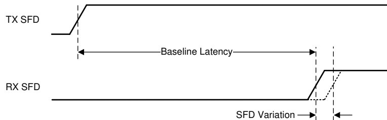
FIG 7-3. Baseline Latency and SFD Variation in Latency Measurement
