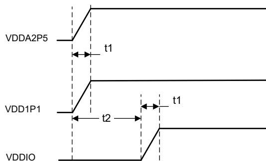
図 8-9. Two-Supply Sequence Diagram
