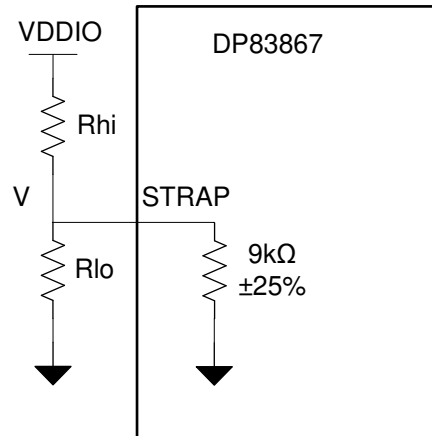
図 7-12. Strap Circuit
