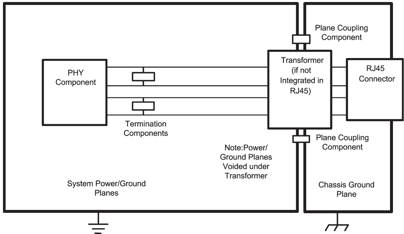
Figure 8-5. Layout Example
