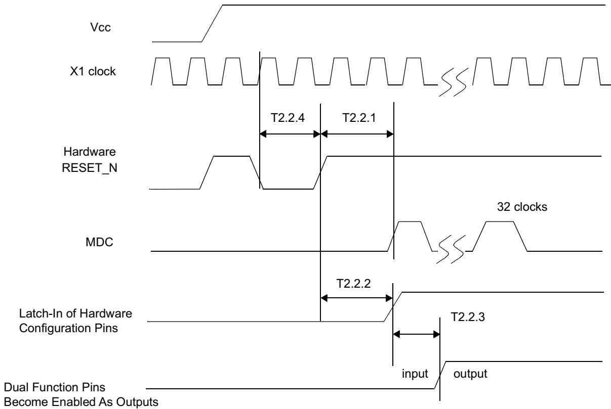
Figure 5-2. Reset Timing
