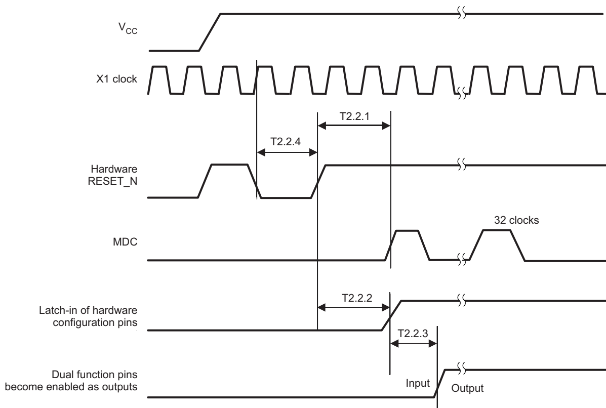
FIG 4-3. Reset Timing
