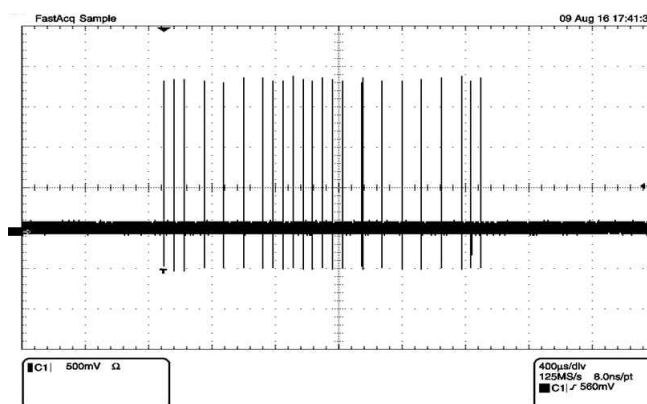
6-11. Auto-Negotiation FLP
