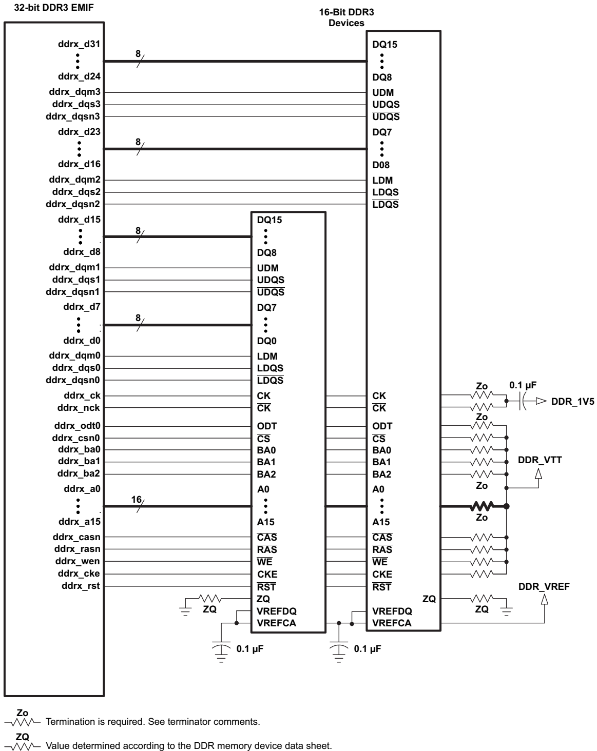
7-46. 32-Bit, One-Bank DDR3 Interface Schematic Using Two 16-Bit DDR3 Devices
