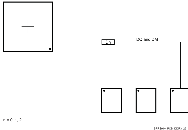
7-68. DQ/DM Routing With Any Number of Allowed DDR3 Devices
