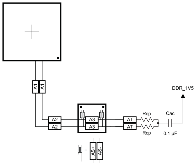
7-53. CK Routing for Two Mirrored DDR3 Devices
