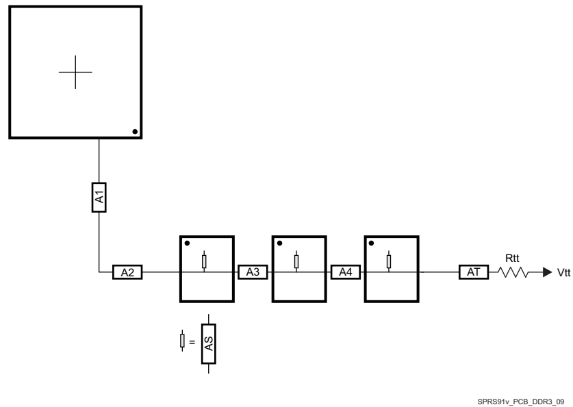
7-52. ADDR_CTRL Routing for Three Single-Side DDR3 Devices
