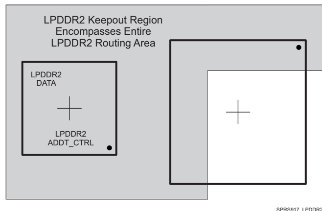
☒ 7-26. LPDDR2 Keepout Region
