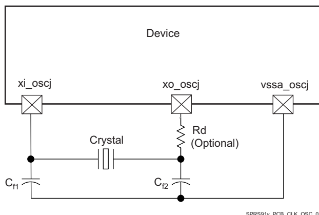
图 7-22. Grounding Scheme for High-Frequency Clock
