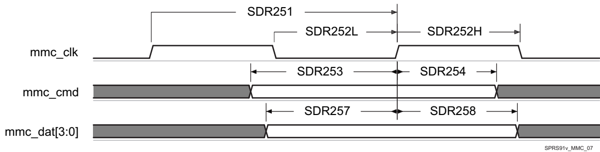
図 5-60. MMC/SD/SDIOj in - SDR25 - Receiver Mode
