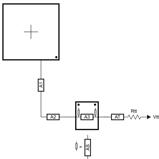
7-54. ADDR_CTRL Routing for Two Mirrored DDR3 Devices
