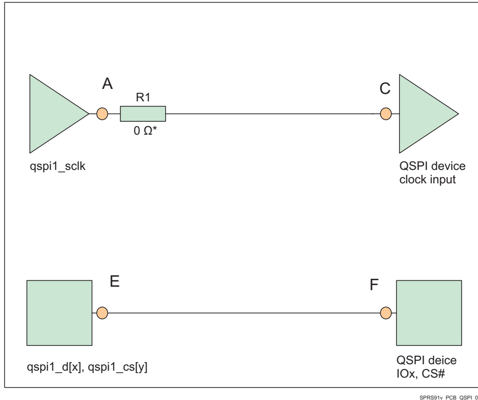
図 7-20. QSPI Interface High Level Schematic Mode 3 (POL=1, PHA=1)
