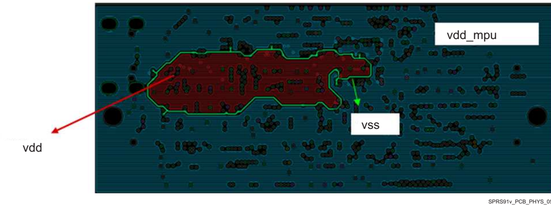
✎ 7-2. Coplanar Shielding of Power Net Using Ground Guard-band
