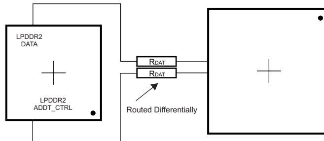
7-28. DQ[x] Topology
