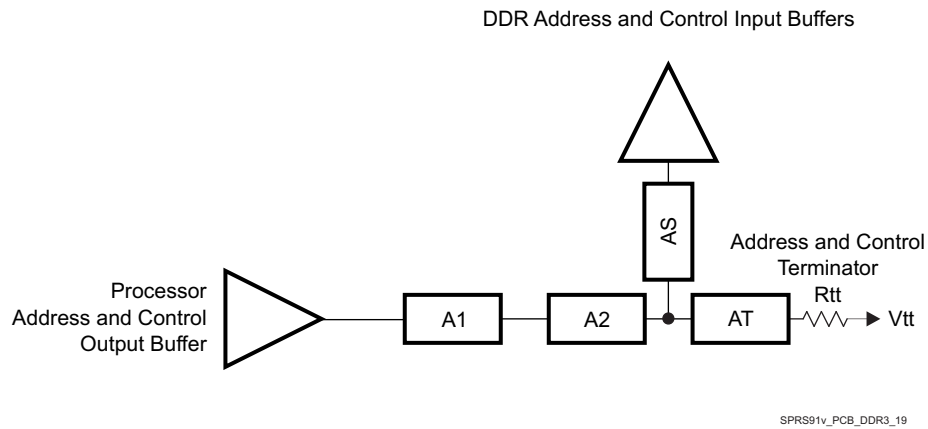
7-62. ADDR_CTRL Topology for One DDR3 Device
