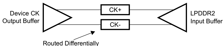
7-32. CK Signals Topology
