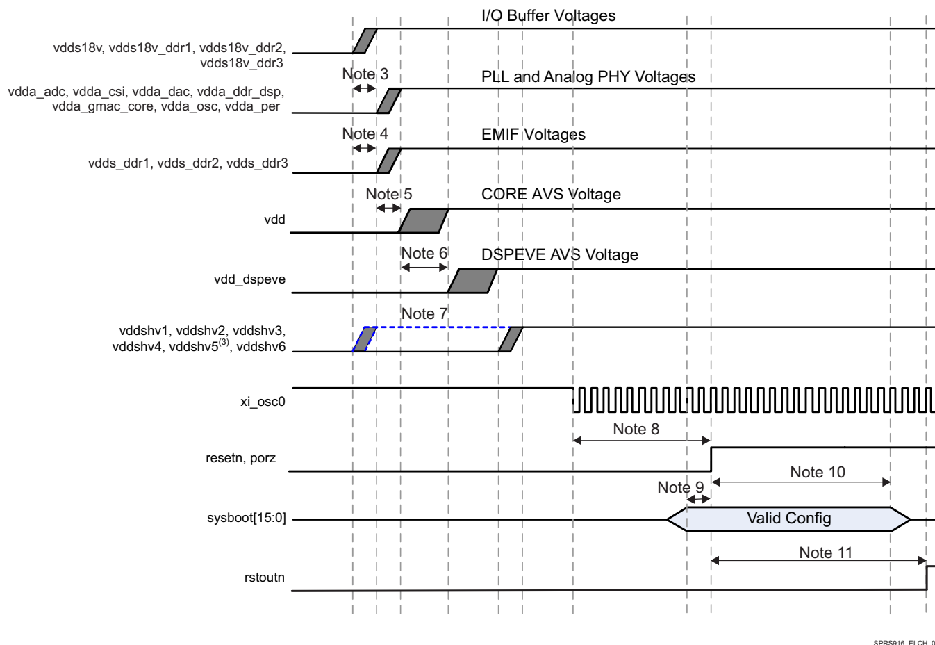
Figure 5-4. Power-Up Sequencing
