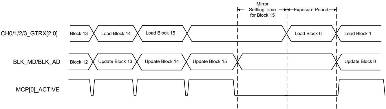
図 6-5. Single Block Load Phased Sequence
