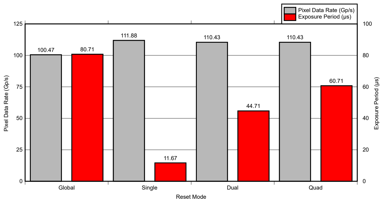
図 7-2. DLP991U DMD Performance Plot at 3.6Gbps Data Rate
