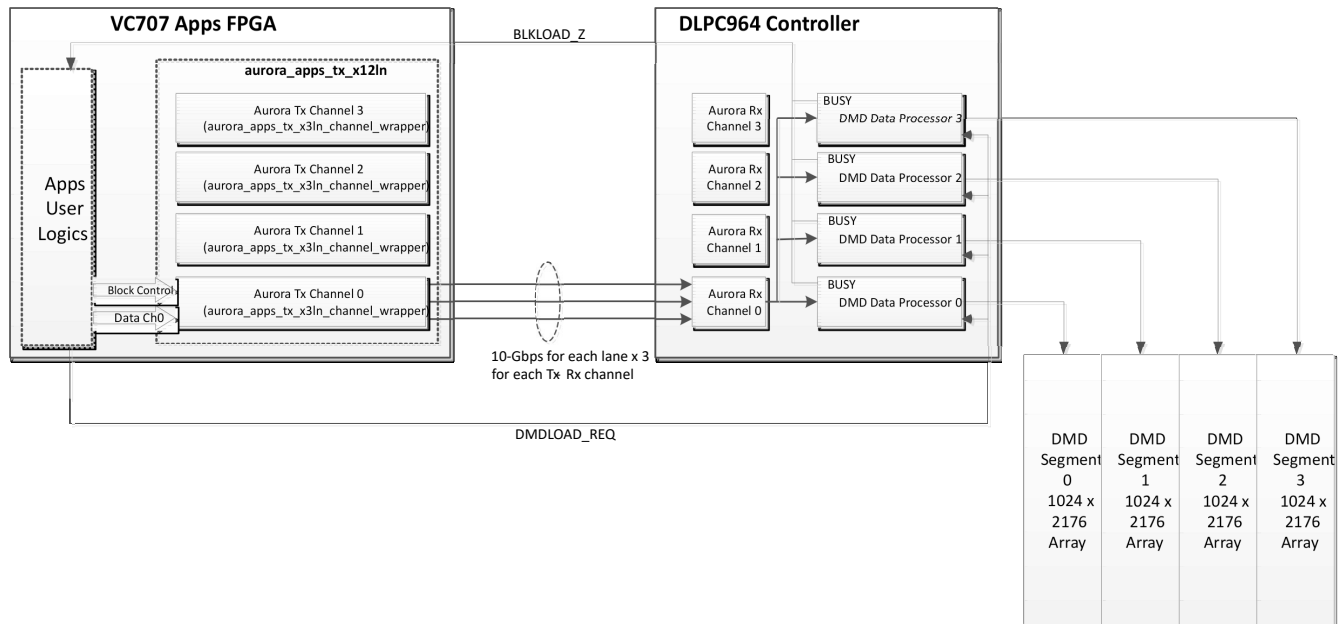
図 7-9. System Block Diagram for Single Channel Transfer Mode
