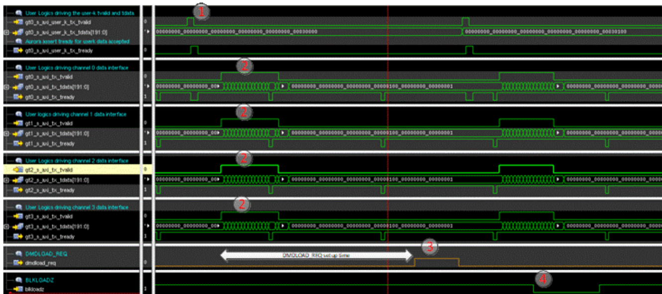
図 7-7. Example of DMDLOAD_REQ Setup Time for Three DMD Row Load Operation
