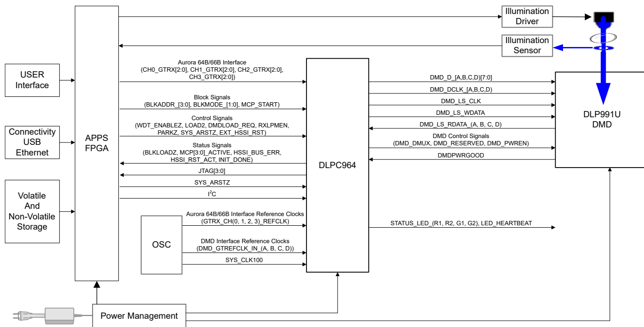
図 7-1. Typical DLP991U High Speed Application
