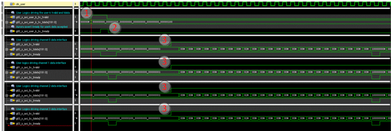
図 7-4. Block Start with Block Control Word Waveform
