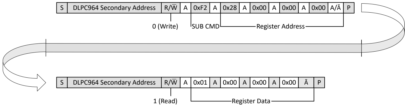
図 6-3. Example I 2 C Primary Reading DLPC964 Register Data
