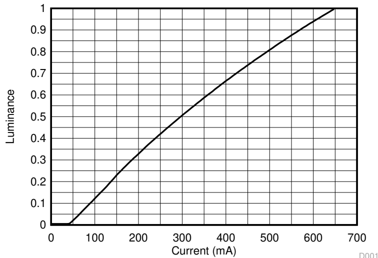
Figure 8-2. Typical Luminescence vs Current
