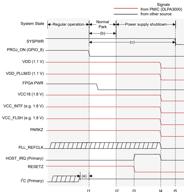
9-2. DLPC3437 Normal Power-Down
