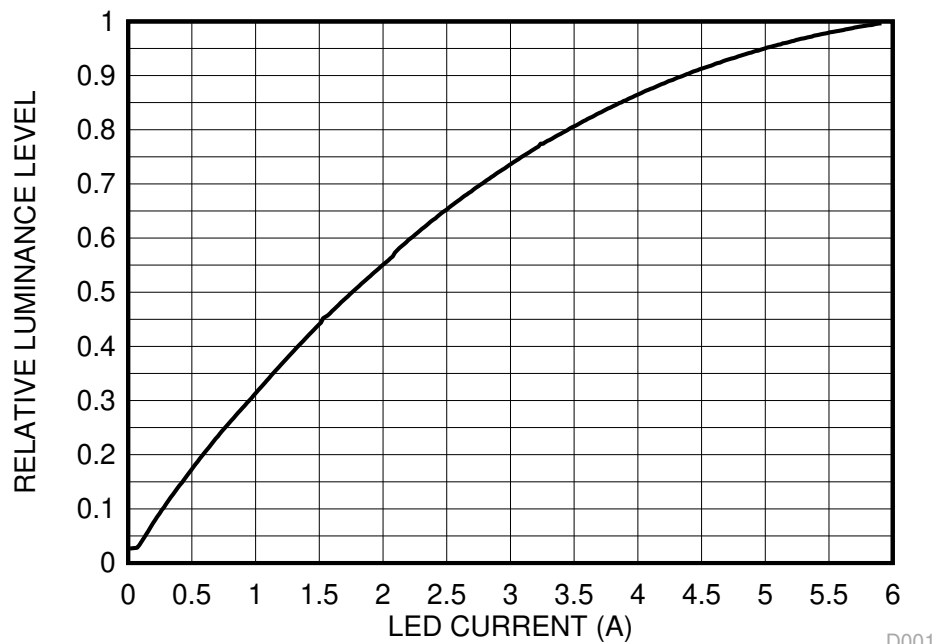
8-2. Typical Luminance vs Current
