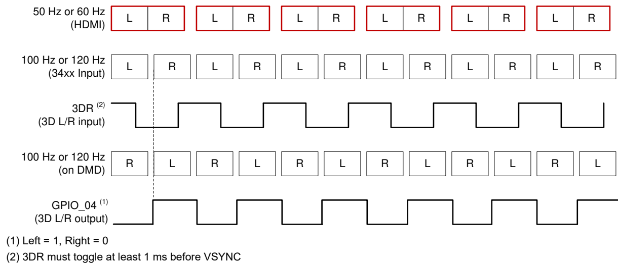
FIG 7-1. 3D Display Left and Right Frame Timing
