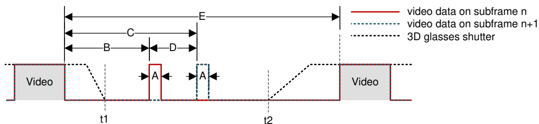
図 6-10. 3D DLP Link Pulse Timing
