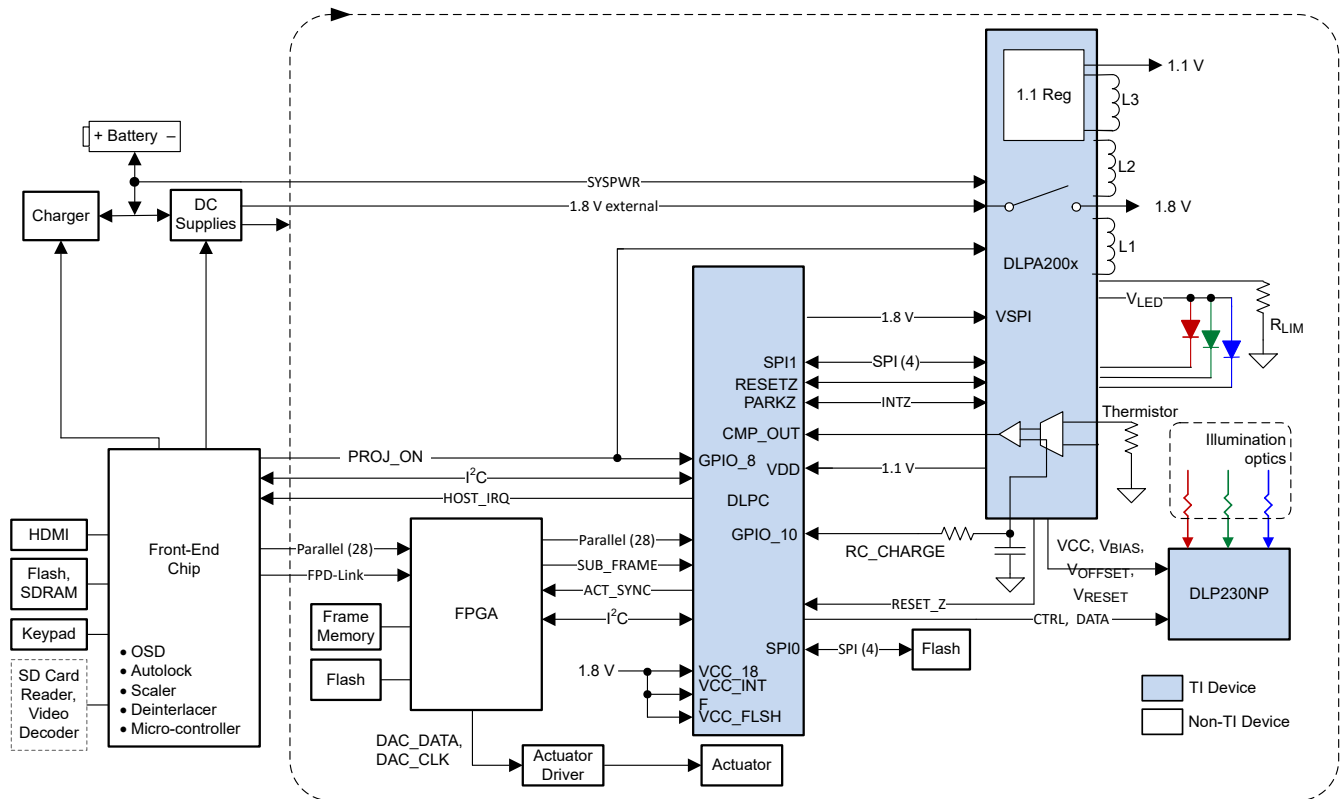
☒ 7-1. Typical Application Diagram (using DLPA200x)
