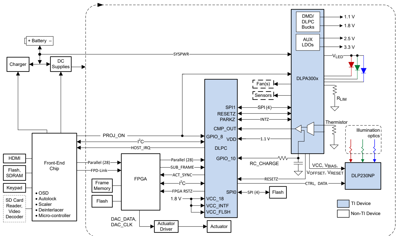
7-2. Typical Application Diagram (using DLPA300x)
