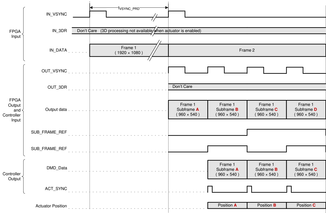
図 6-1. 2D Actuator Frame and Signal Timing
