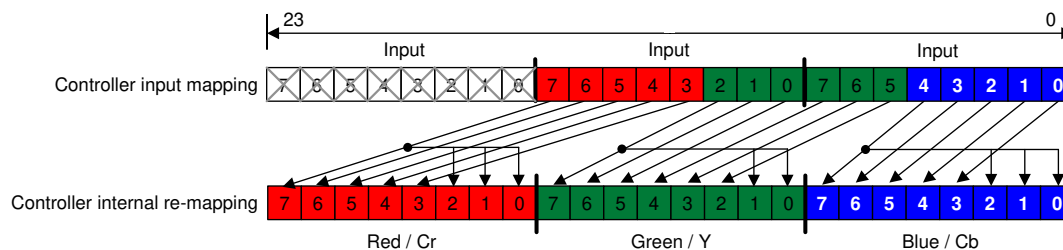
FIG 7-4. RGB-565 and YCbCr-565 I/O Mapping
