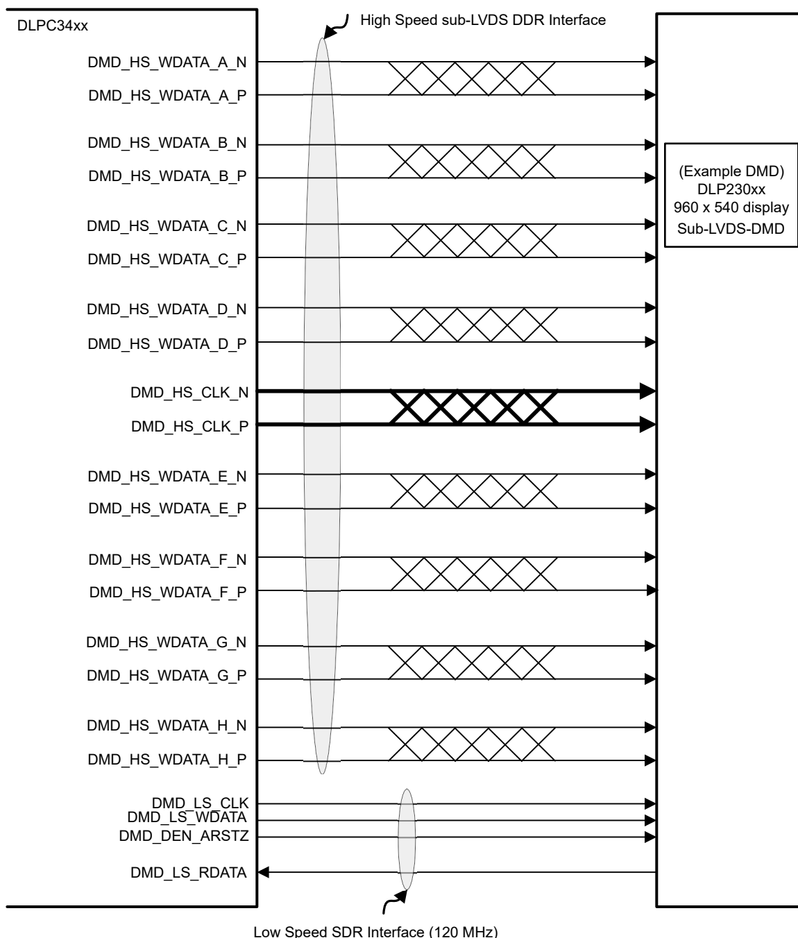
FIG 7-16. DLP230GP (.23 qHD) DMD Interface Example
