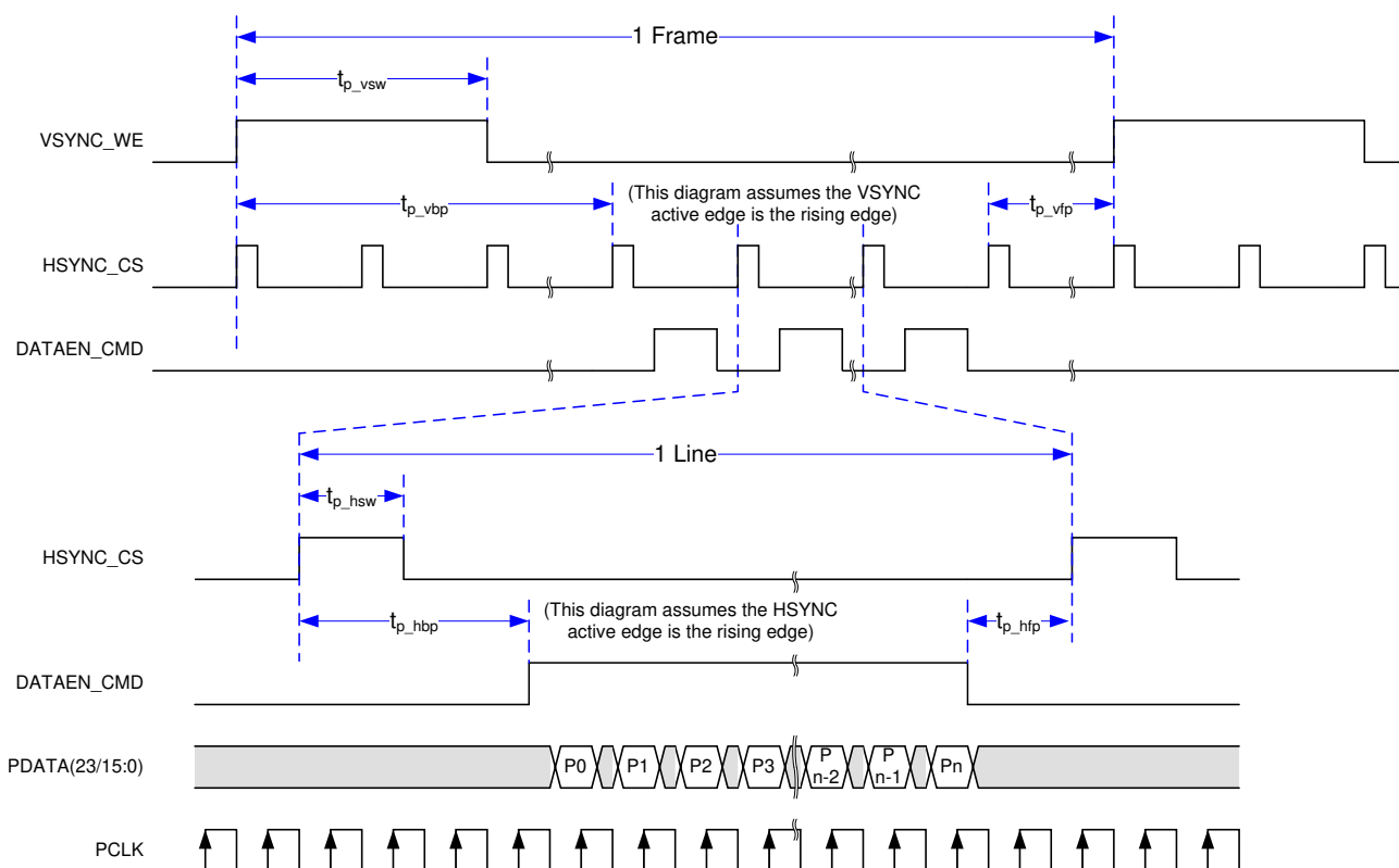
6-7. Parallel Interface Frame Timing
