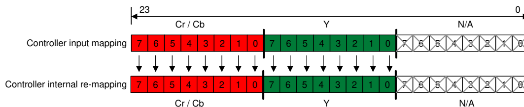
FIG 7-5. 16-Bit YCbCr-880 I/O Mapping
