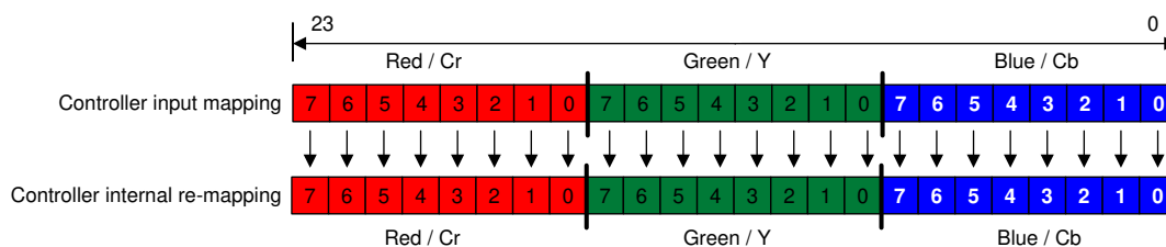
FIG 7-2. RGB-888 and YCbCr-888 I/O Mapping
