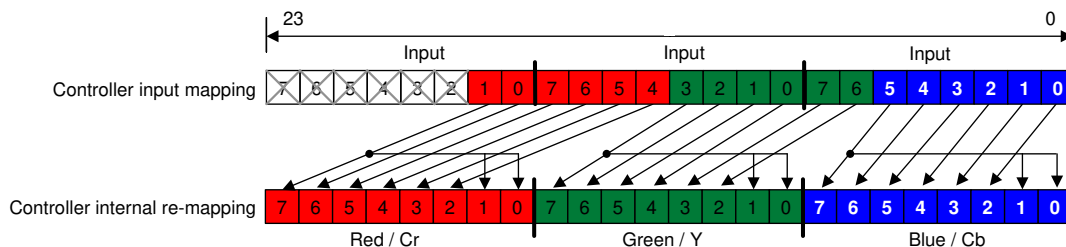
FIG 7-3. RGB-666 and YCbCr-666 I/O Mapping
