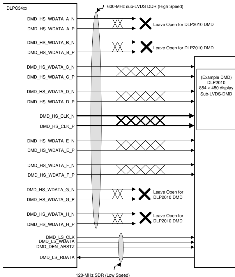
図 7-16. DLP2010 (.2 WVGA) DMD Interface Example (Option 1 and 2)
