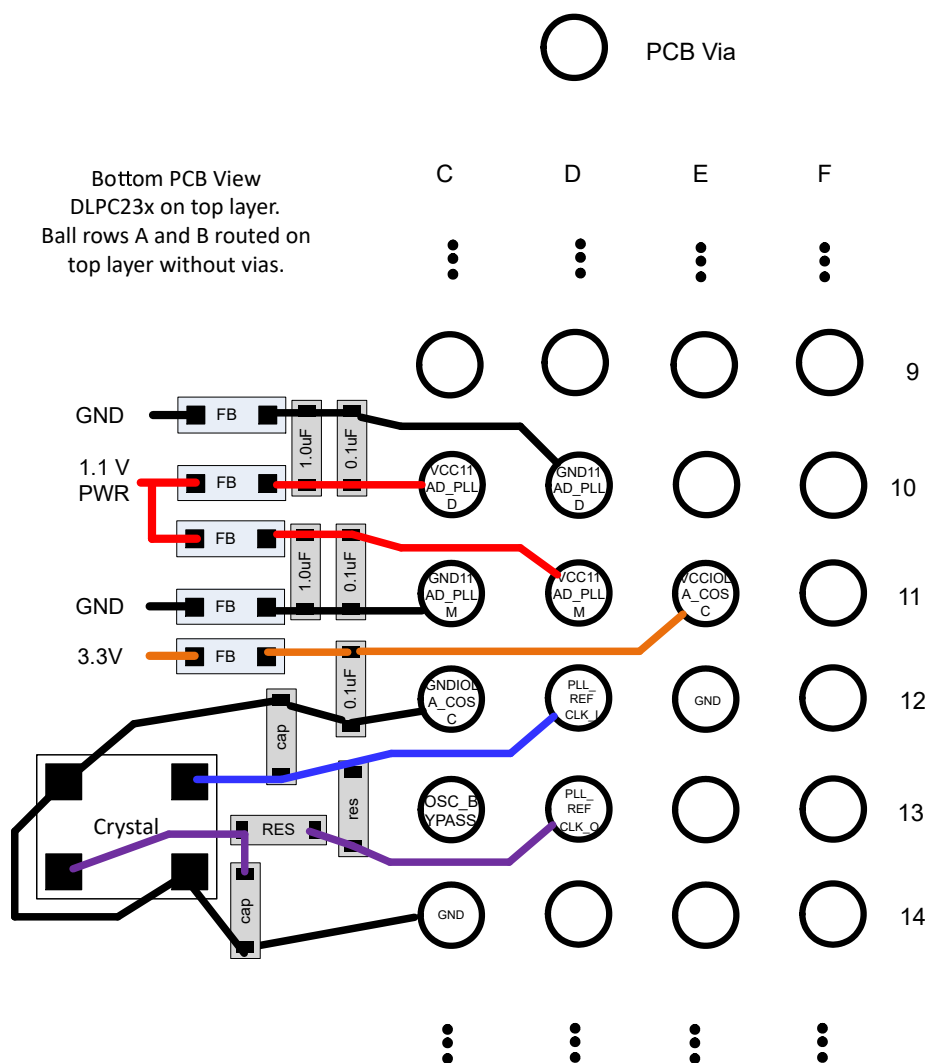
図 8-12. DLPC231-Q1 PLL Filter and Crystal Layout
