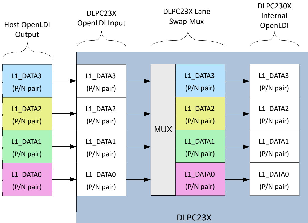
図 7-3. Example of Typical OpenLDI Port Lane Mapping
